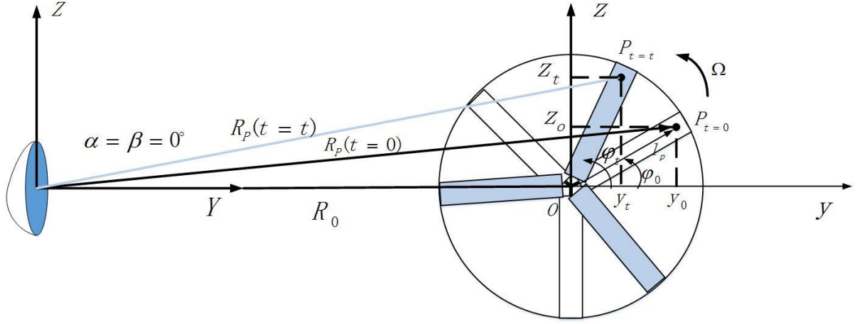
Figure 5.2 Geometric of radar and the rotation rotor blades
