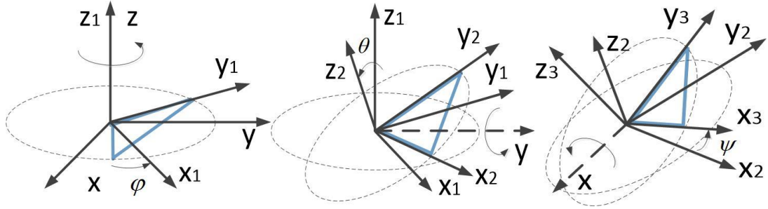
Figure 4.2 Euler angles of three consecutive rotation
