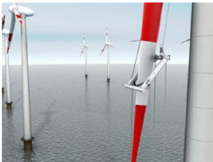
Figure 1.4 Robot RIWEA remote FIG [37]
