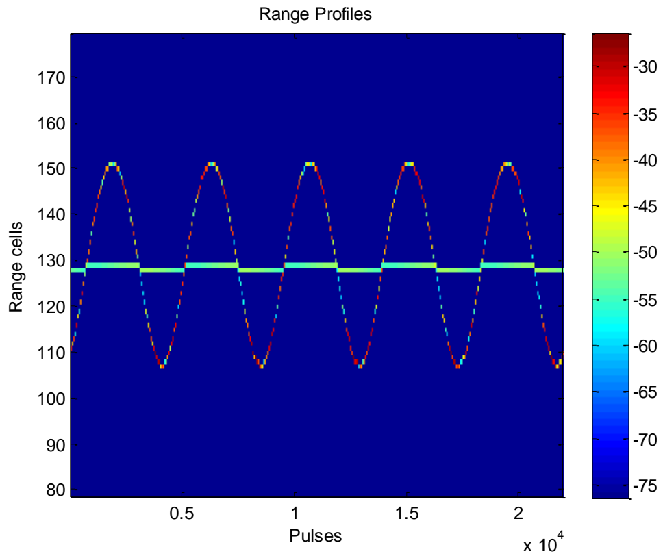
Figure 5.6 One blade tip scattering signal in time domain
