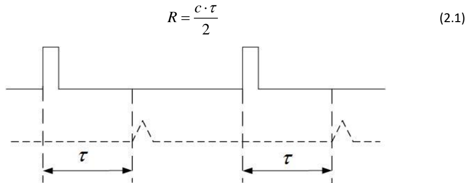
Figure 2.2 Transmitted pulse and target echo schematic
