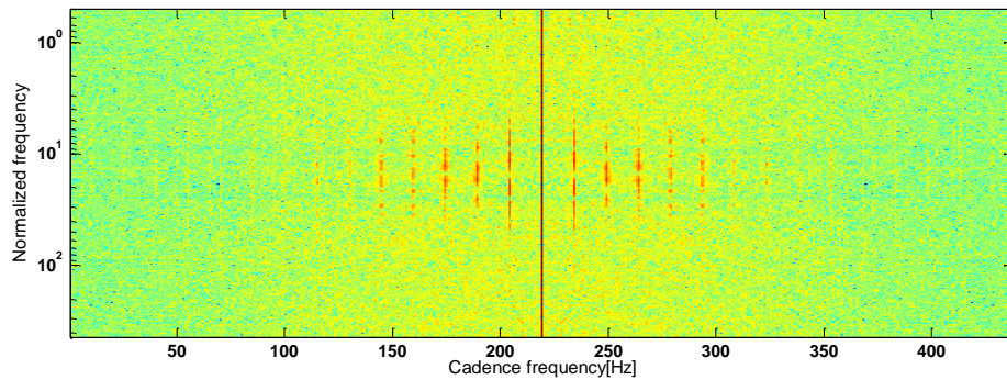
Figure 6.2 CVD from returns relative to rotation blade
