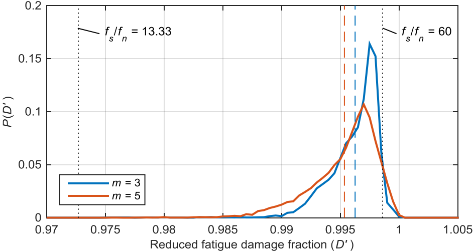
Figure 4-14. Distribution of the reduced fatigue damage resulting from digital sampling of the measured data, calculated using Equation (3-40). The mean values from each distribution are shown with a dashed line of the same colour. The reduced fatigue damage calculated from Equation (3-16) for normalised sample frequencies of 20/1.5 = 13.33 and 20/0.33 = 60 using m = 3 , relating to the second and first modes of the support structures, are shown for comparison.
