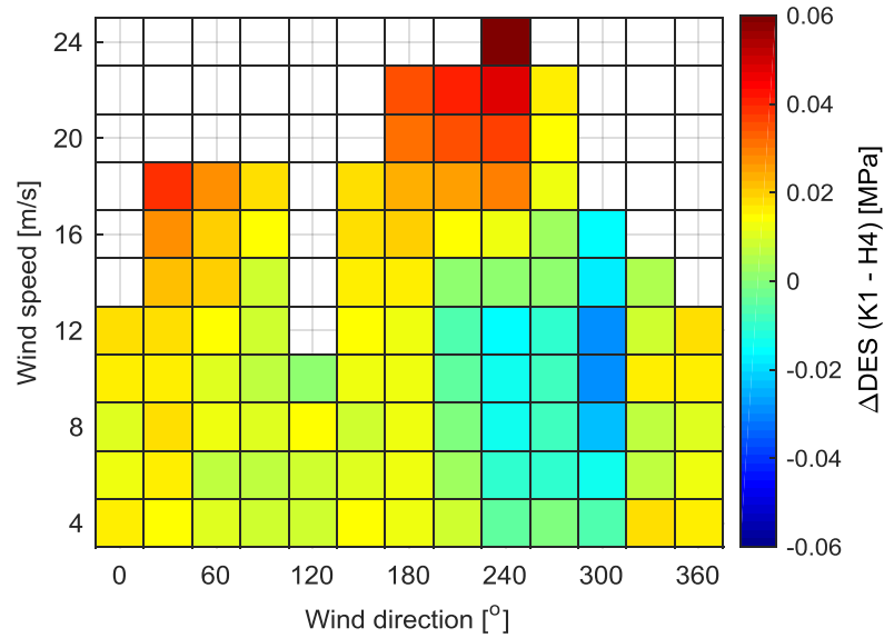
Figure 6-9. Difference between Turbine K1 and H4 mean DES for the full population measurements in MPa, calculated using m = 3 . Power production cases only.
