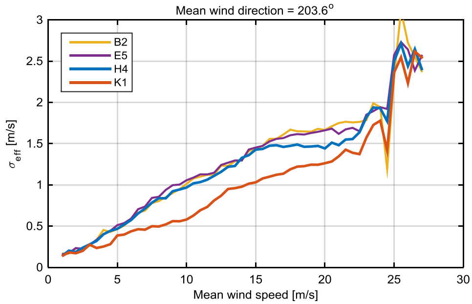
Figure 5-9. Effective standard deviation for turbine spacing of approximately 5.1 rotor diameters (turbines aligned in the mean wind direction of 203.6° +/- 5°).
