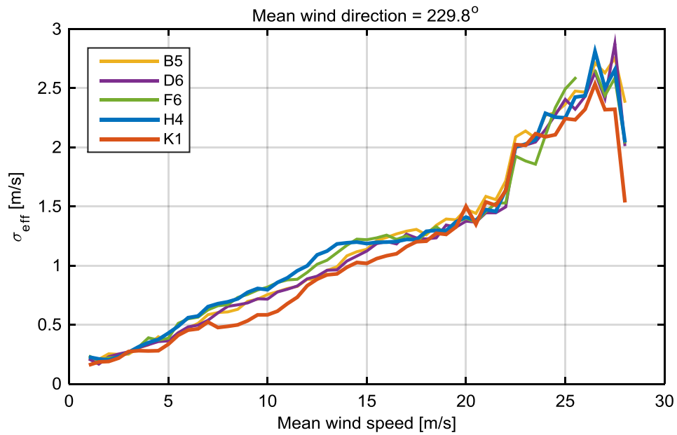
Figure 5-10. Effective standard deviation for turbine spacing of approximately 11.7 rotor diameters (turbines aligned in the mean wind direction of 229.8° +/- 5°).
