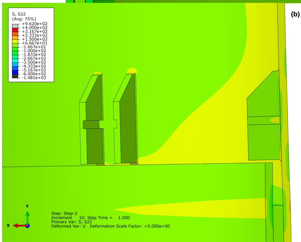
Figure 4-1. FE results showing the stress distribution and scaled displacements for the stopper brackets on the compressive side (a) and tensile side (b) of the structure.
