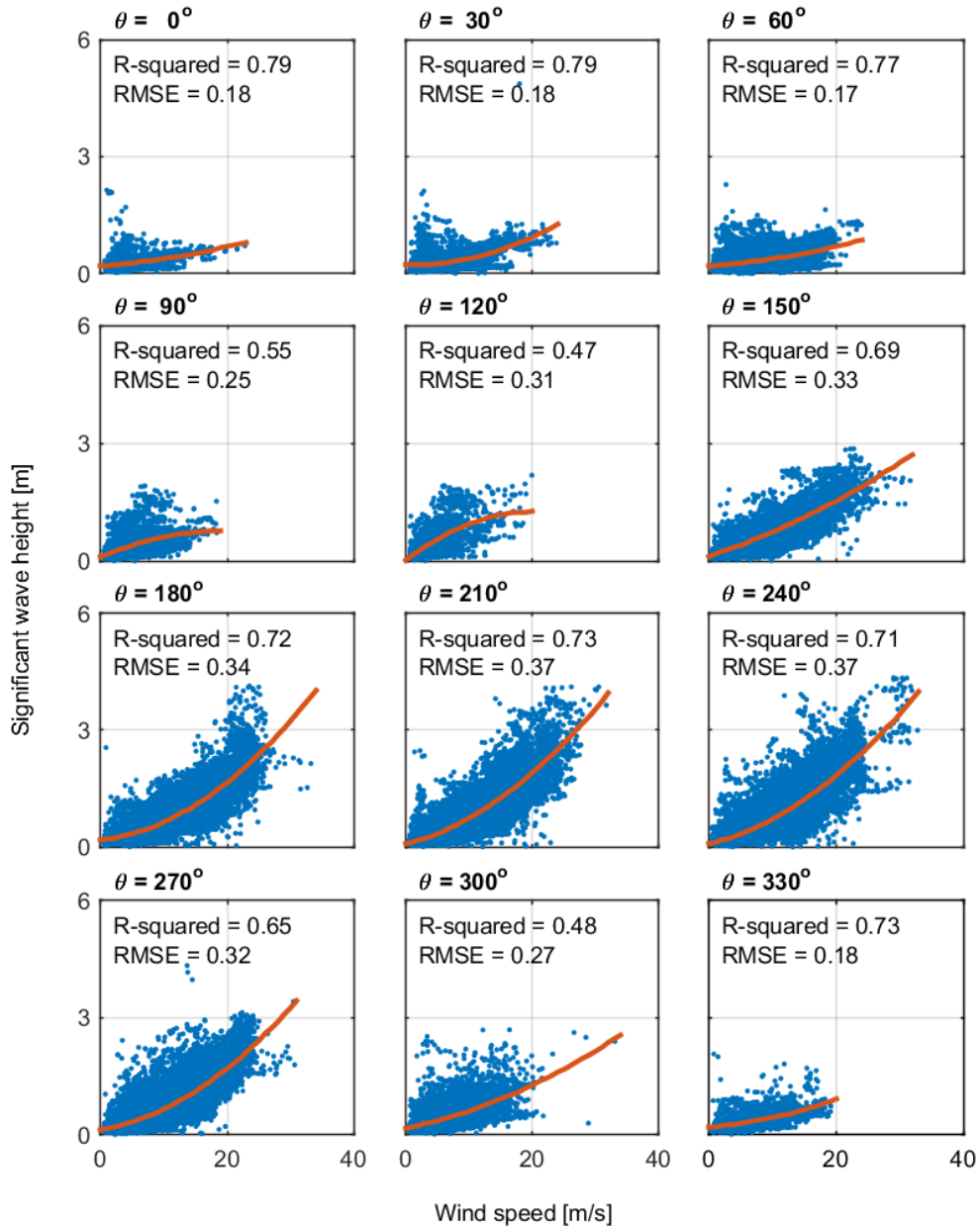
Figure 5-16. Correlations between mean wind speed and significant wave height for each 30^\circ directional sector. The red lines show a second order polynomial function fitted to the data using least squares regression.
