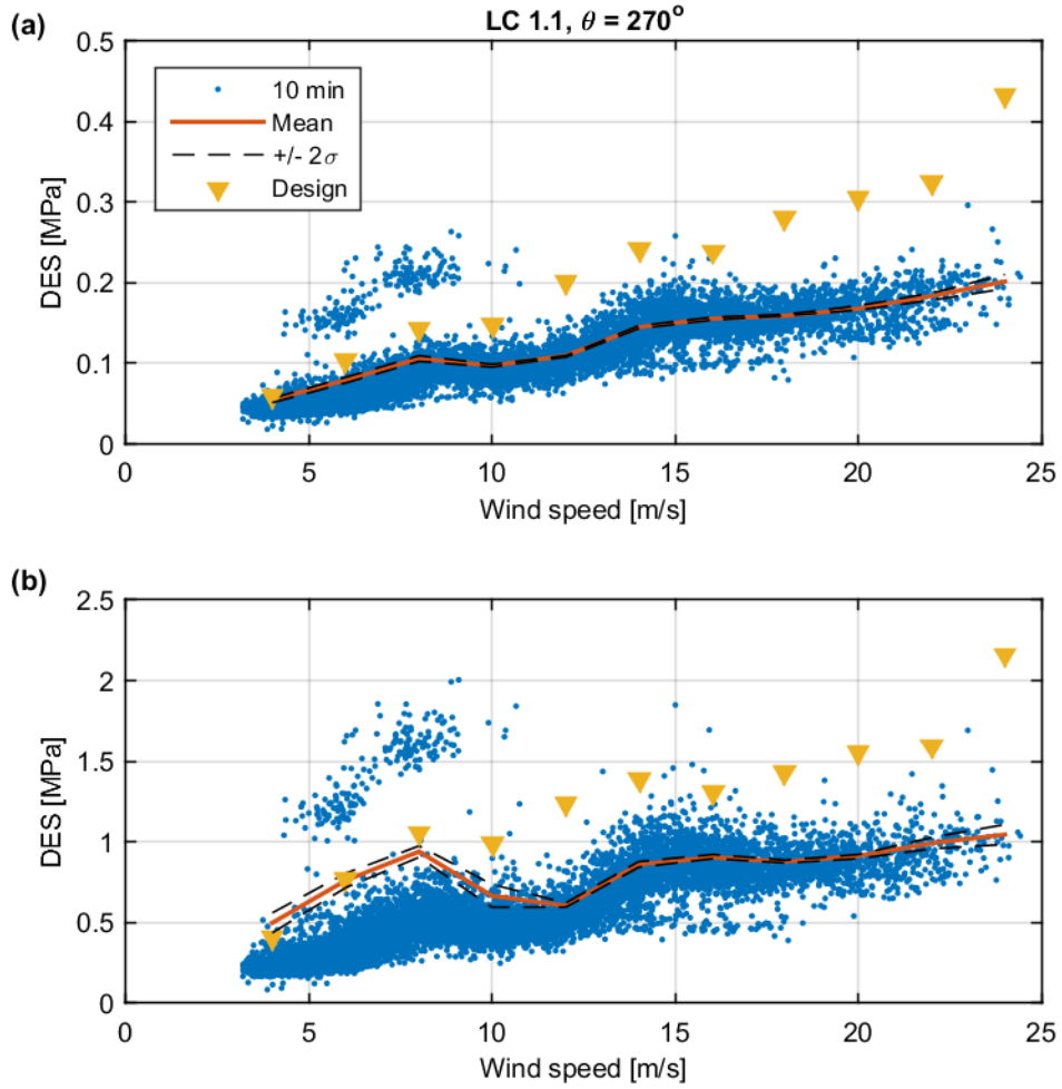
Figure 6-4. DES measured during power production operating conditions, for the 270° wind direction (Turbine K1). Blue dots show single measurements calculated from ten minute periods, red line and black lines show the Bootstrap mean and two standard deviations, respectively, for each 2 m/s wind speed bin, and yellow triangles show the mean DES value calculated from the DLC simulations. (a) DES calculated using m = 3 . (b) DES calculated using m = 5 .
