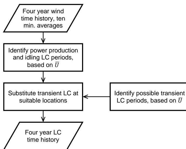
Figure 3-16. Process diagram showing methodology used to construct a representative LC history.
