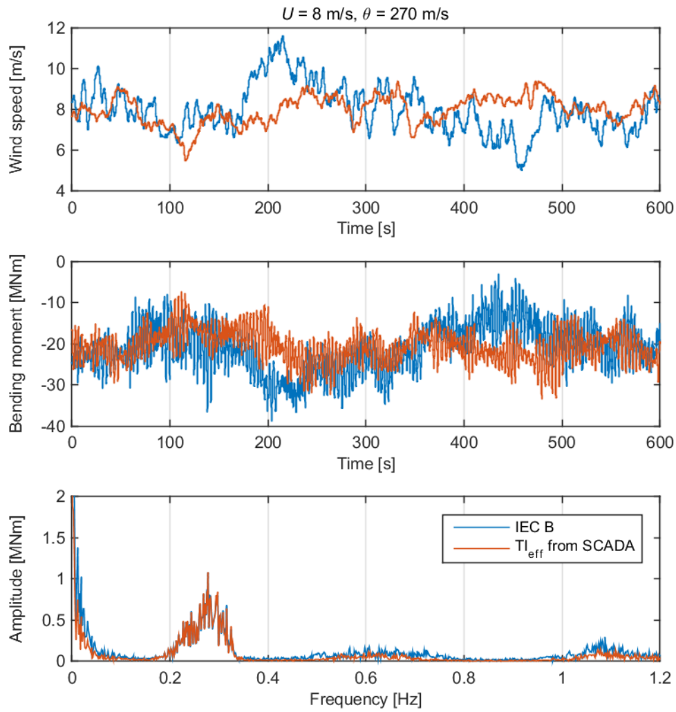
Figure 8-8. M_y bending moment results from the Bladed model under measured Tl_{eff} , compared with IEC B class turbulence, below rated wind speed. (a) Wind time series at hub height. (b) Bending moment time series at -10.6 mCD. (c) Amplitude spectrum calculated from FFT of the ten minute time series (average value from two simulations).
