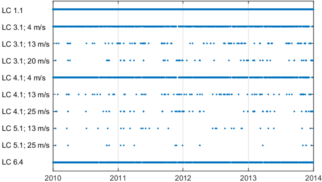
Figure 7-4. Four year representative Load Case sequence identified from the ten minute average wind history. LC 1.1 = normal power production, LC 3.1 = normal start-up, LC 4.1 = normal shut-down, LC 5.1 = emergency stop, LC 6.4 = idling conditions.
