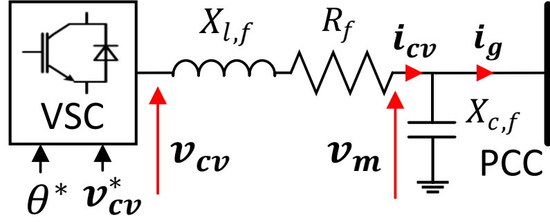
Figure 2.4: Grid-connected voltage-sourced converter. PCC=point of common coupling.
