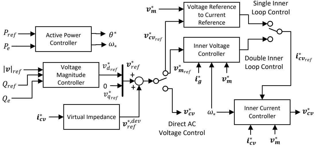
Figure 2.14: Grid-forming cascaded control structure.
