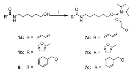
Scheme 3 (i) [( i Pr) 2 N] 2 CN(CH 2 ) 2 OP, 5-benzylthio-1 H -tetrazole, MeCN, rt, 7a 63%, 7b 74%, 7c 64%.
