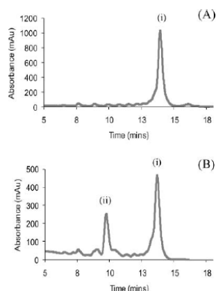
Fig. 2 Ion-exchange HPLC traces of 5'-furyl-modified oligonucleotide and oligonucleotide TAT peptide conjugate at 260 nm. (A) Starting material; (i) 5'-X CGC ATT CAG GAT, (B) Diels-Alder reaction mixture; (i) starting material 5'-X CGC ATT CAG GAT, (ii) TAT 5'-X CGC ATT CAG GAT conjugate.
