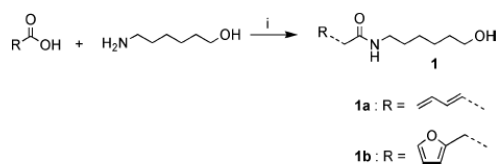
Scheme 1 (i) CDI, rt, MeCN, 1a 70%, 1b 30%.
