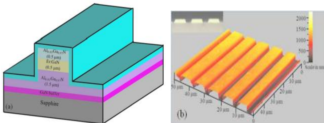
Fig. 7.5: (a) Schematic diagram of an Er-doped GaN Waveguide Amplifier (Here GaN:Er is used as optical gain medium with \text{Al}_{0.03}\text{Ga}_{0.97}\text{N} as top and bottom cladding layers; (b) Atomic Force Microscopy Image of the devices. Reproduced with permission from Ref. [121]
