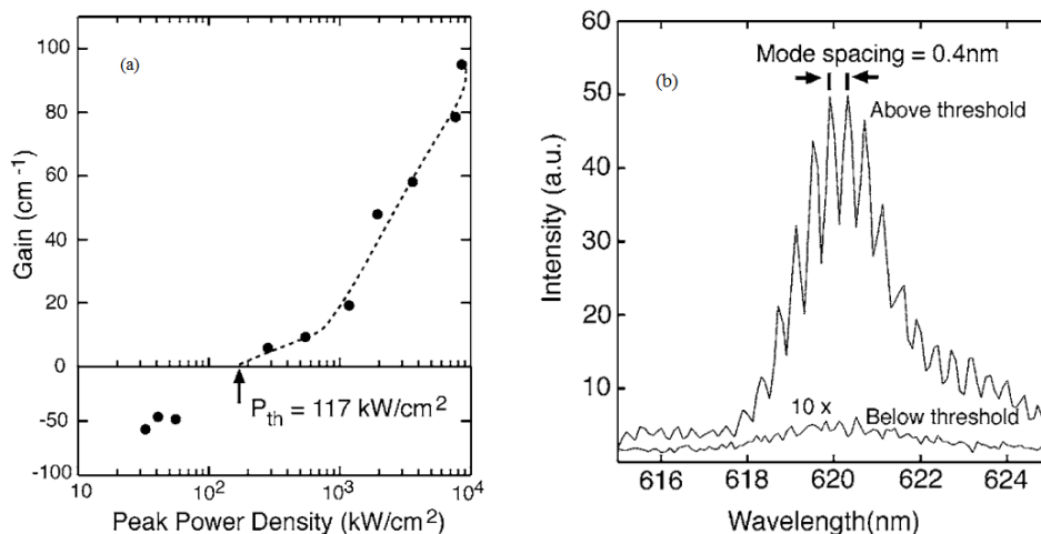
Fig. 8.8: (a) Gain and loss as a function of peak pump power density for GaN:Eu on Si laser structure, (b) Spectrum of edge emission from 350 \mu\text{m} long cavity [147]
