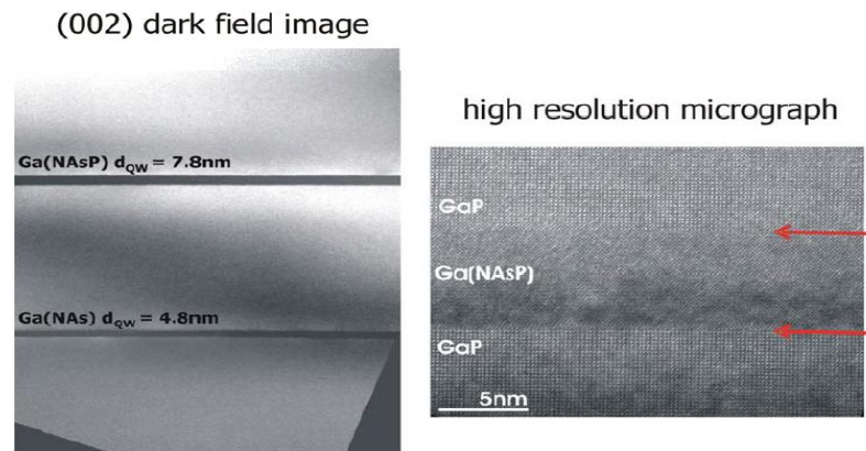
Fig. 8.5: Transmission electron microscopy (TEM) images of Ga(NAsP) quantum wells grown on GaP substrate. Reproduced with permission from Ref. [134]
