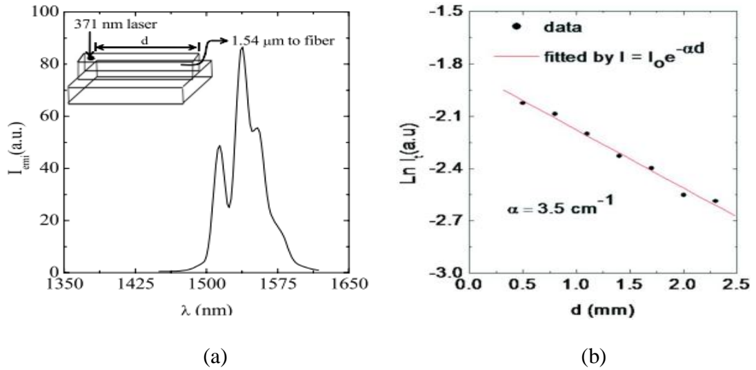
Fig. 7.6: (a) Photoluminescence spectra of Er-doped GaN waveguide amplifier, (b) Plot of 1.54 \mu\text{m} peak intensity vs laser excitation spot distance, 'd'. Reproduced with permission from Ref. [121]
