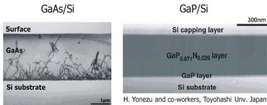
Fig. 8.3: Transmission Electron Microscopy (TEM) images of lattice mismatch due to dislocations formed in the GaAs layer grown on Si (Left), Contrarily GaP/GaNP layers can be formed on Si without any threading dislocations. Reproduced with permission from Ref. [141]
