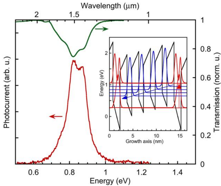
Fig. 7.4: Photocurrent spectrum of 700 \times 700 \mu\text{m}^2 QCDs and transmission spectrum of the sample in multi-pass waveguide configuration with 450 polished facets at room temperature. Conduction band diagram and squared envelope functions of one QCD period. Reproduced with permission from Ref. [117].
