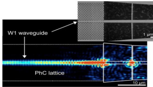
Fig. 5.10: Light propagation through a GaN photonic crystal waveguide. Reproduced with permission from Ref. [69]
