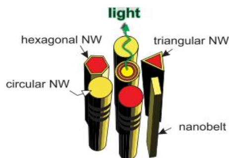
Fig. 5.11: Different structures of nanowires. Reproduced with permission from Ref. [71]
