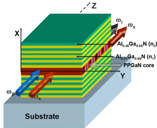
Fig. 5.9: Schematic diagram of a Bragg Reflection Waveguide. Reproduced with permission from Ref. [58]
