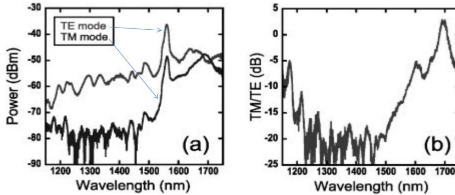
Fig. 6.7: (a) Transmission spectra in an AlN waveguide with GaN/AlN quantum wells, (b) Inter-subband absorption spectrum. Reproduced with permission from Ref. [93]
