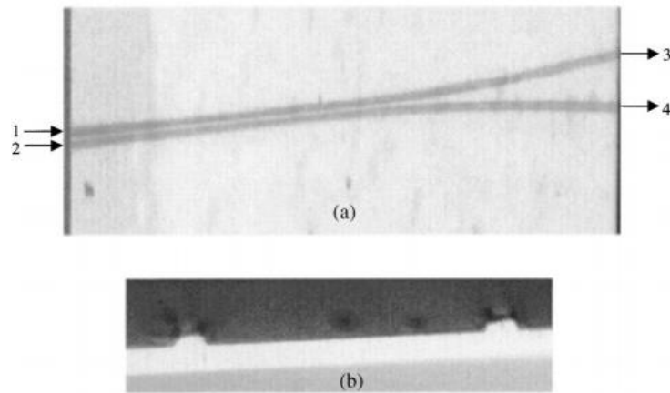
Fig. 5.5: Optical microscope image of GaN/ \text{Al}_x\text{Ga}_{1-x}\text{N} hetero-structure optical waveguide Coupler: (a) Top View (b) Cross-section at the output. Reproduced with permission from Ref. [49]
