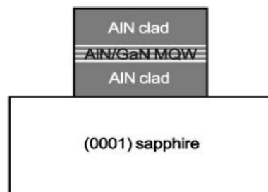
Fig. 6.4: An AlN waveguide structure. Reproduced with permission from Ref. [93]
