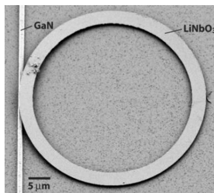
Fig. 8.16: SEM picture of a GaN microring positioned vertically on GaN waveguide. Reproduced with permission from Ref. [165]
