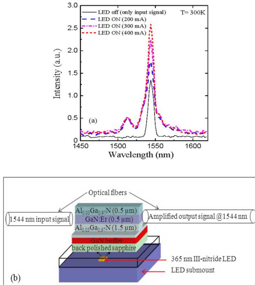
Fig. 7.7: (a) Spectra of the transmitted 1.54 \mu\text{m} signal emerged from the Er-doped GaN waveguide, (b) Schematic of the optical amplification property measurement setup. Reproduced with permission from Ref. [121]
