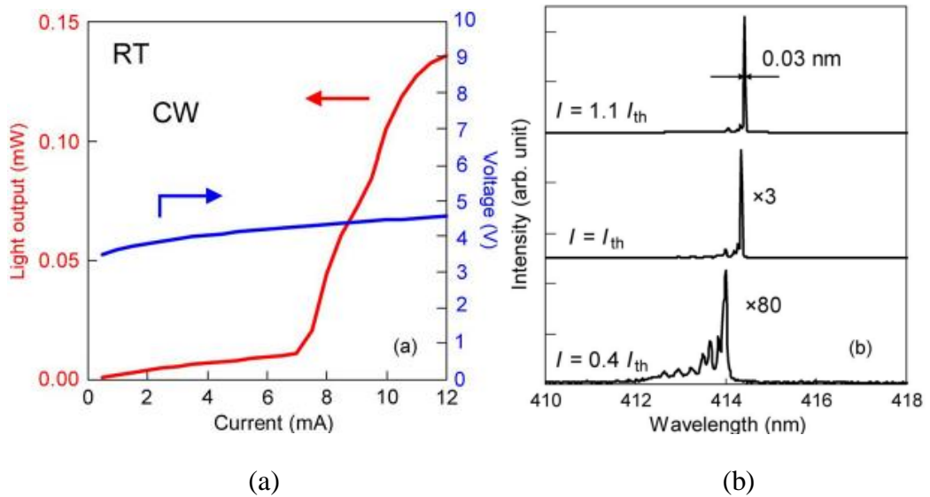
Fig. 7.9: (a) Current vs light output and voltage characteristics of GaN-based VCSEL (b) Spectral emission at different current injections. Reproduced with permission from Ref. [127]
