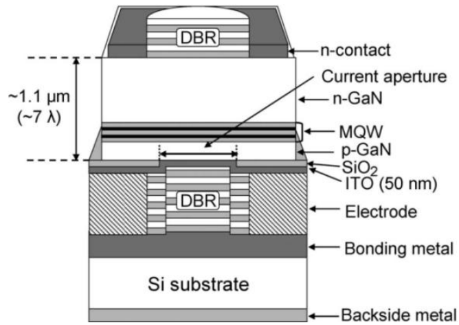
Fig. 7.8: Schematic cross-sectional diagram of a GaN-based VCSEL with vertical current injection feature. Reproduced with permission from Ref. [127]
