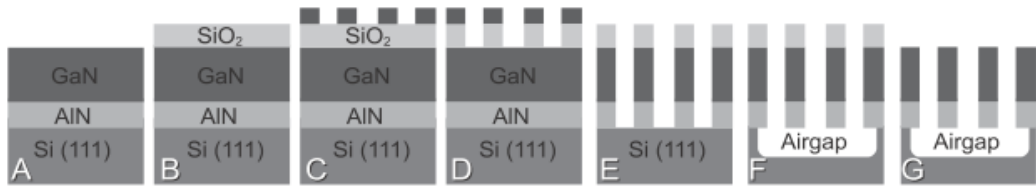
Fig. 4.2: Fabrication process of a GaN based photonic crystal waveguide. Reproduced with permission from Ref. [44]
