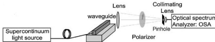
Fig. 6.5: Schematic diagram of measurement setup. Reproduced with permission from Ref. [93]
