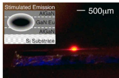
Fig. 8.7: Stimulated emission from the edge of the GaN:Eu on Si lasing structure. The inset shows the cross-section of the structure. Reproduced with permission from Ref. [147]
