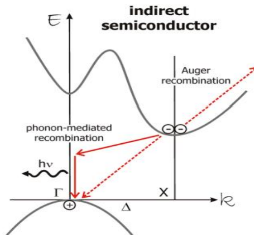
Fig. 8.1: Indirect band-gap structure of Si. Reproduced with permission from Ref. [134]
