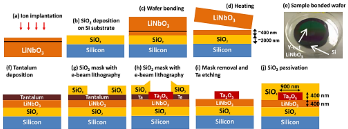
Fig. 8.12: (a) to (d) Processing steps for the fabrication of \text{LiNbO}_3 -on-Si wafers; (e) A successful bonding of a 3" \text{LiNbO}_3 wafer bonded to a 4" Si wafer; (f) to (j) SORAM process of submicron \text{LiNbO}_3 ridge waveguide on Si. Reproduced with permission from Ref. [160]
