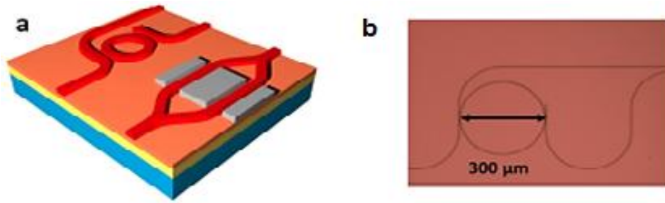
Fig. 8.13: (a) A schematic of microring resonator and Mach-Zehnder modulator, (b) A top view of a high magnification optical microscope image of a fabricated ring-resonator with input and output bent bus waveguides. Reproduced with permission from Ref. [160]
