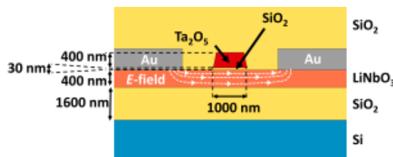
Fig. 8.11: Cross-section of a \text{LiNbO}_3 on Si waveguide. Reproduced with permission from Ref. [160]
