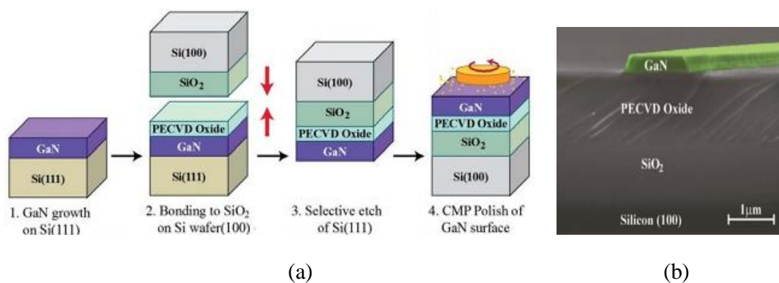
Fig. 4.1: (a) GaN photonic circuits are built on ‘GaN on \text{SiO}_2 on Si’ (GaNOI) substrates. (b) A cross sectional scanning electron micrograph showing a fabricated GaN waveguide. Reproduced with permission from Ref. [42]
