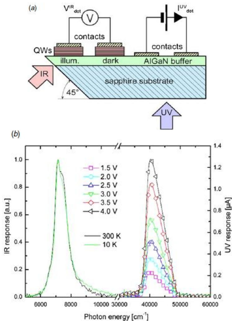
Fig. 7.2: (a) Schematic cross section through the sample showing the relative positions of the UV and the IR detector. The QWs are used as the detection layer for the IR, while the AlGaN buffer is the detection layer for the UV radiation. (b) Spectral responsivity curves measured for the UV (1.5 to 4.0 V in steps of 0.5 V). Reproduced with permission from Ref. [114]
