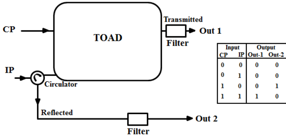
Fig. 3.3: TOAD-based all-optical interferometric switch
