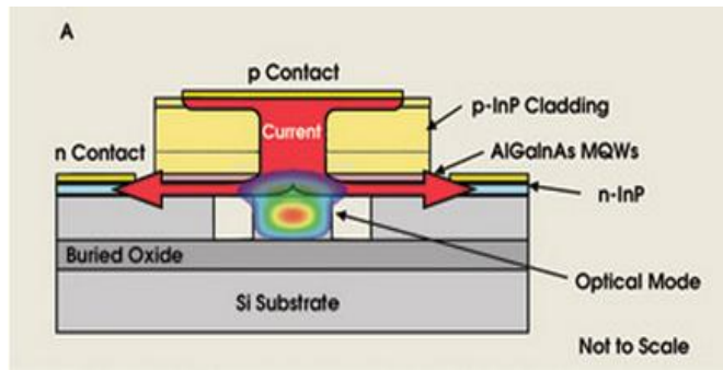
Fig. 8.2: The Schematic diagram of a hybrid laser
