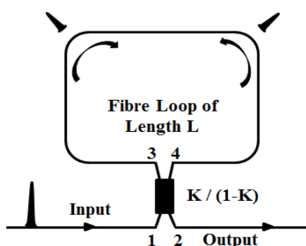
Fig. 3.1: Structure of a NOLM
