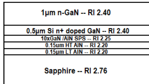
Fig. 6.10: Schematic diagram of the waveguide structure
