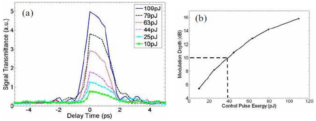
Fig. 6.2: (a) Signal transmittance through a GaN QW waveguide versus signal-control delay time for different control energies (b) Modulation depth versus control pulse energy (calculated from the traces of (a)). Reproduced with permission from Ref. [80]
