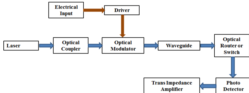
Fig. 8.9: Different components in an integrated photonic chip (brown lines indicate electrical signals and blue lines indicate optical signals)
