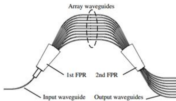
Fig. 5.8: Schematic diagram of an AWG de-multiplexer
