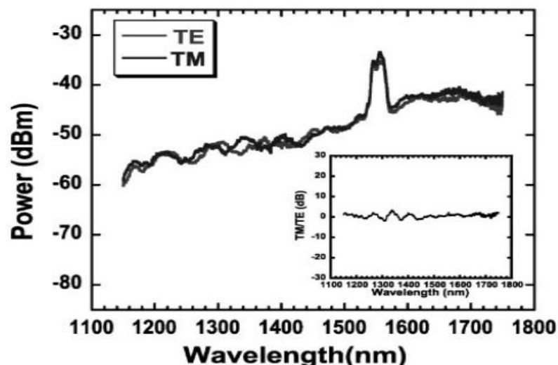
Fig. 6.6: TE and TM polarized transmission spectra in an AlN waveguide without GaN/AlN quantum wells. Reproduced with permission from Ref. [93]
