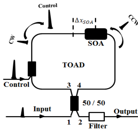
Fig. 3.2: Schematic diagram of TOAD
