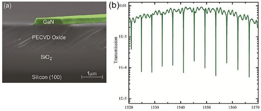
Fig. 8.10: (a) Scanning Electron Micrograph of a cross section of a GaOI waveguide (b) Optical transmission of a GaN microresonator. Reproduced with permission from Ref. [155]
