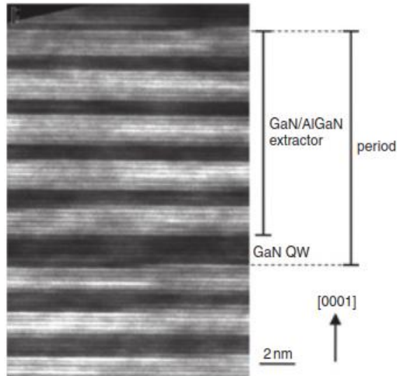
Fig. 7.3: TEM Image of hetero-structure dark, grey and bright regions which correspond to GaN, AlGaN and AlN respectively. Reproduced with permission from Ref. [118]
