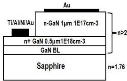
Fig. 6.11: The electro-optic structure on GaN/sapphire
