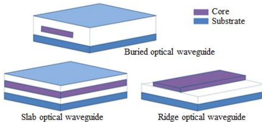
Fig. 5.1: Examples of waveguides
