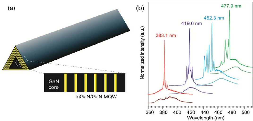
Fig. 6.13: (a) Diagram of a GaN/InGaN nanowire showing the cross-sectional magnified view of NW facet with MQW structure (b) Normalized PL spectra collected from four representative 26 MQM nanowire structures. Reproduced with permission from Ref. [71, 103]
