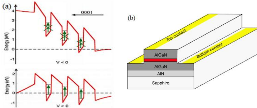
Fig. 6.8: (a) Principle of operation of depletion modulator (b) Ridge waveguide modulator device. Reproduced with permission from Ref. [95]
