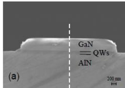
Fig. 6.1: A SEM image of the facet of a GaN/AlN QW waveguide. Reproduced with permission from Ref. [81]
