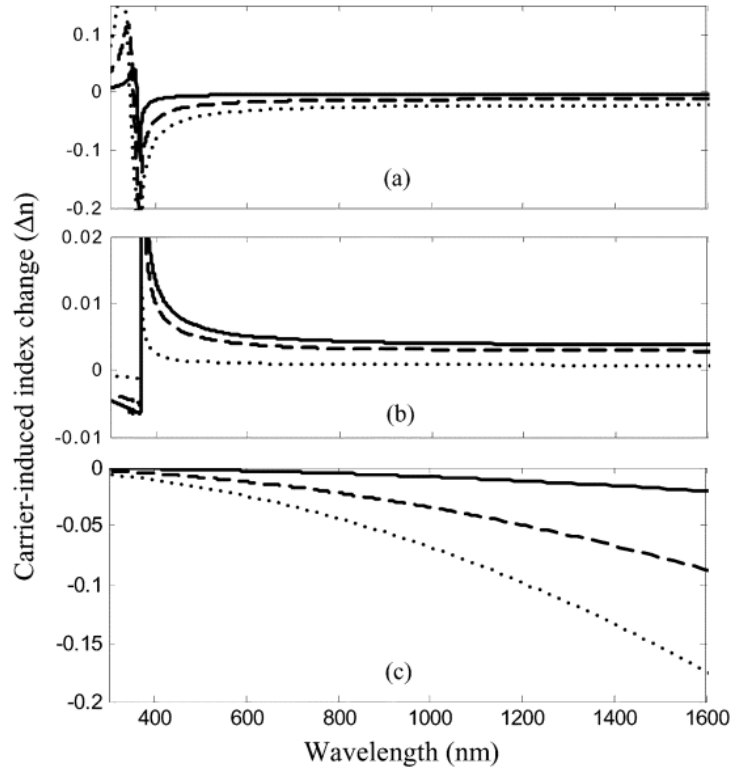
Fig. 5.6: (a) Index change for bandfilling, (b) Band shrinking, (c) Free carrier absorption at N = 7 \times 10^{18} \text{ cm}^{-3} as solid line, N = 3 \times 10^{19} \text{ cm}^{-3} as dashed line and 6 \times 10^{19} \text{ cm}^{-3} as dotted lines. Reproduced with permission from Ref. [51]
