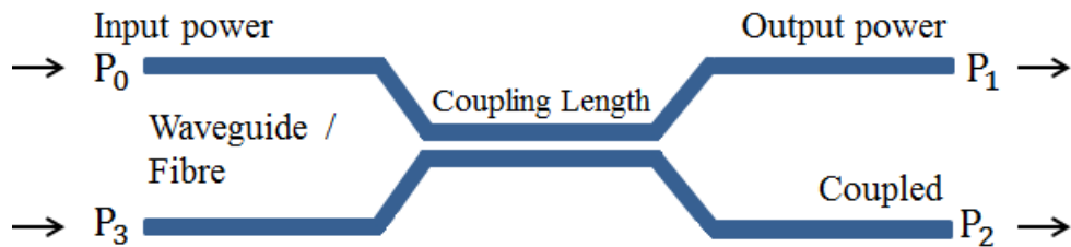
Fig. 5.2: A 2x2 directional coupler
