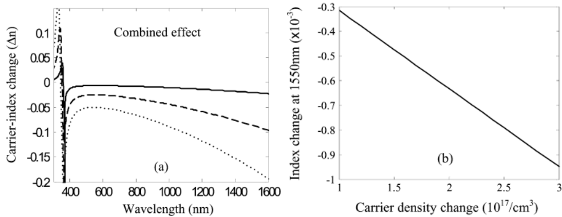
Fig. 5.7: (a) Overall index change vs wavelength at three carrier density levels ( N = 7 \times 10^{18} \text{ cm}^{-3} as solid line, N = 3 \times 10^{19} \text{ cm}^{-3} as dashed line and 6 \times 10^{19} \text{ cm}^{-3} as dotted lines). (b) Overall index change vs carrier density at 1550 nm. Reproduced with permission from Ref. [51]
