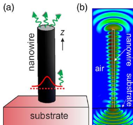
Fig. 6.12: (a) Schematic diagram of a single nanowire Fabry-Perot (FP) cavity, (b) Laser intensity profile. Reproduced with permission from Ref. [71]
