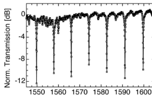
Fig. 8.17: Measured transmission spectrum through the GaN port waveguide of the microring resonator. The resonances are separated by a FSR of 8.1 nm at 1.55 μm wavelength. Reproduced with permission from Ref. [165]
