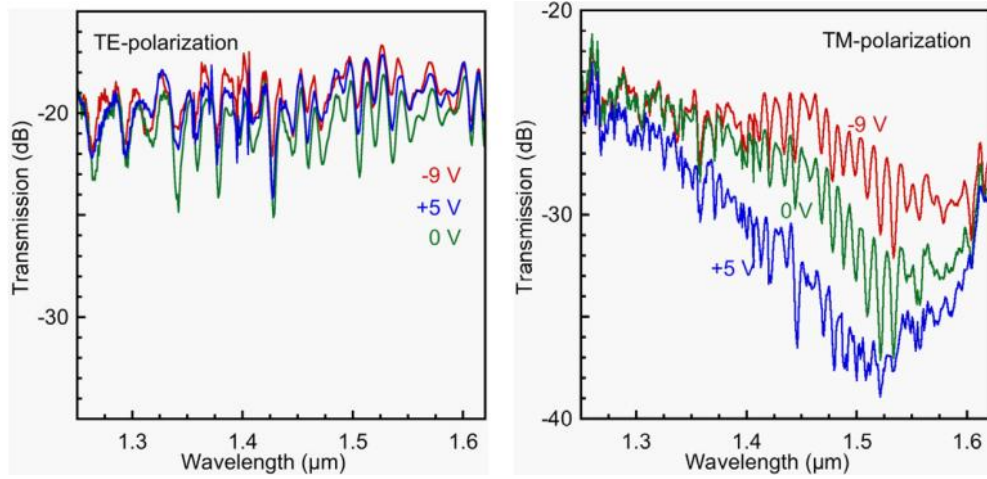
Fig. 6.9: Waveguide transmission spectra of the depletion modulator for TE and TM polarized light. Reproduced with permission from Ref. [95]
