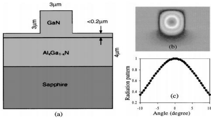
Fig. 5.4: Optical waveguide design using GaN/ \text{Al}_x\text{Ga}_{1-x}\text{N} hetero-structure grown on sapphire substrates: (a) Waveguide Cross-section, (b) Single mode simulation, (c) Radiation pattern vs exit angle. Reproduced with permission from Ref. [49]
