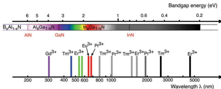
Fig. 8.6: Associated band-gap energies of III-N compound semiconductors and emission wavelengths from selected transitions in rare earth ions. Reproduced with permission from Ref. [145]
