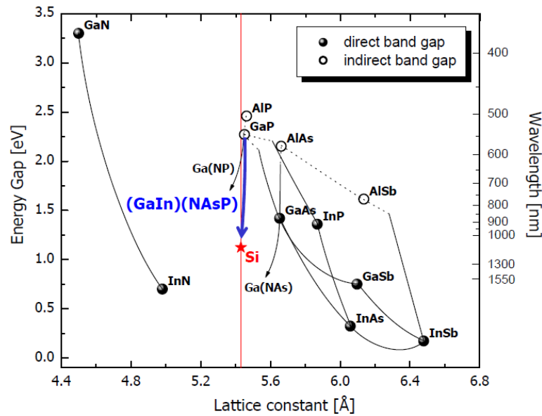
Fig. 8.4: Plot for the energy gap vs lattice constant of common III-V materials compared to Si. Reproduced with permission from Ref. [134]
