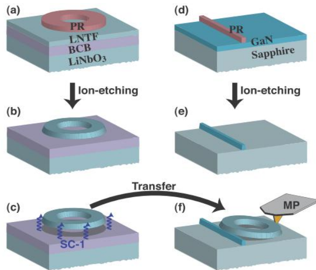
Fig. 8.15: The fabrication process of realizing the hybrid microring resonator. Reproduced with permission from Ref. [163, 165]
