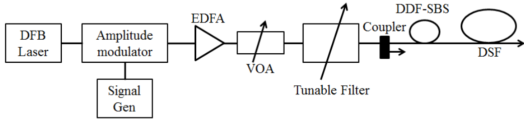
Fig. 3.4: Experimental setup for comb-like spectrum generation
