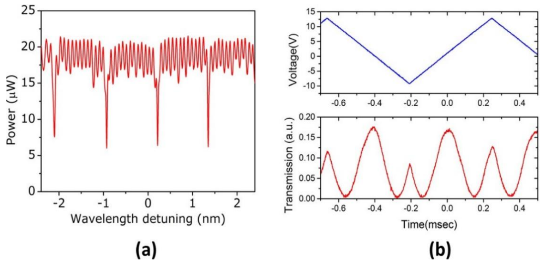
Fig. 8.14: (a) Transmission spectrum of a microresonator (300 \mu\text{m} dia) for TE mode at telecom band. The resonance linewidth is 2.7 GHz; (b) Sawtooth electrical signal applied and the measured modulation response of the Mach-Zehnder modulator. Reproduced with permission from Ref. [160]
