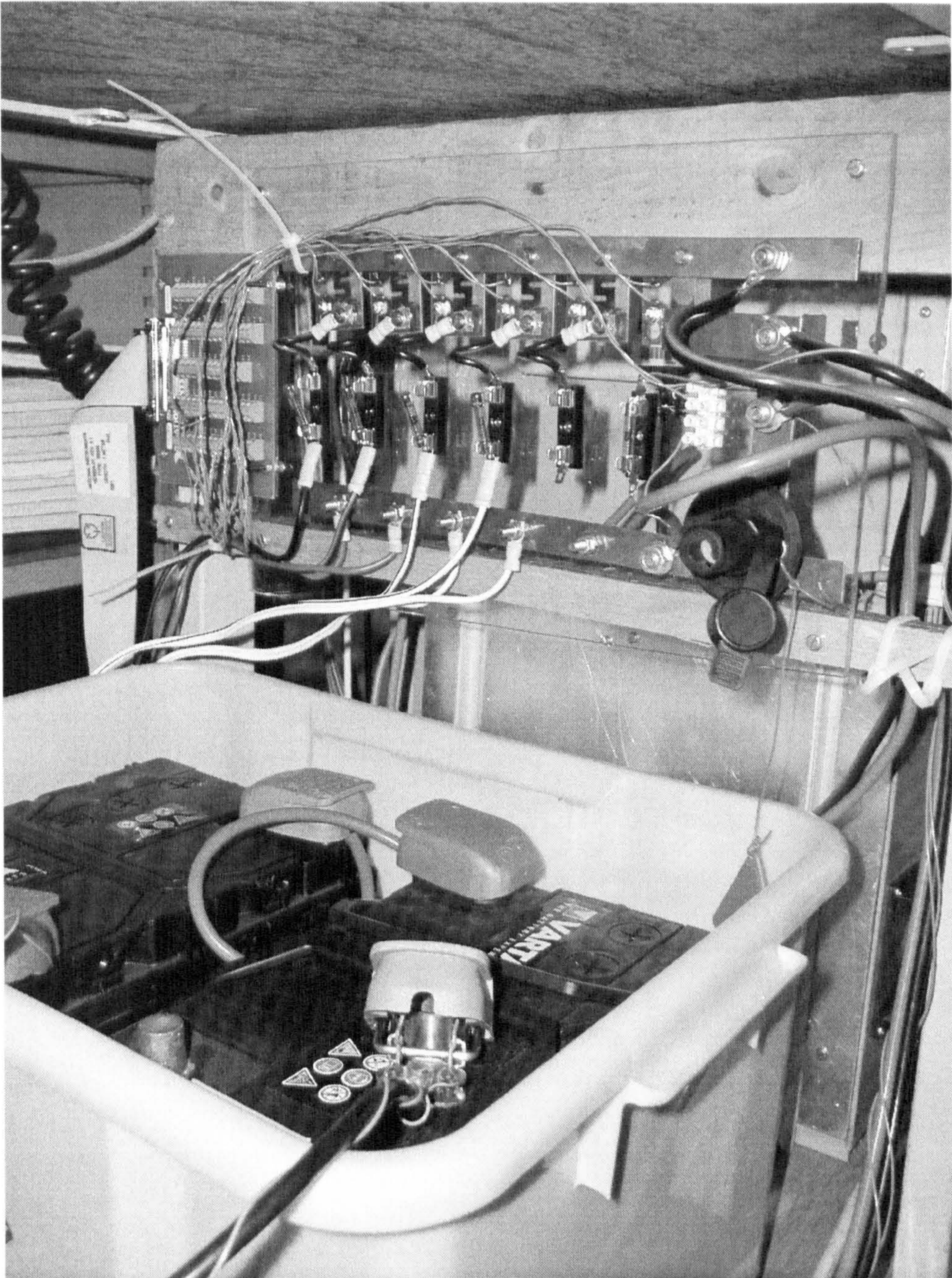
(Fig. 6.5: DC terminal board and battery bank)
