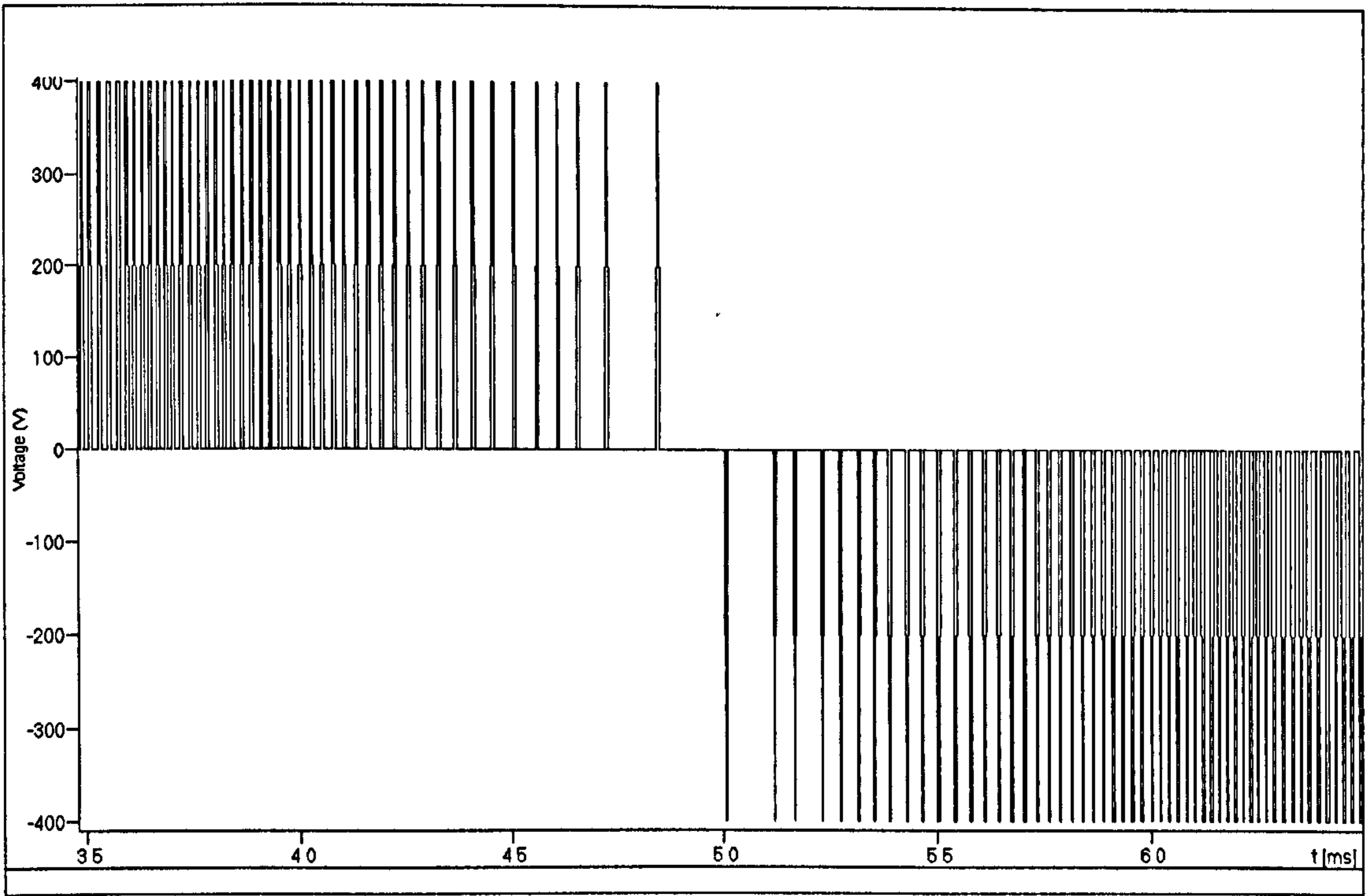
(Fig. A.7: Simulated switching waveform: close-up shown, note time scale)
