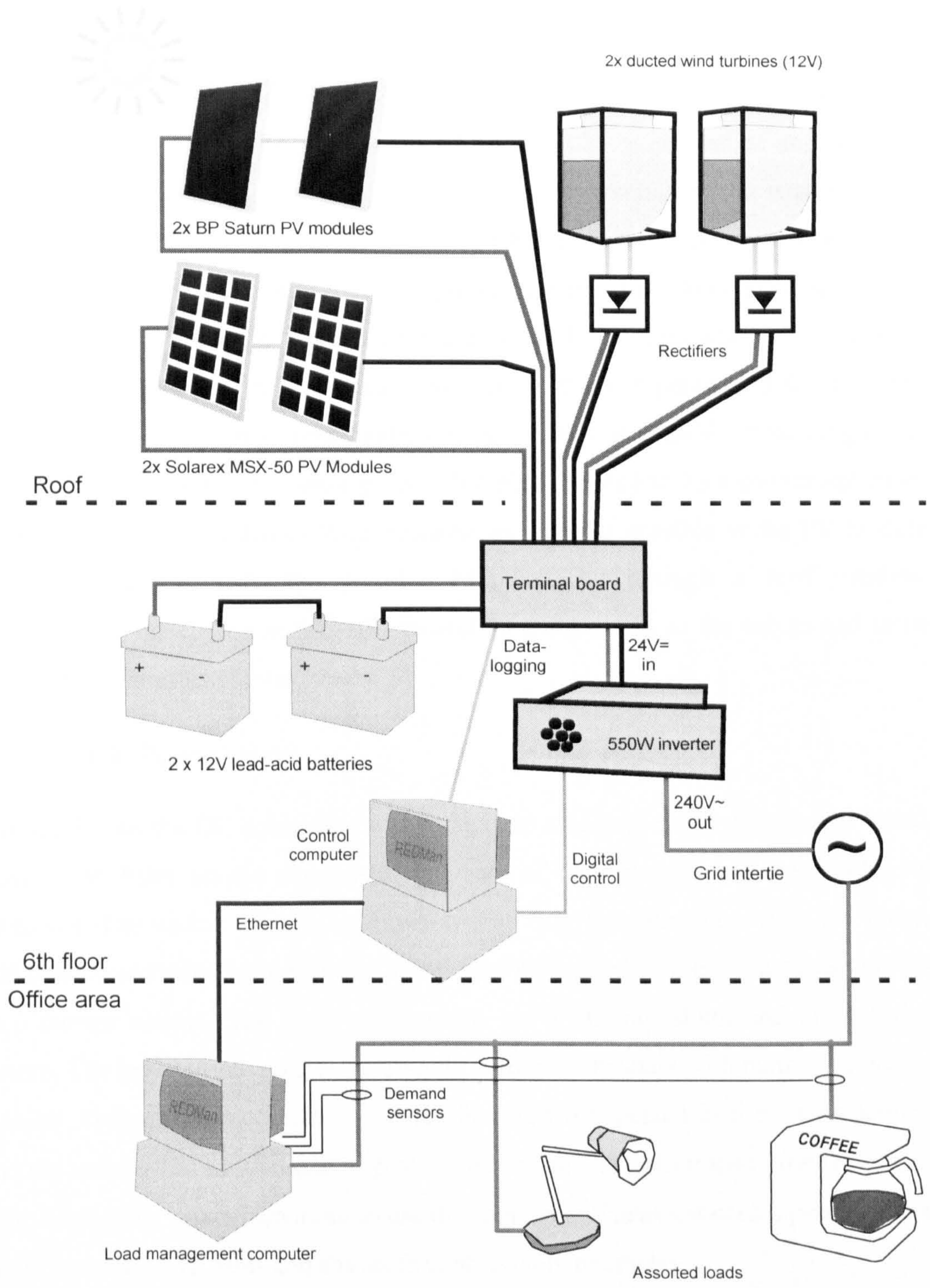
(Fig 6.1: Layout of the test-bed)
