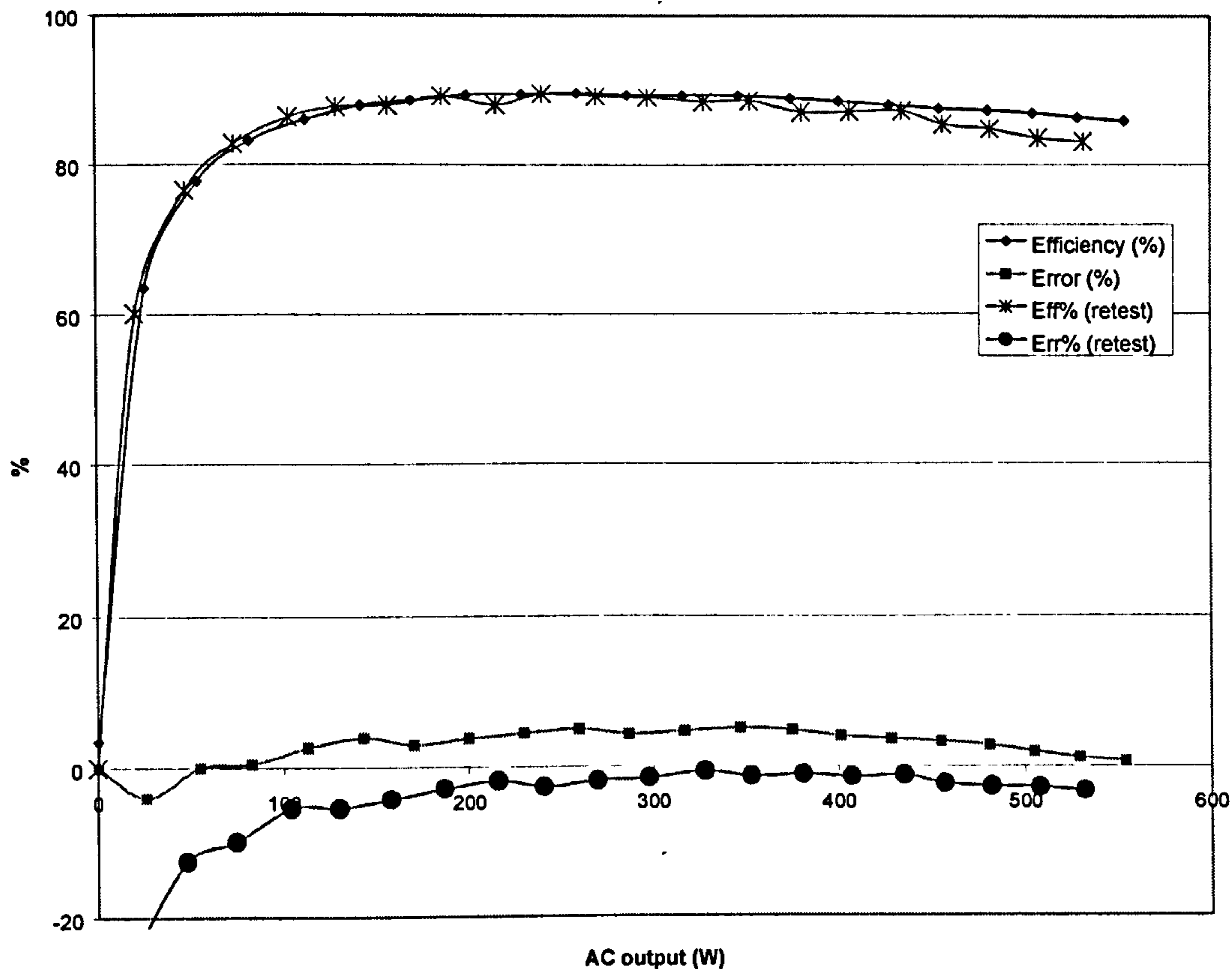
(Fig. 9.1: Efficiency and calibration curves of inverter re-test)
