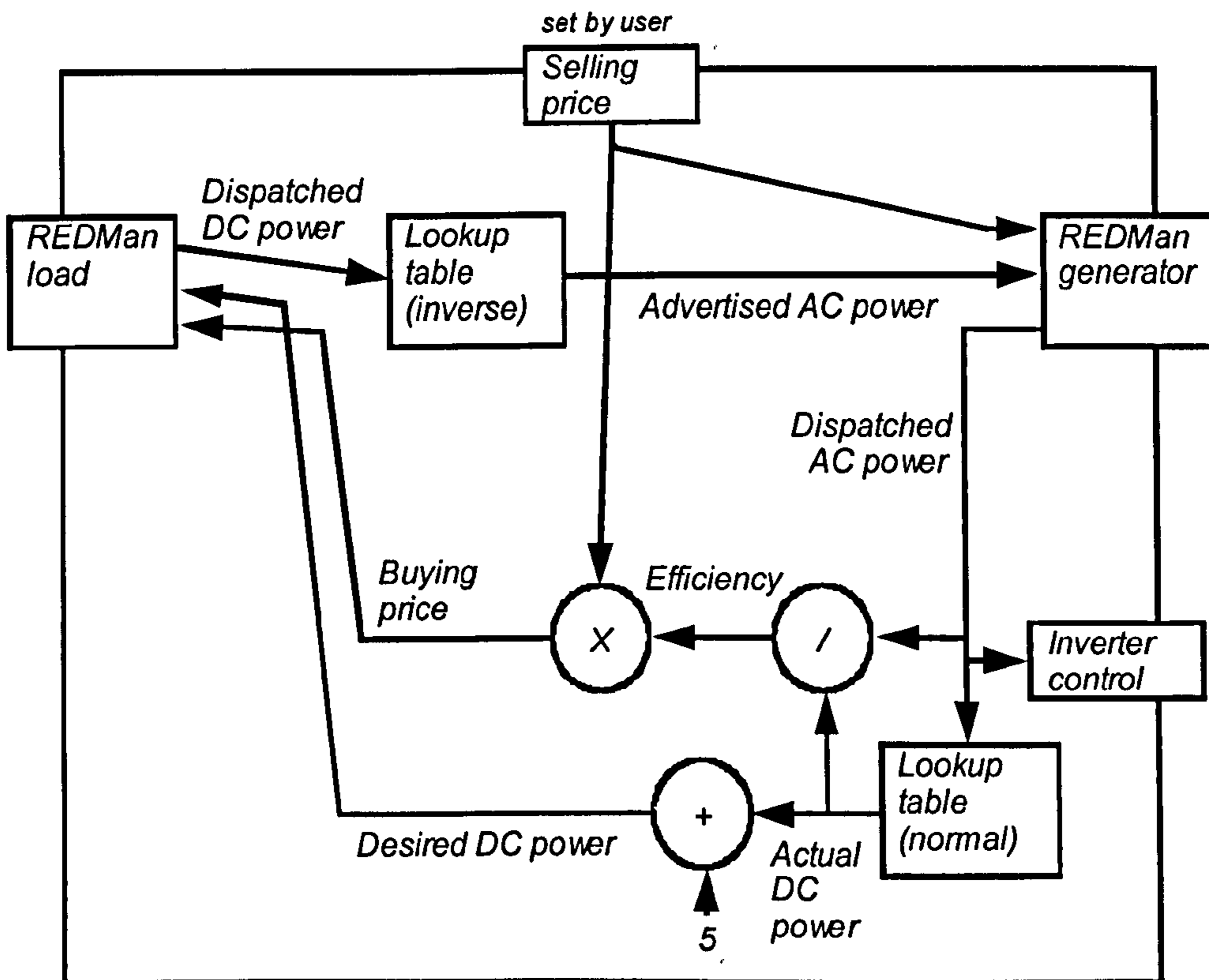
(Fig. 7.5: Inverter management with revised economic dispatching)
