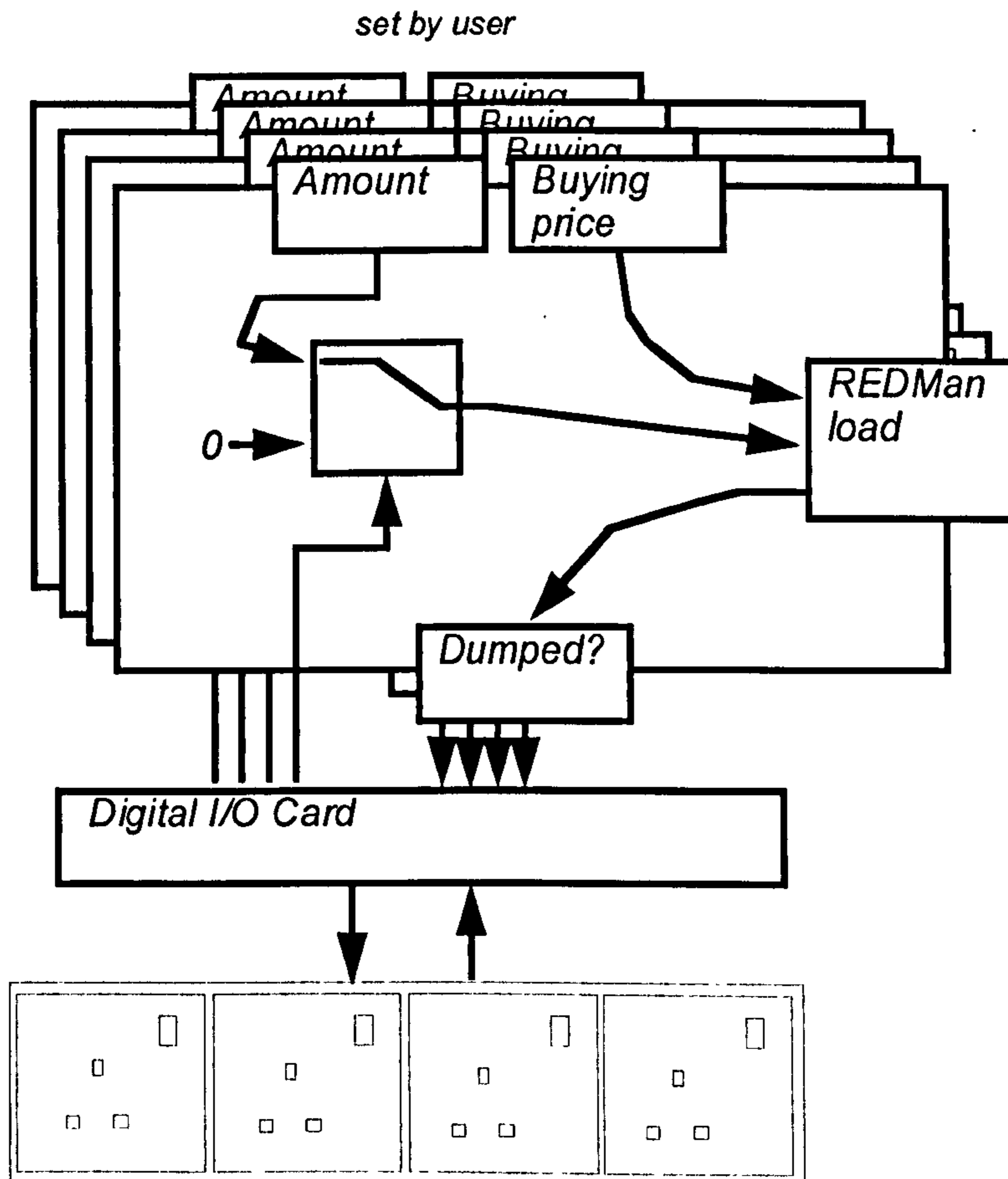
(Fig. 7.9: block diagram of smart socket/agent system)
