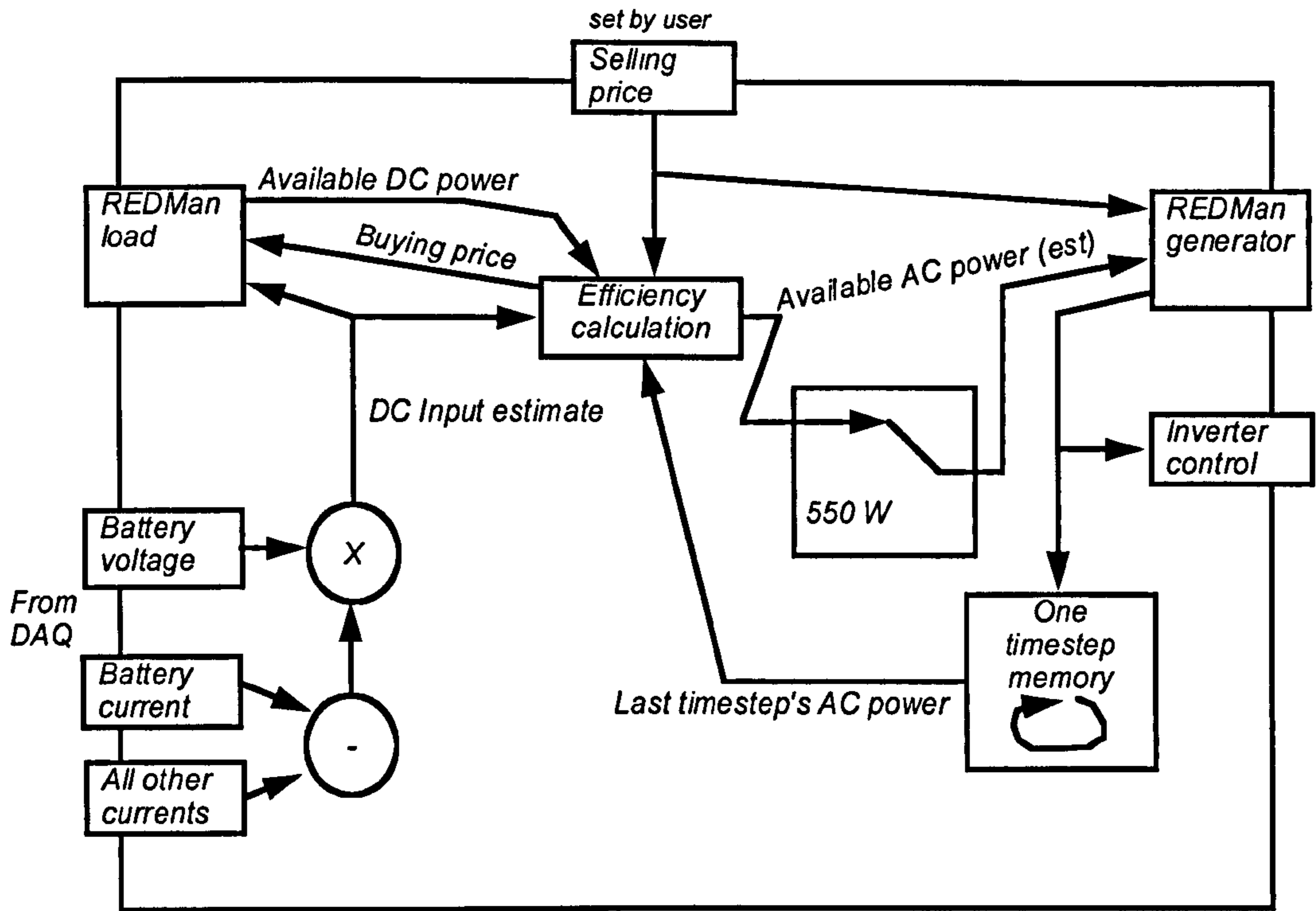
(Fig. 7.4: Original inverter management)
