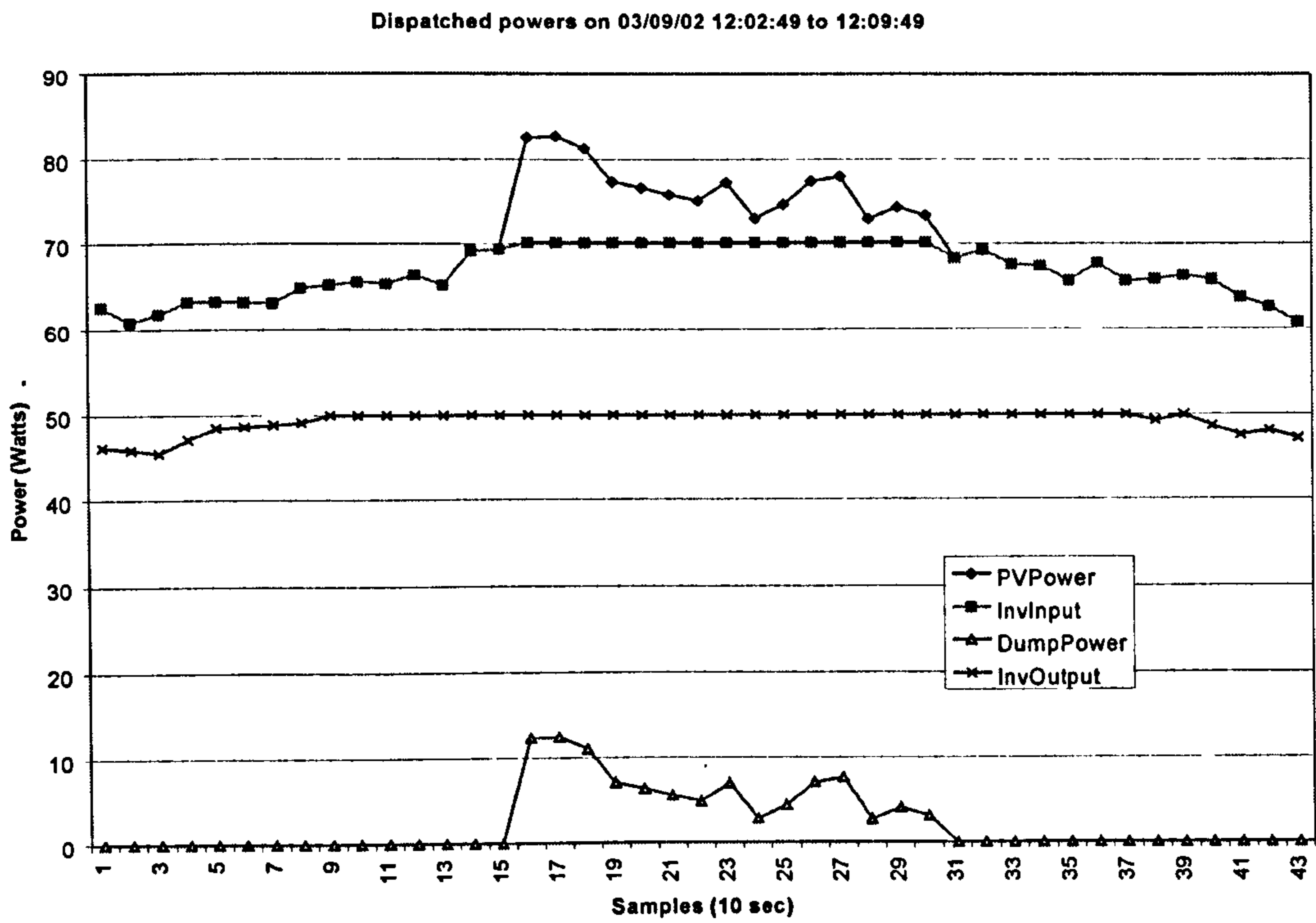
(Fig. 9.2: Time history of dispatched powers)
