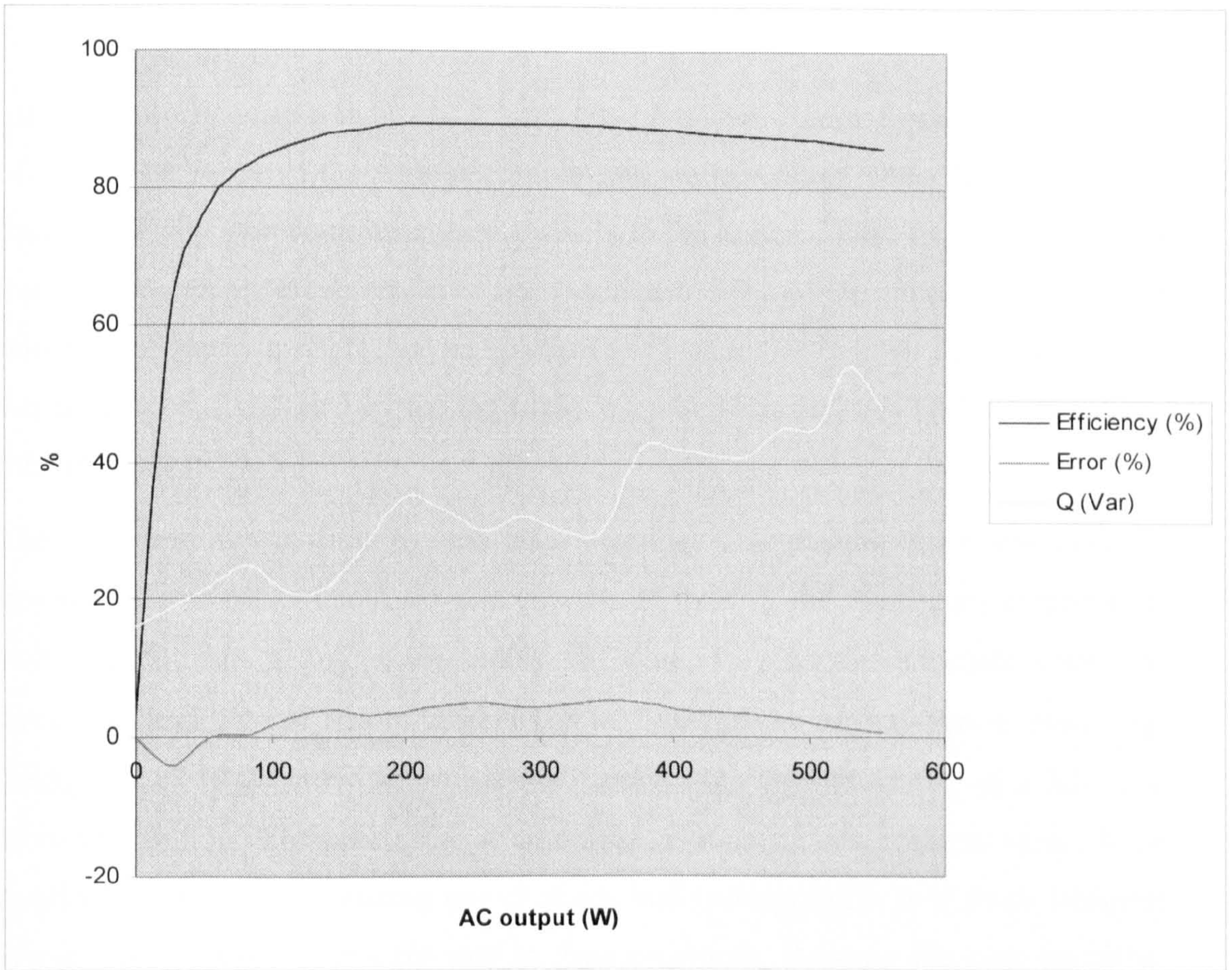
(Fig. A.21: Mark Two efficiency/reactive power/control error)
