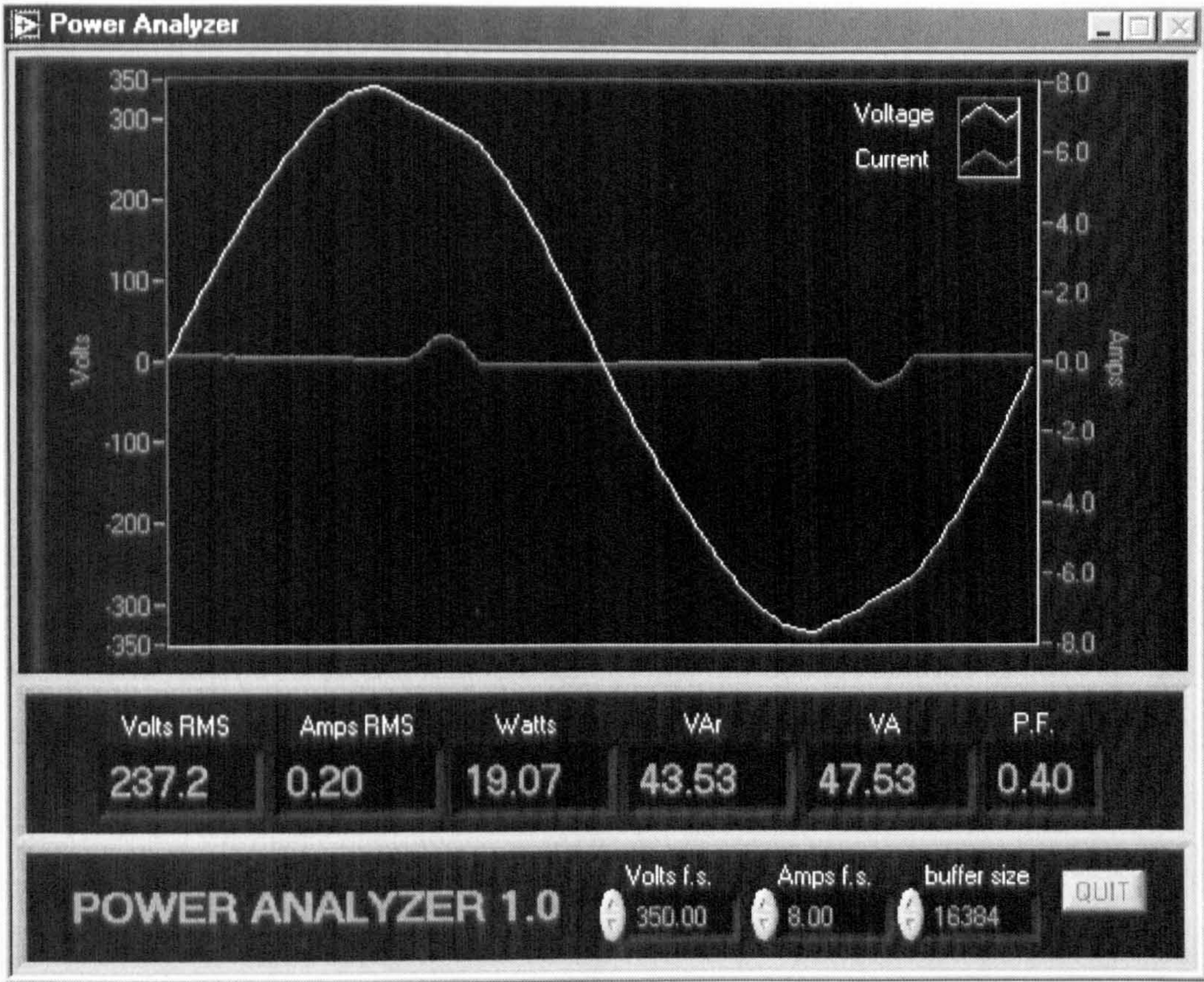
(Fig. D.5: Power analysis of mains power unit of a laptop)
