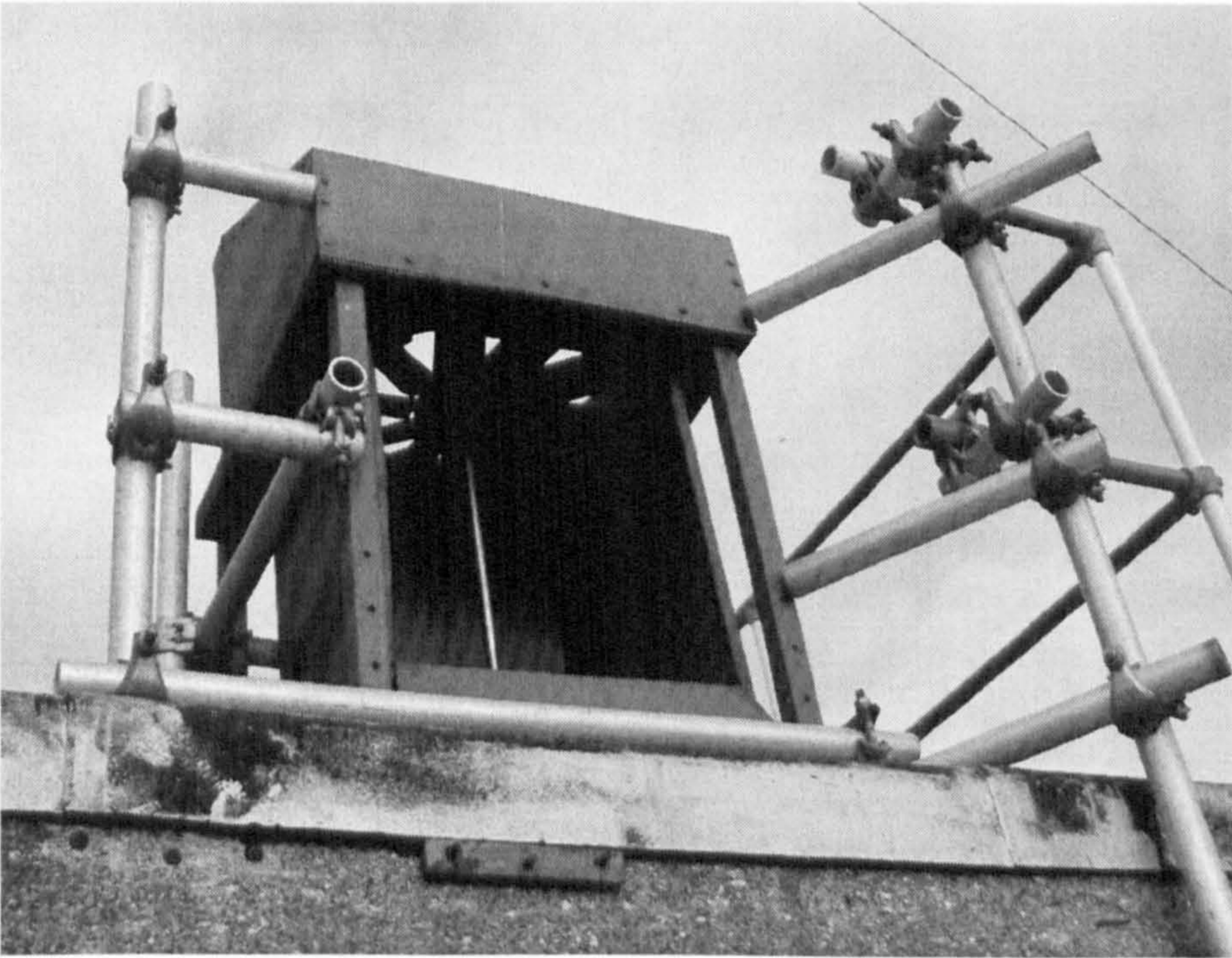
(Fig. 6.4: Ducted wind turbine)
