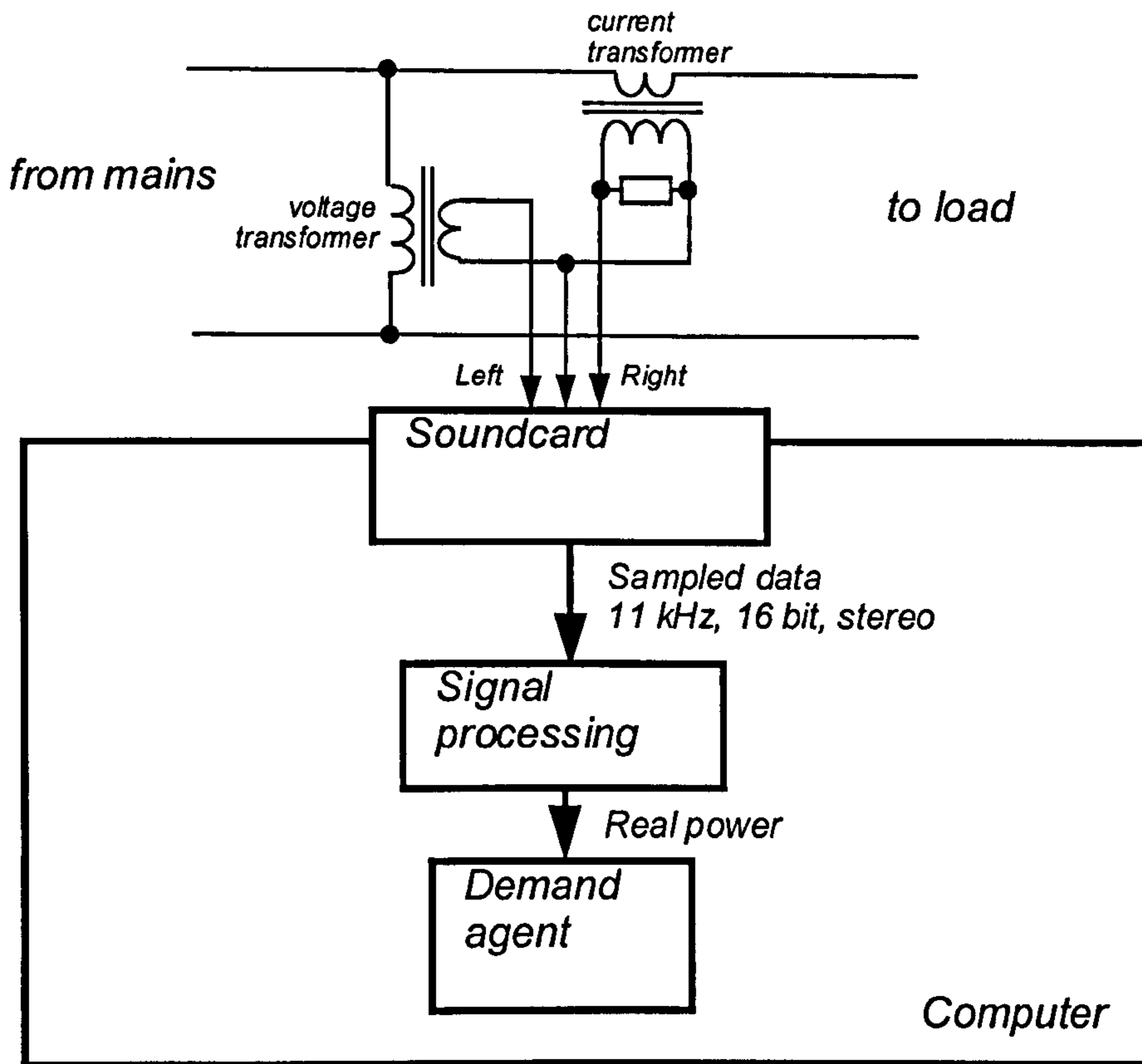
(Fig. 7.10: block diagram of power measurement hardware/software/agent)
