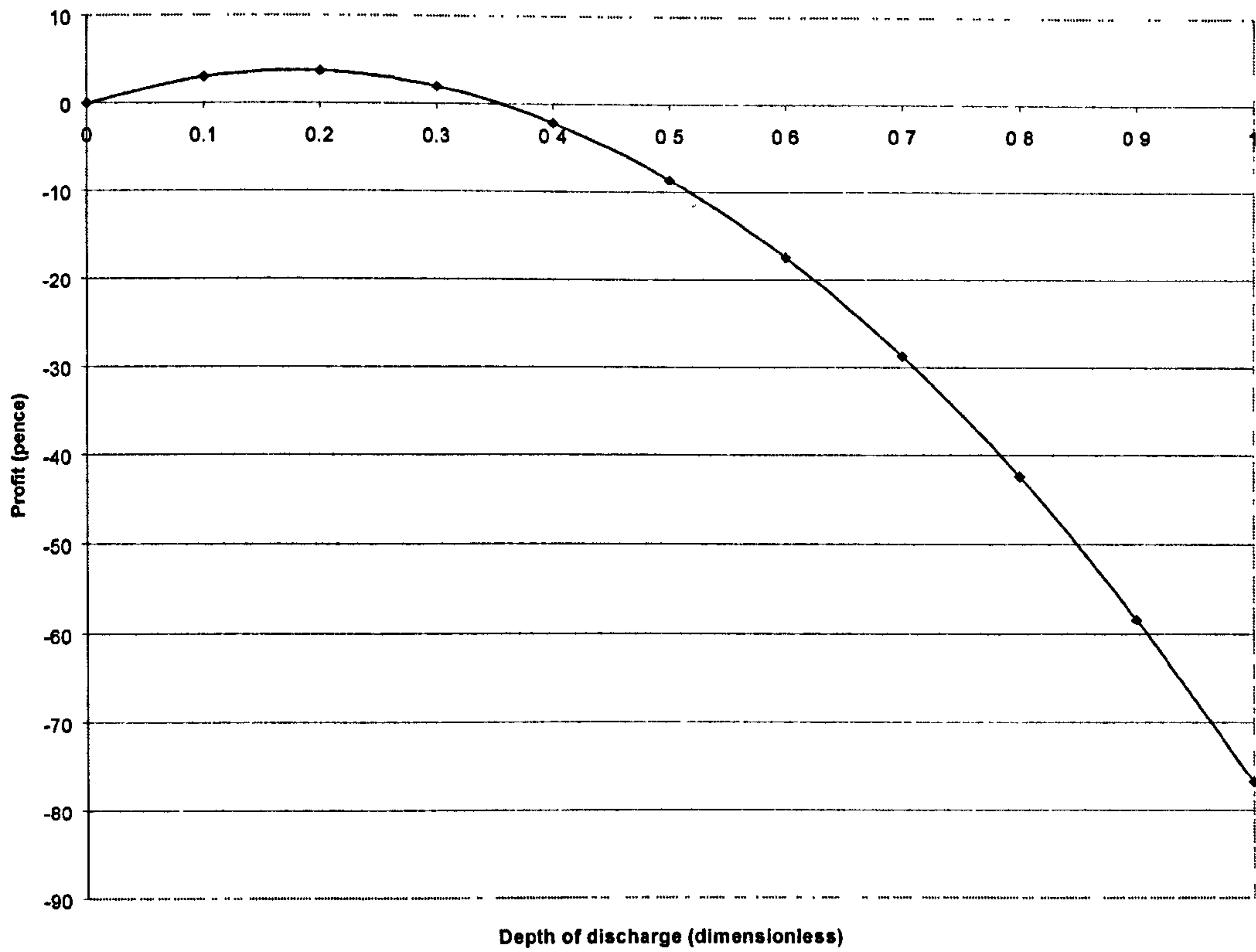
(Fig 7.1: Profit vs. depth of discharge for a sample run of economic battery management.)
