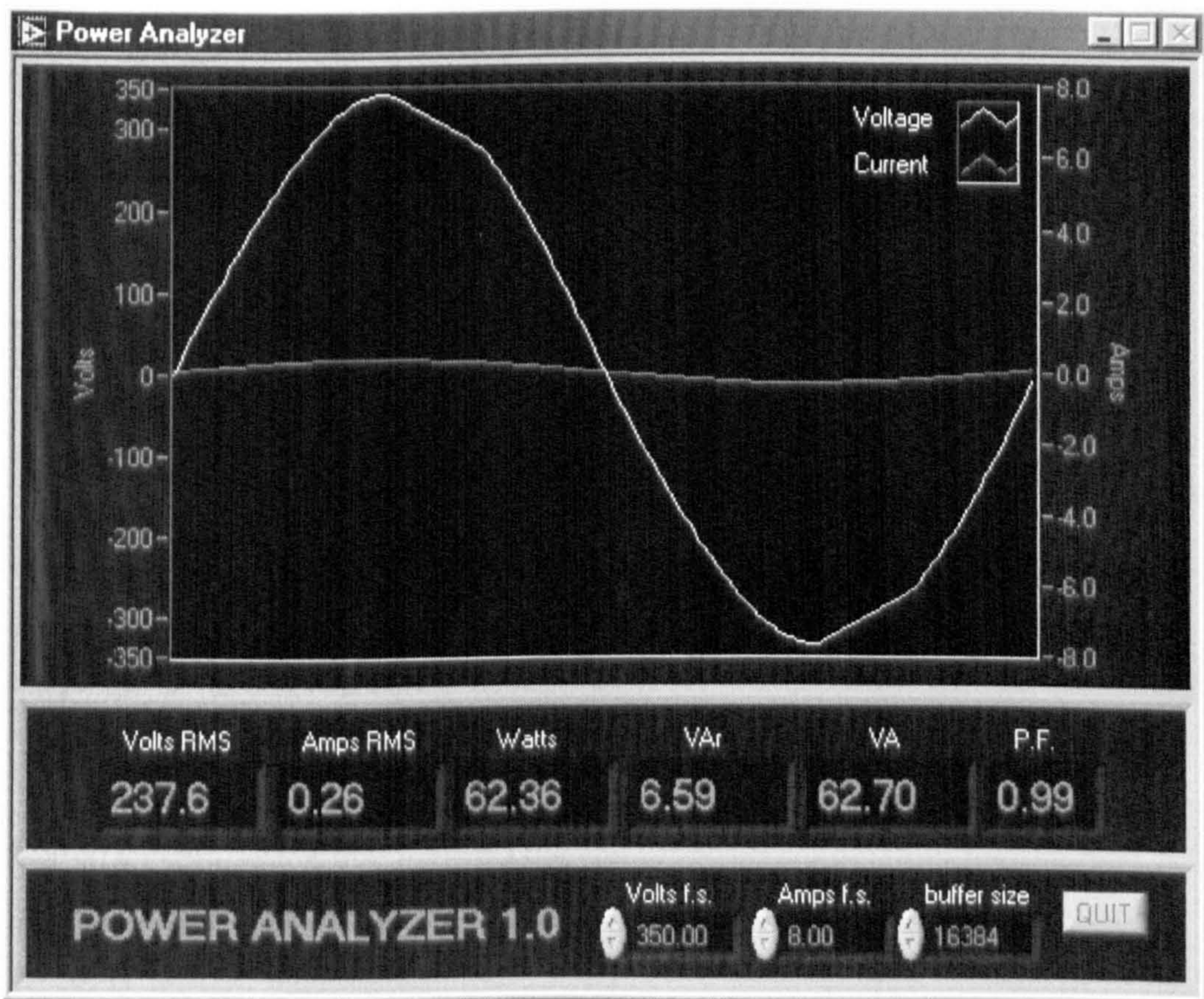
(Fig. D.4: Power analysis of 60-watt light bulb)
