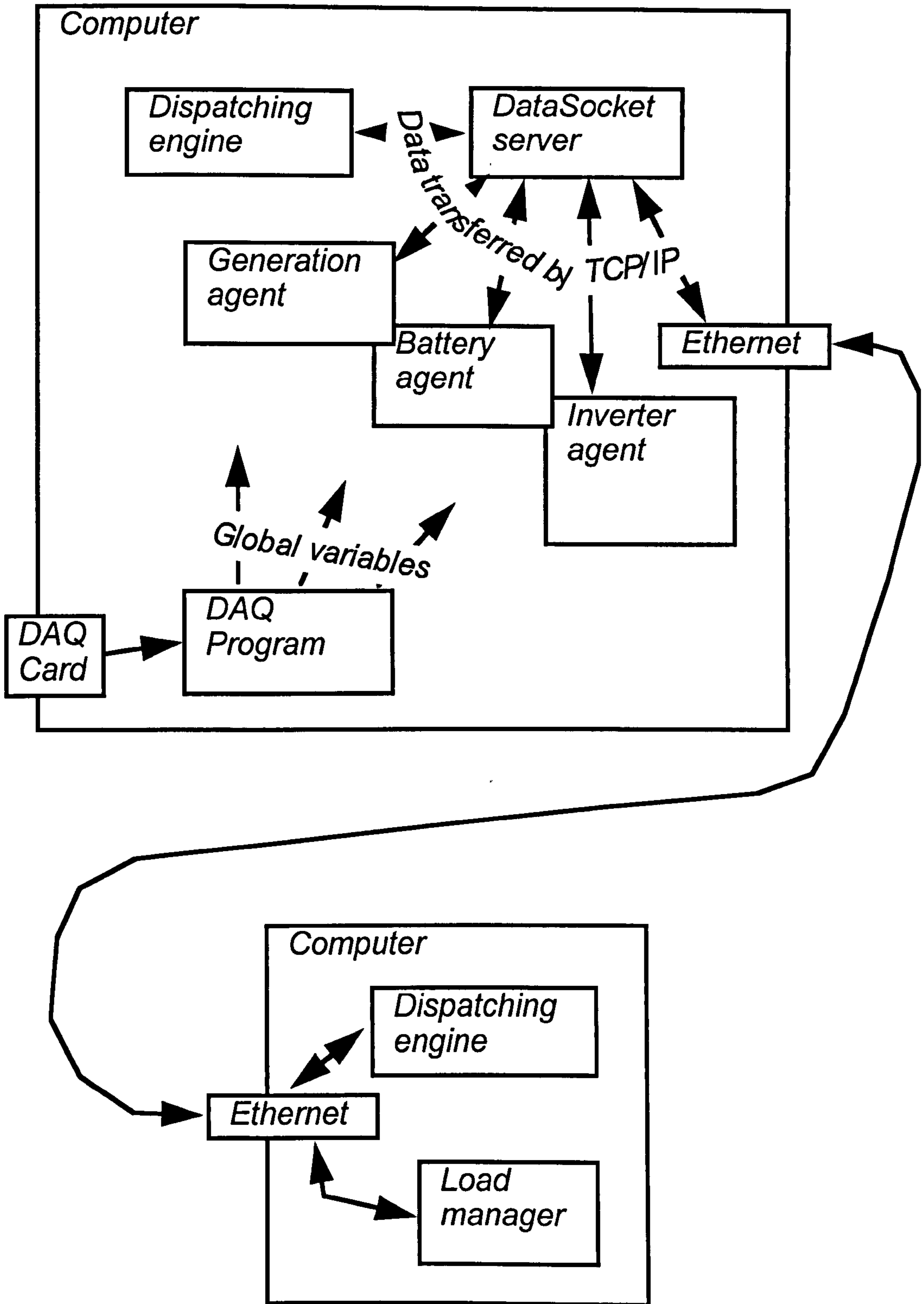
(Fig. 7.11: Software configuration of experimental system)
