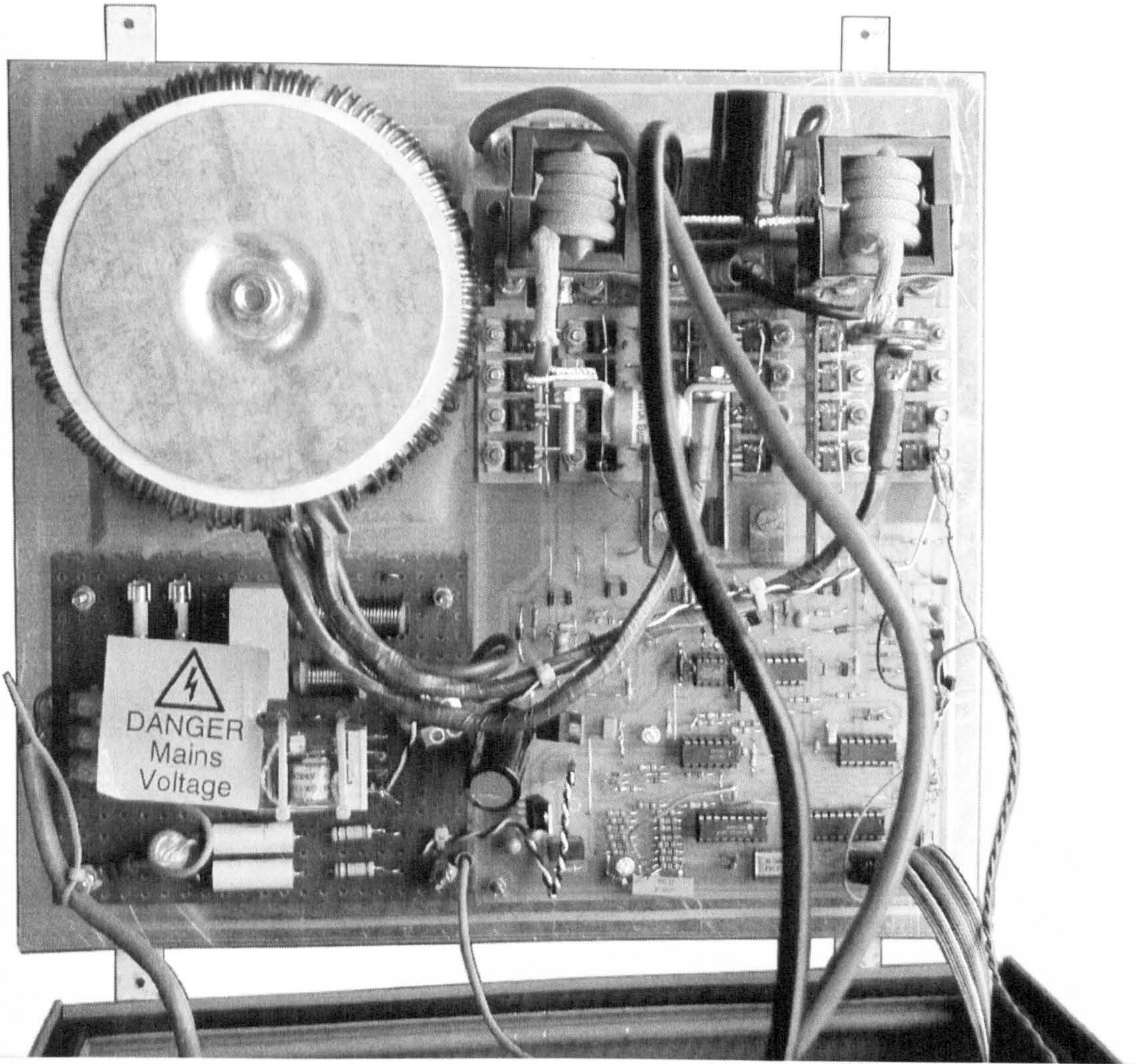
(Fig. A.15: Internal view of Mark Two inverter. Overall size approx. 250 x 300mm)
