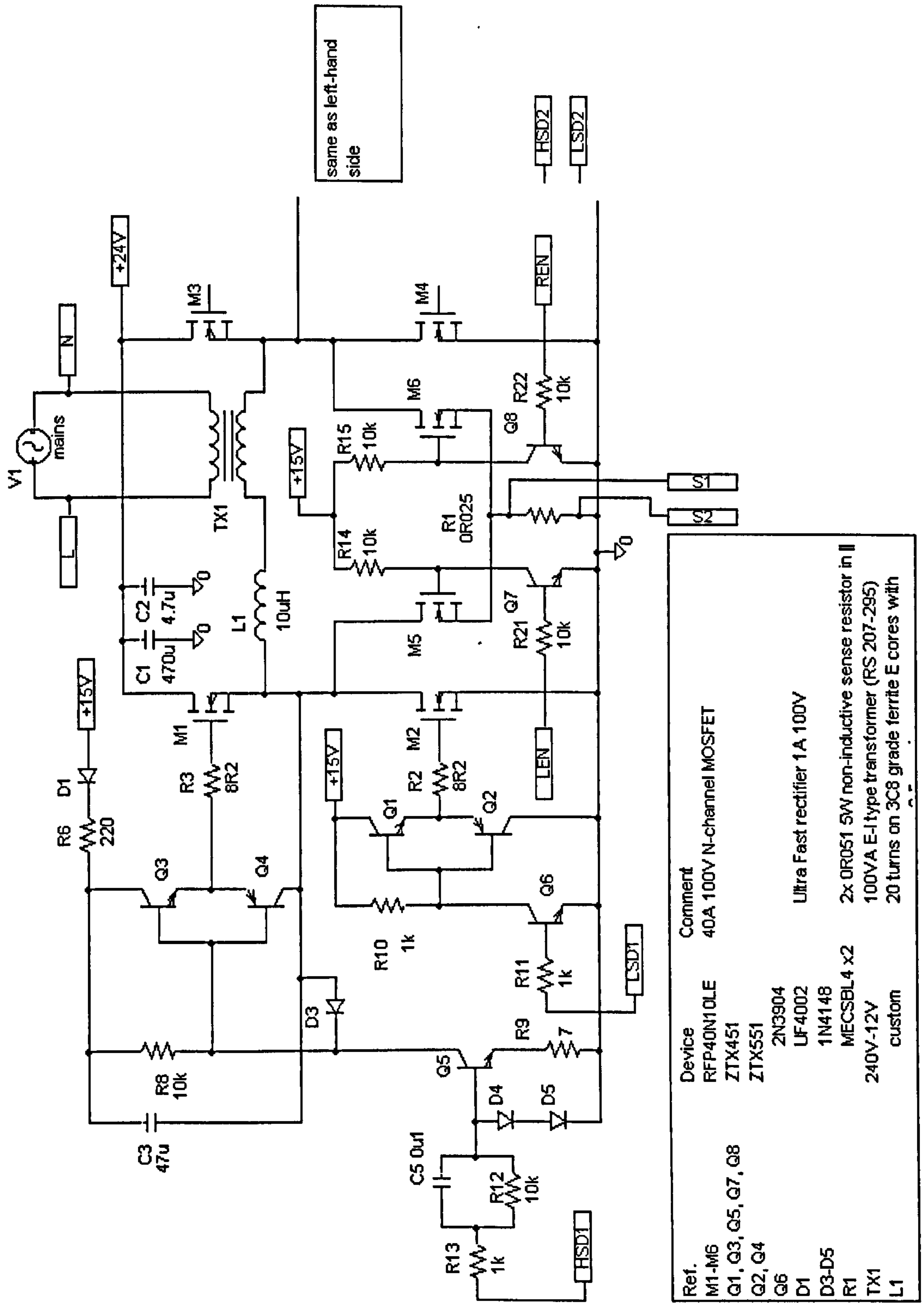
(Fig. A.11: Circuit diagram of driver stage. One half only shown.)
