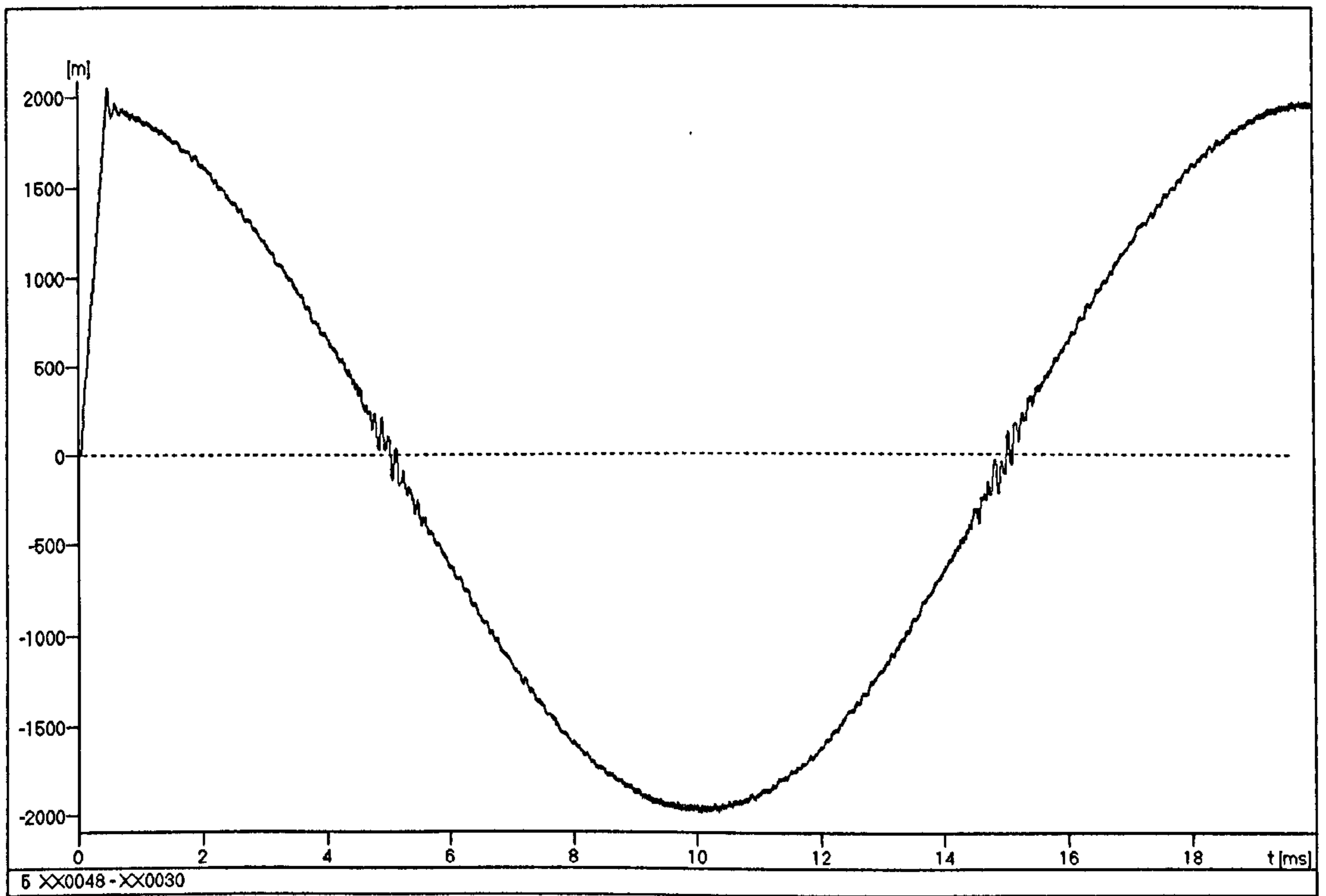
(Fig. A.8: Simulated line current waveform)
