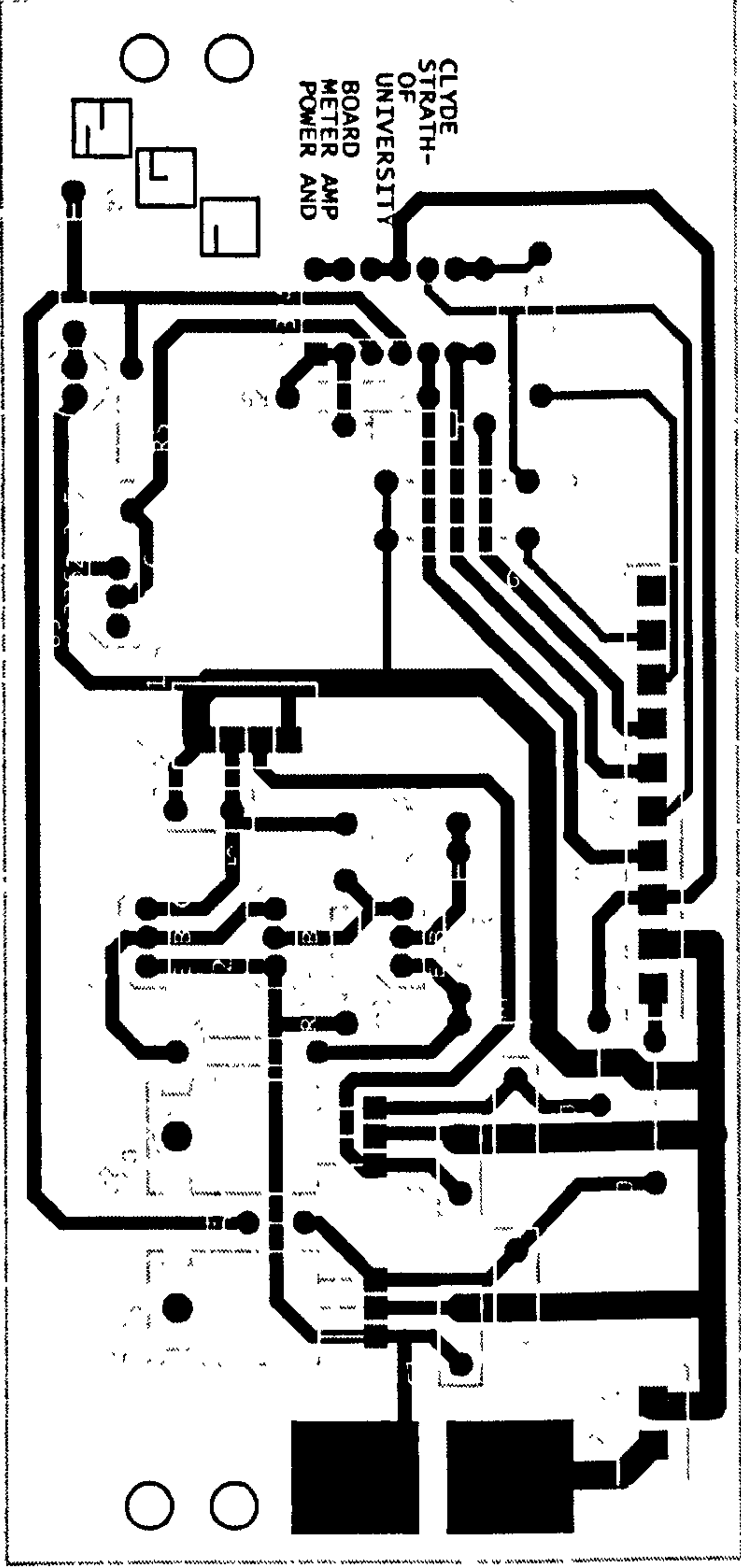
(Fig. F.5: Circuit board for power/meter module)
