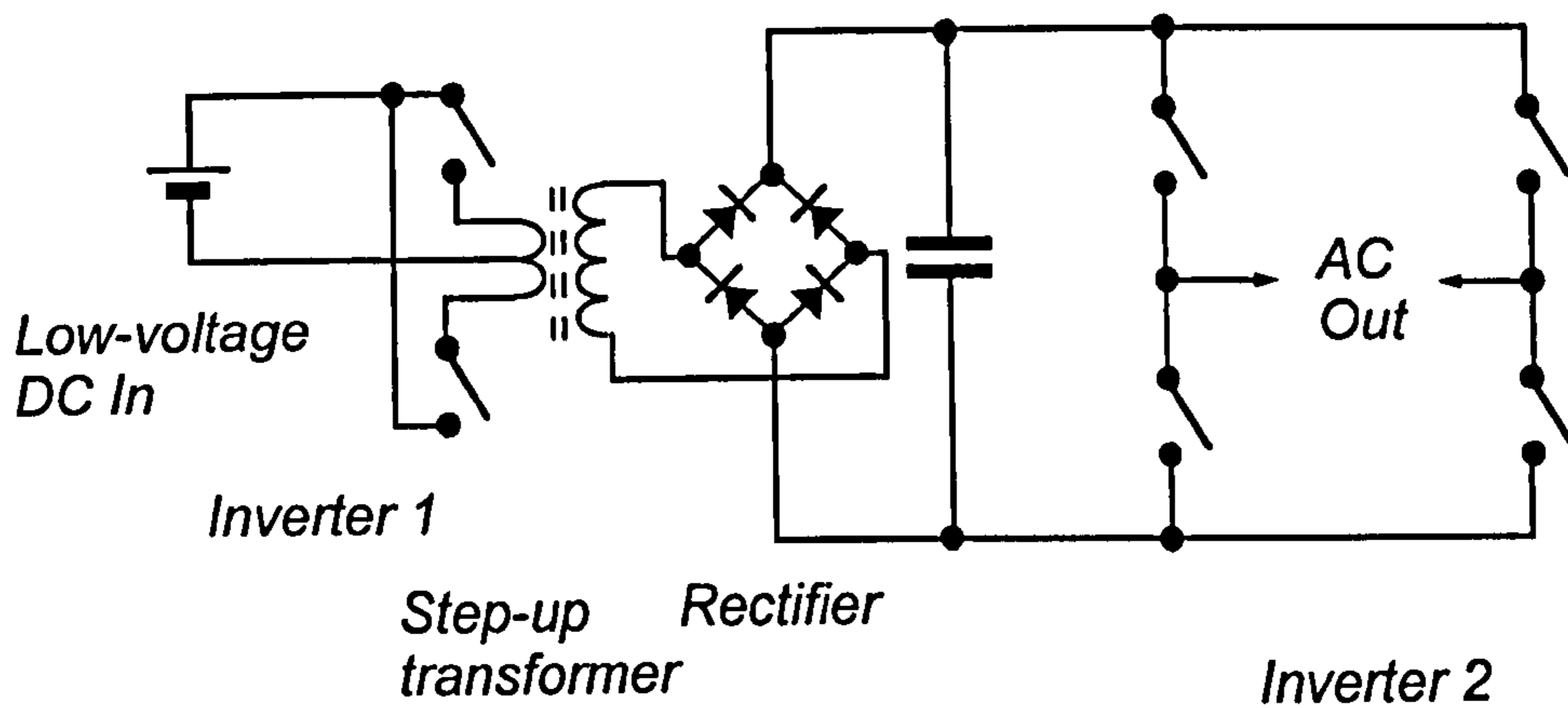
(Fig. A.3: Inverter with DC-DC converter)
