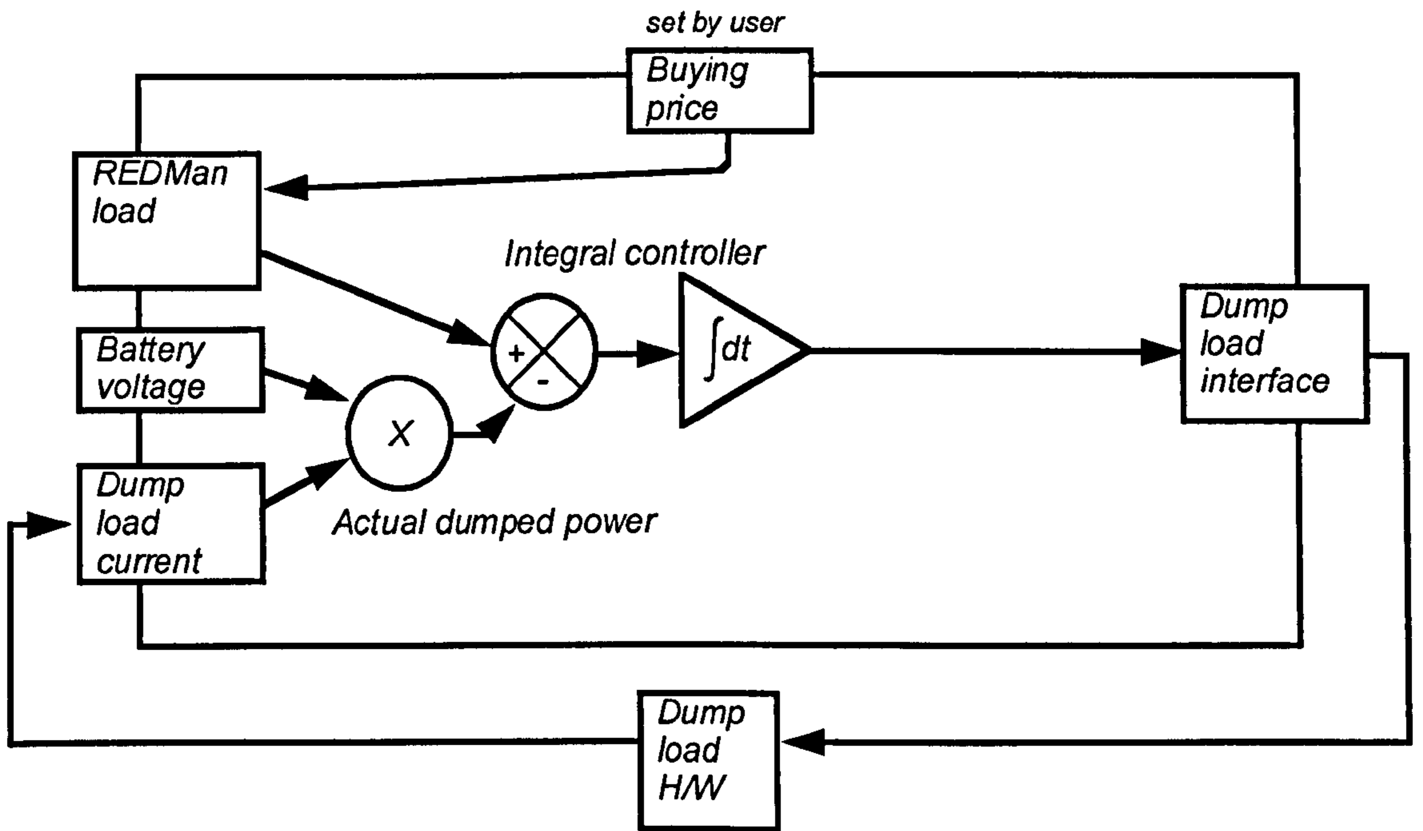
(Fig. 7.7: block diagram of dump load agent/hardware)
