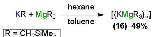
Scheme 3.7: Synthesis of 16 .
