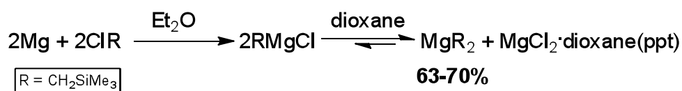
Scheme 2.1: Preparation of \text{MgR}_2
