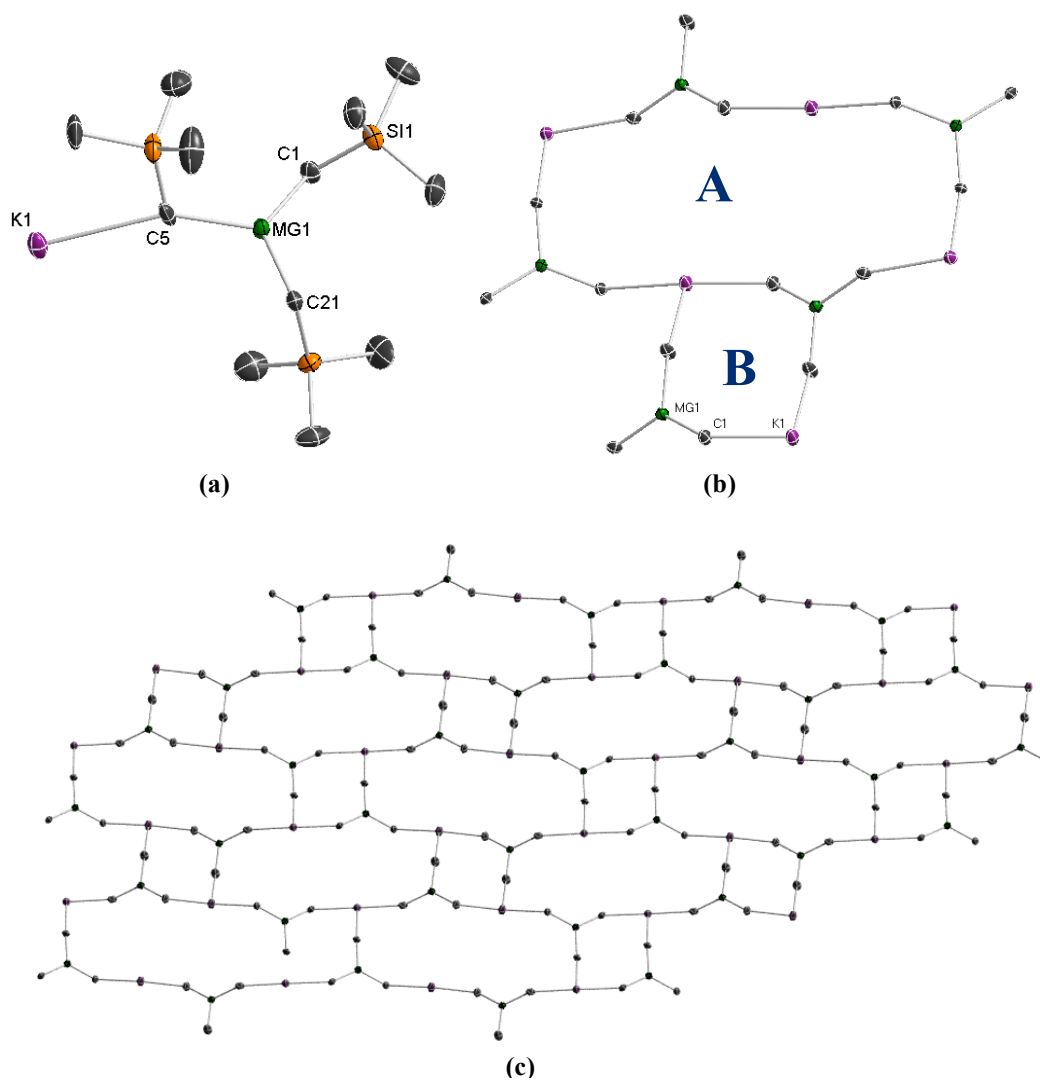
Figure 3.18: (a) T-shaped monomeric structure of 16 . (b) Sub-rings A and B made up of T-shaped \text{KMgR}_3 unites. (c) Sheet network of 16 . Displacement ellipsoids are drawn at the 50% probability level. Hydrogen atoms in all figures and TMS groups in (b) and (c) have been omitted for clarity.
