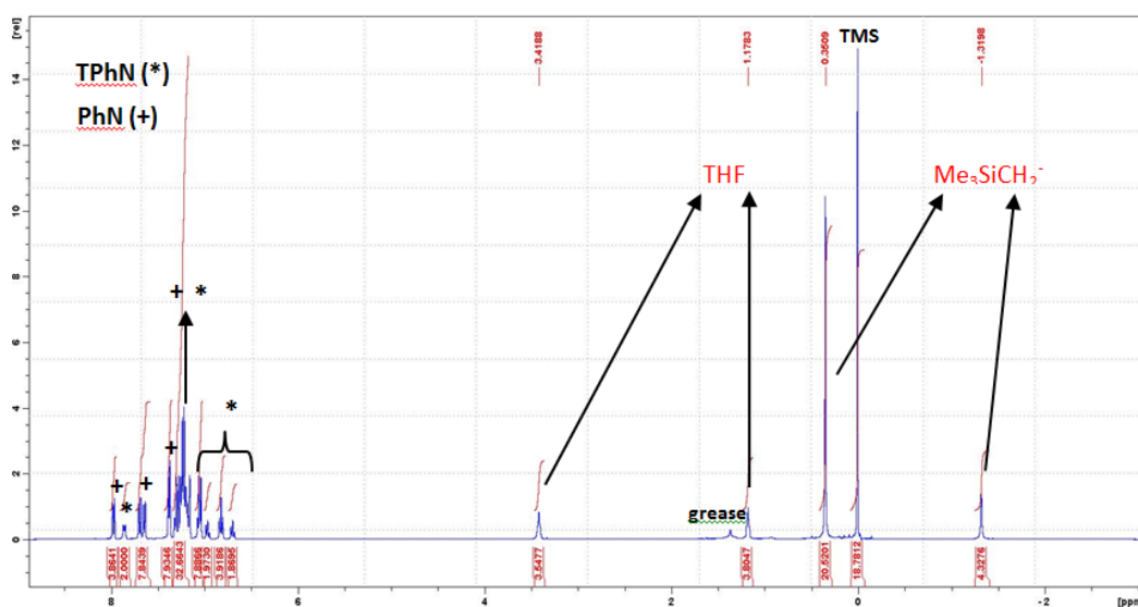
Figure 2.8: ^1\text{H} NMR spectrum of [\text{LiMg}(\text{CH}_2\text{SiMe}_3)_3(\text{THF})] ( 2 ), TPhN, PhN and TMS at 27\text{ }^\circ\text{C} in \text{C}_6\text{D}_6 (traces of grease are also observed).
