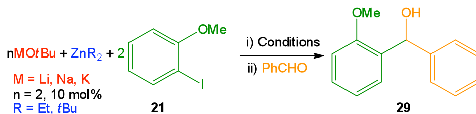
Scheme 5.12: General scheme for the synthesis of 29 under various conditions.
