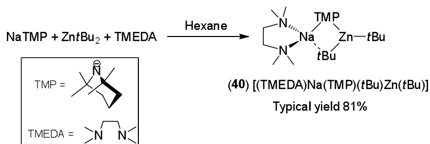
Scheme 6.11: Synthesis of monoamido/dialkyl sodium zincate 40 .
