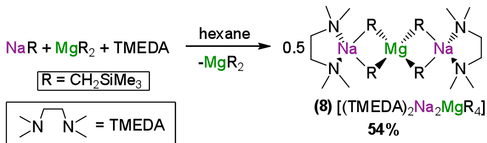
Scheme 3.1: Synthesis of 8
