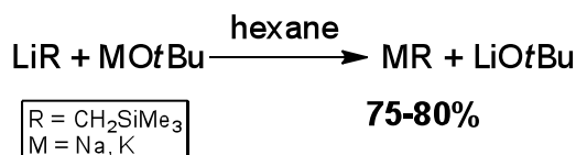
Scheme 2.2: Preparation of NaR and KR
