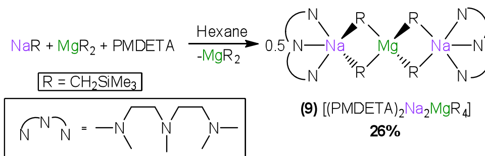
Scheme 3.2: Synthetic route to 9
