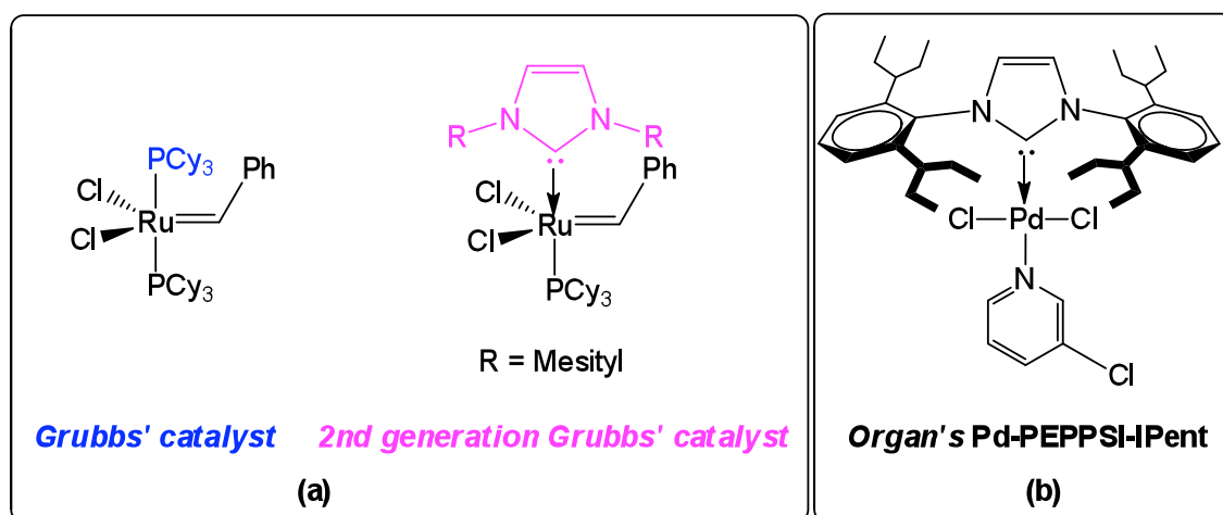
Figure 6.3: Incorporation of NHCs into catalysts for organic transformations.
