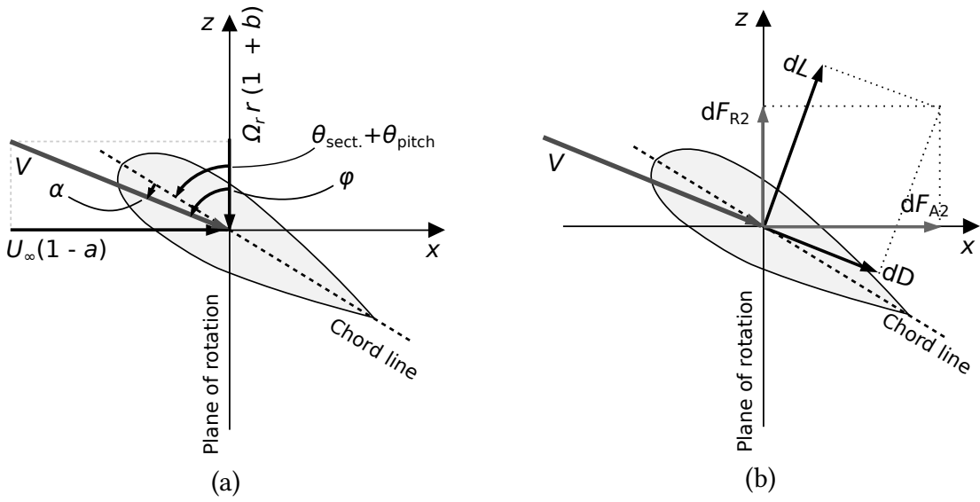
Figure 3.7: Diagrams of inflow velocity vectors (a) and induced blade-forces (b) on a blade section as viewed from the blade tip towards the hub. The inflow U_\infty is originating from the left and the rotational plane is perpendicular to the paper.
