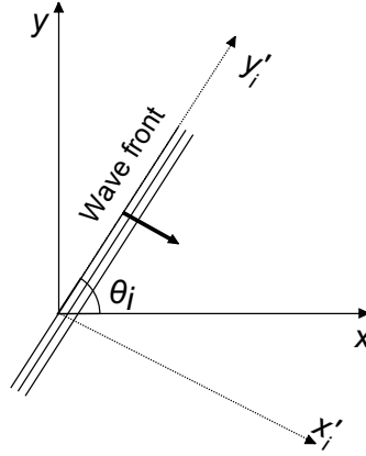
Figure 3.3: Wave-centred coordinate system transformation for each harmonic component. The vector perpendicular to the wave-front is the wave orthoganol and \theta_i is the angle of wave incidence. The kinematica of the wave component velocities are evaluated using the local coordinate x'_i .
