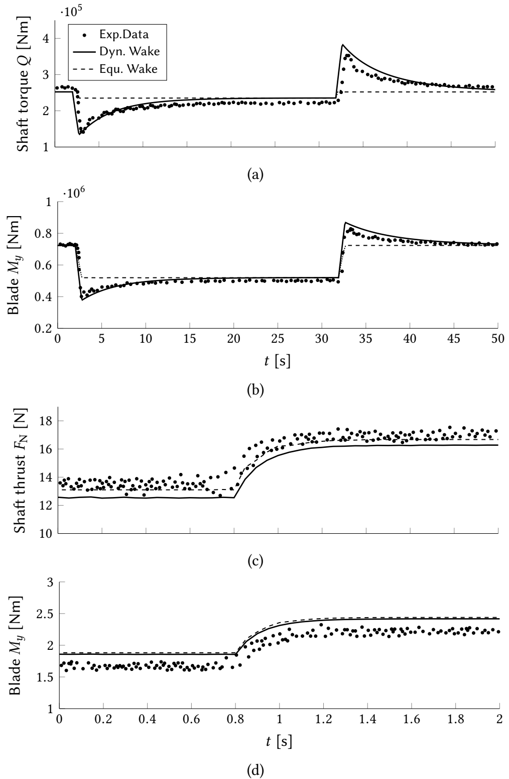
Figure 4.2: The verification of the accuracy of the dynamic wake formulation in the BEMT model. The figures show the performance of the dynamic wake model (Dyn. Wake) compared to the standard equilibrium wake solutions (Eq. Wake). The plots shown are from the 60m Øye [37] wind turbine torque signal (a) and blade out-of-plane bending moment (b), and the Snel & Schepers [41] small scale wind turbine thrust (c) and out-of-plane bending moment (d) on each respective time-axis. The pitching manoeuvres can clearly be seen in the reaction loads at 2 and 32s for the Øye case, and the inflow step-change is also visible at 0.8s for the Snel & Schepers experiment.
