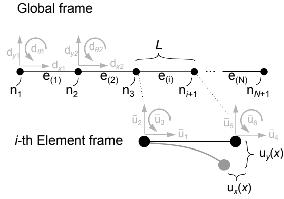
Figure C.1: 1-D array of beam elements in a global reference frame (upper) where each node is assumed to have three global degrees of freedom ( d_{x_i} , d_{y_i} , d_{\theta_i} ). The lower figure shows an element in the i -th elemental reference frame having 6 elemental degrees of freedom and two nodal displacements are highlighted to be used in the derivations below.
