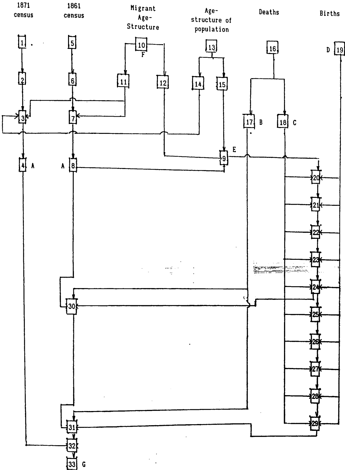
DIAGRAM 1 - THE LINKING OF SPSS-X FILES TO CREATE AN ESTIMATED 1871 CENSUS FROM THE 1861 CENSUS AND TO COMPARE IT WITH THE ACTUAL 1871 CENSUS IN ORDER TO CALCULATE EMIGRATION
