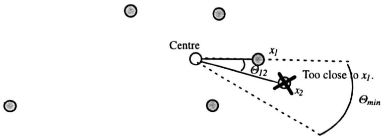
Figure 4.5: Eliminating centres with a common direction. The neighbouring points are used to define a ‘covariance’ matrix which is used to determine the overlap between neighbouring units. Neighbours in the same direction are ignored.
