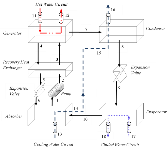
Fig 3.3 - Internal and external flows inside an absorption chiller
