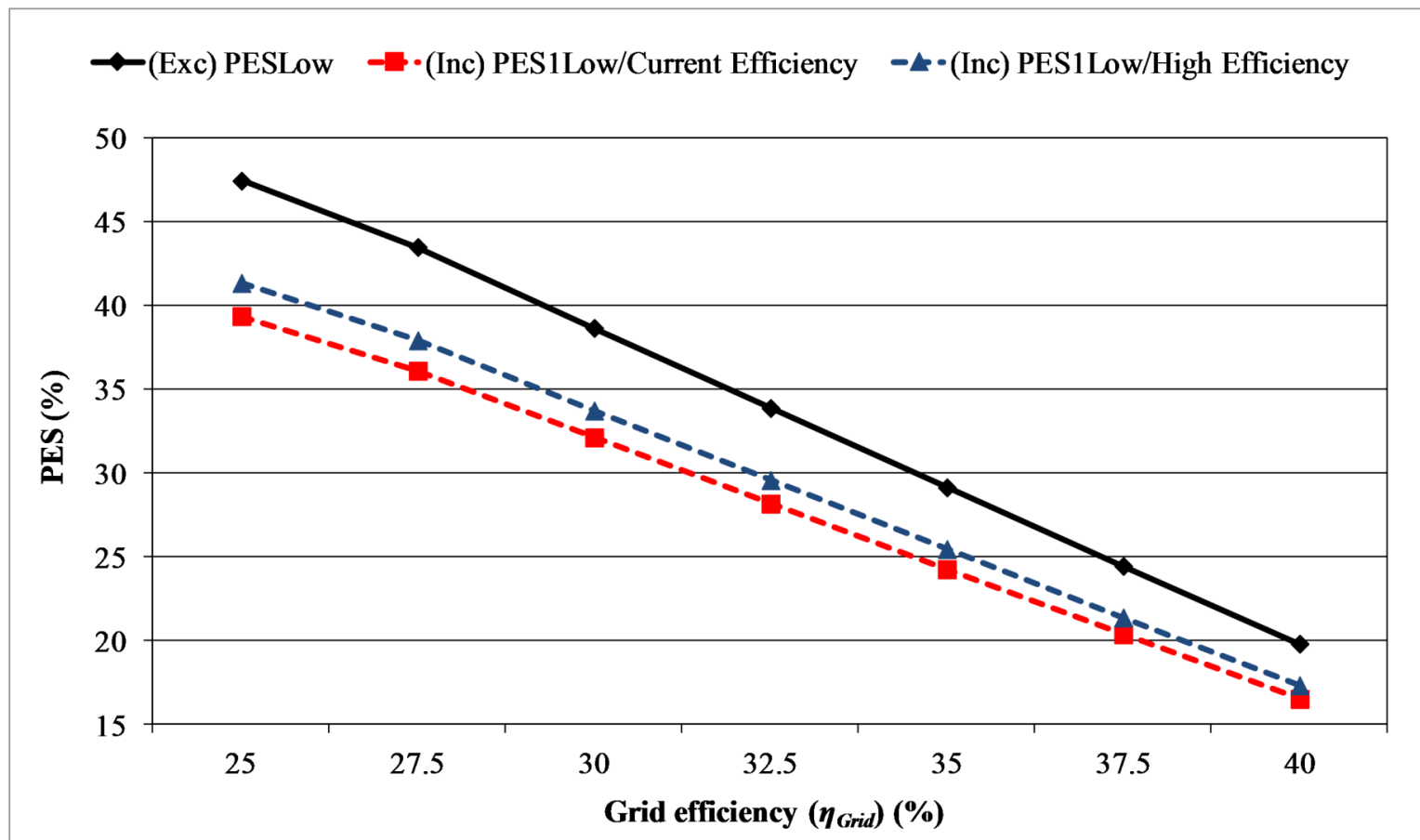
Fig. 5.7 - Sensitivity of PES to grid efficiency ( \eta_{Grid} ) (Scenario 1 Low )
