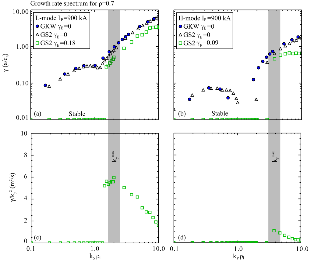
Figure 6.9: Linear growth-rate spectrum for the flux surface \rho = 0.7 in the L-mode (a) and H-mode (b) plasmas at high I_p . Calculations performed with and without flow shear using the GKW (circles) and GS2 (squares,triangles) codes respectively. The dashed lines represent the dominant linear mode in each case. Symbols along the x-axis represent the stable modes found. The mixing length estimates for the simulations with flow shear included is shown respectively for each case in (c) and (d).
