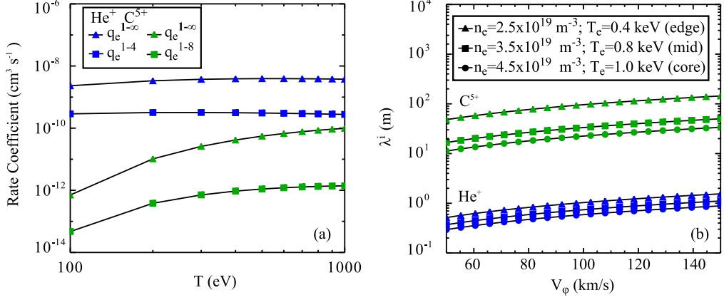
Figure 3.4: (a) The relevant electron impact excitation and ionisation rates for the plume ions and (b) the ionisation mean free path of the He + and C 5+ plume ions as a function of the ion toroidal velocity for three different regions of the plasma.
