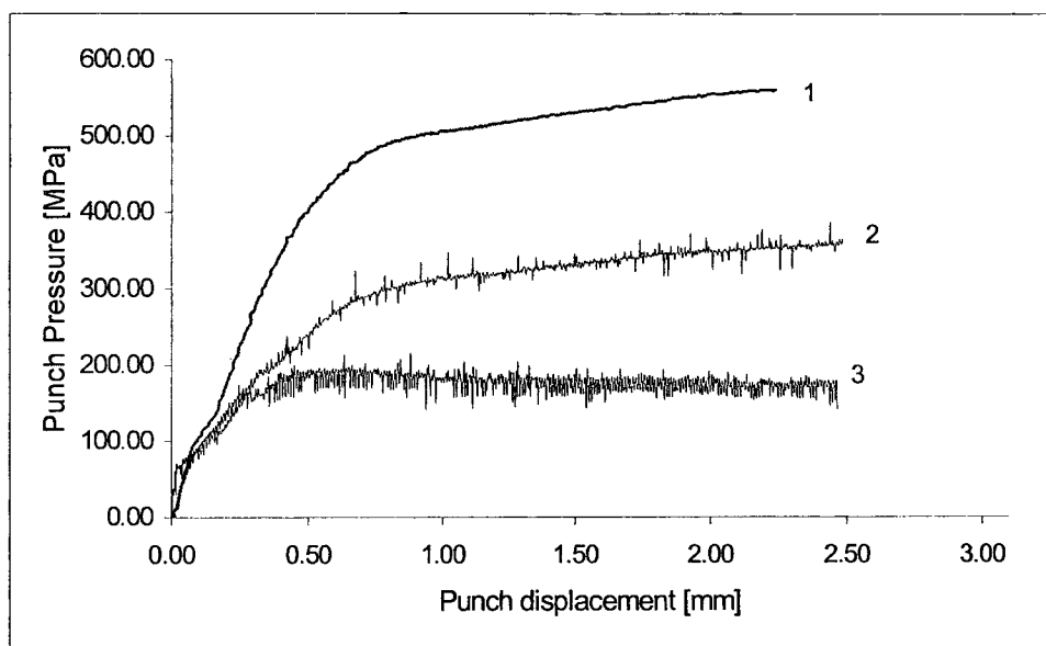
Fig.7.2.3-8 Back extrusion. Punch pressure versus punch displacement, deformation velocity v=1.0\text{mm/s} ; (1) without vibration, (2) amplitude of vibration A=4.5\mu\text{m} , (3) amplitude of vibration A=8.5\mu\text{m} .
