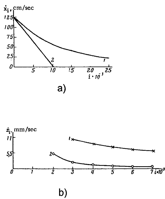
Fig.2.1.2-2 (a) Theoretical variation of the velocity of the body during the motion over a tangentially vibrating surface (1) and at the absence of vibration (2), (b) Experimental results for different initial velocities. In both diagrams time is expressed as i = t \cdot \omega / \pi . [39]
