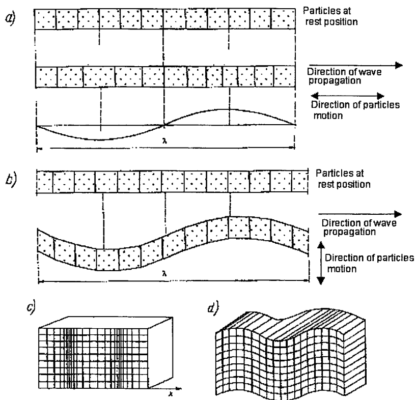
Fig.1-4. Longitudinal (a) and transverse (or shear) waves. D3 image of longitudinal (c) and transverse (d) waves.[100]
