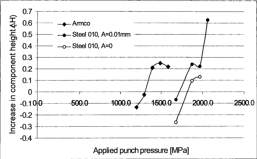
Fig.7.2.3-5 Back extrusion. Increase in component height versus pressure applied to the punch. Amplitude of vibration 10 \mu m. Punch diameter 3mm. Specimen material – Iron Armco and Steel 010.
