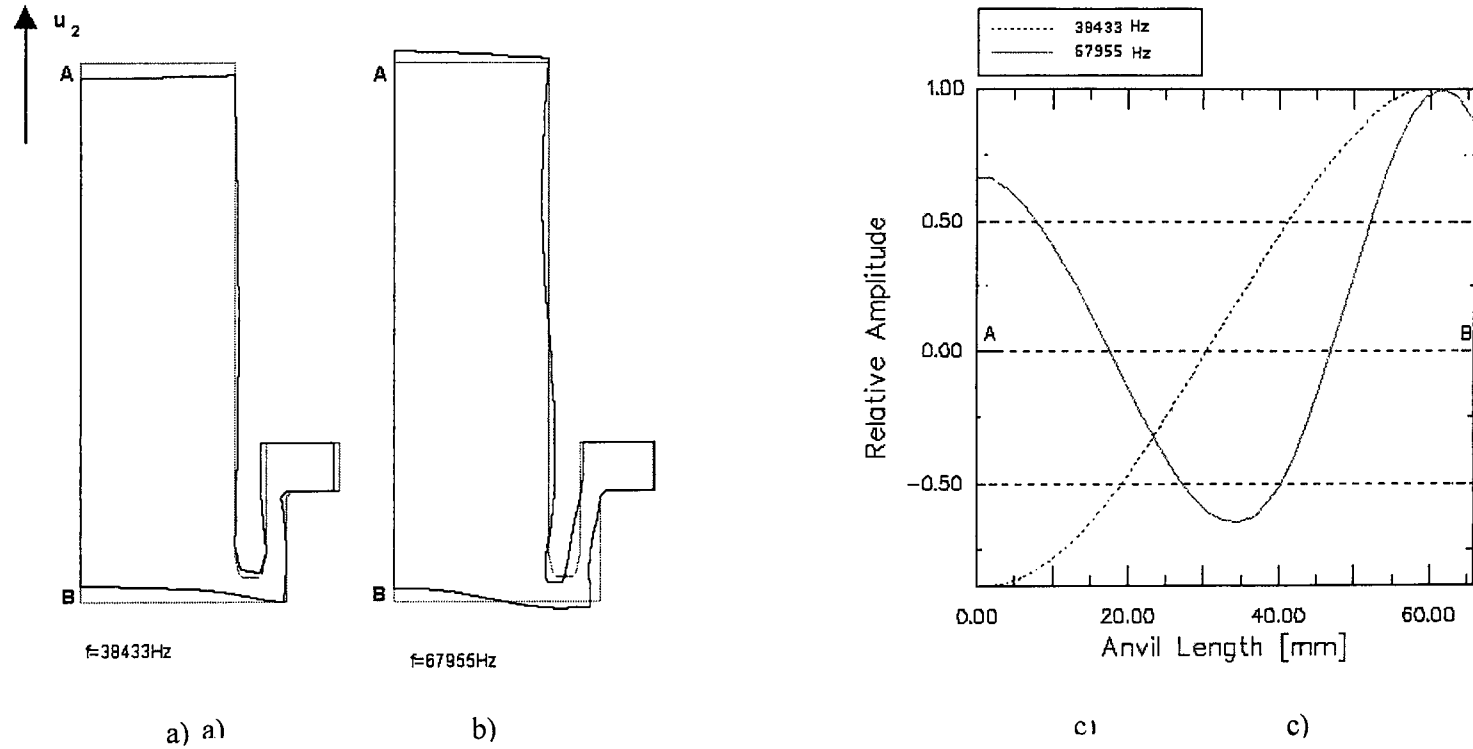
Fig.4.5.4-3 Mode of vibration (undeformed and deformed shape) at frequency (a) 38433Hz, (b) 67955Hz., (c) Amplitude distribution along the axis AB
