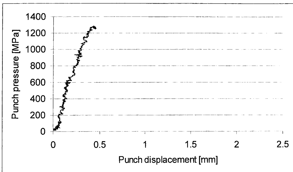
Fig.7.2.3-15 Punch pressure versus punch displacement for the steel specimen and nominal amplitude of vibrations A=8.5\mu\text{m} .
