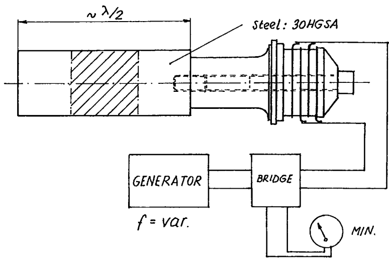
Fig.4.4.3 -1 Scheme for sound velocity measurement.
