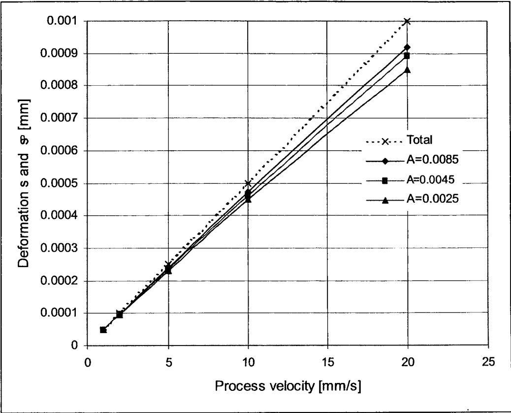
Fig.8.2.2-14 Total deformation over one period of vibration and its component attributed to the punch for amplitudes of 0.0085, 0.0045, 0.0025mm.
