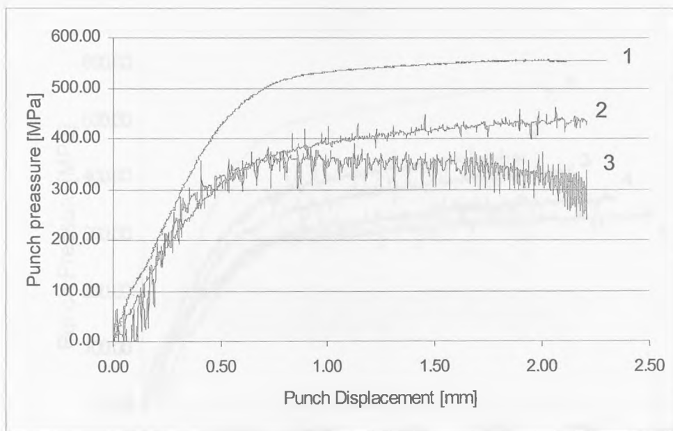
Fig.7.2.3-10 Back extrusion. Punch pressure versus punch displacement, deformation velocity v=10\text{mm/s} ; (1) without vibration, (2) amplitude of vibration A=3.0\mu\text{m} , (3) amplitude of vibration A=7.5\mu\text{m} .
