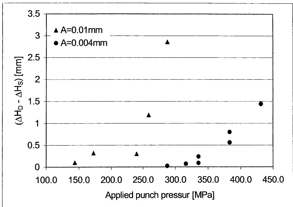
Fig.7.2.3-4 Back extrusion. Increase in the component height caused by the application of vibration with amplitude of 10 and 4, \mu\text{m} . Punch diameter 3mm. Specimens – Al-2.
