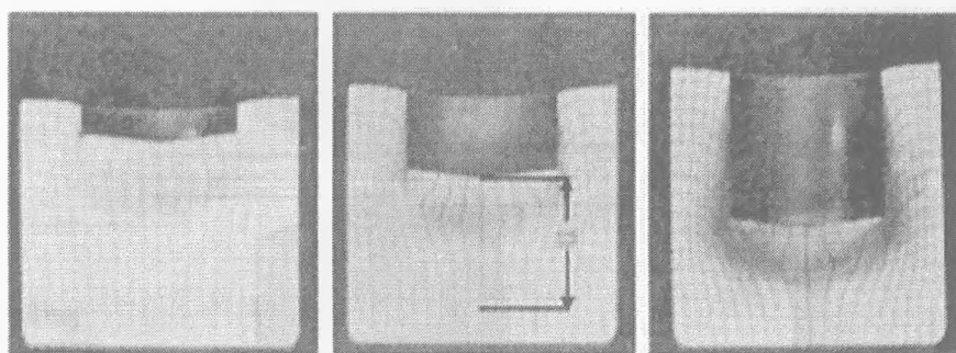
Fig.4.5.1-6 Material flow in can extrusion; u – the height of the deformation zone. [101]
