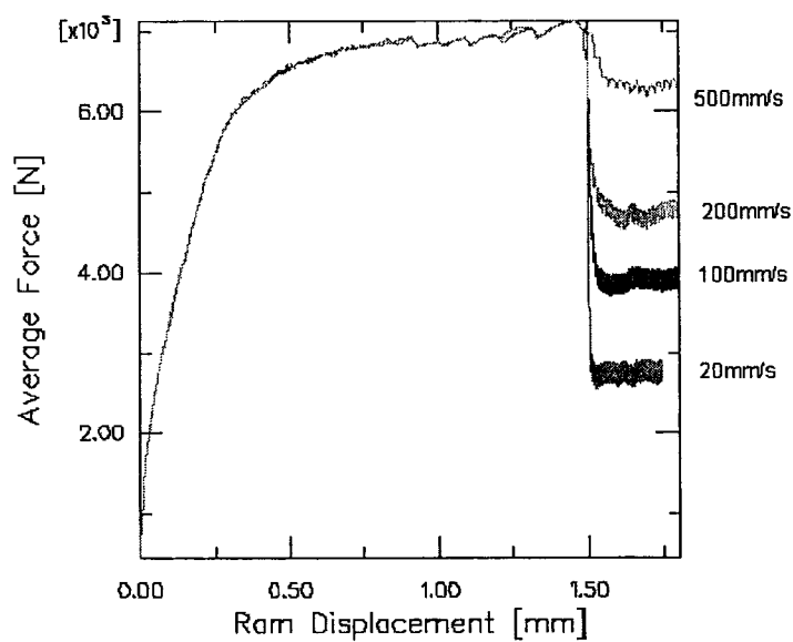
Fig.7.3.2-6 Average forming force versus displacement for anvil velocities of 20, 100, 200 and 500mm/s.
