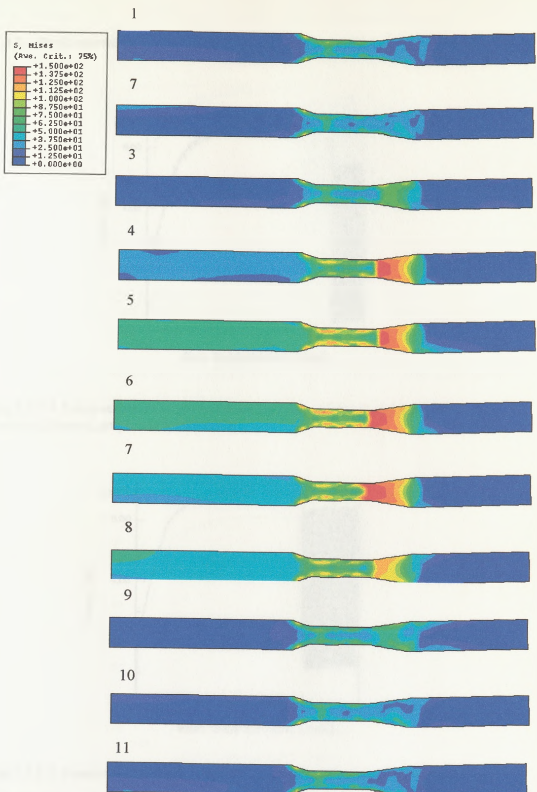
Fig.7.3.1-6 Distribution of equivalent stress in the flattened wire with vibration imposed to the tool at 10 moments equally spaced during one vibration cycle.
