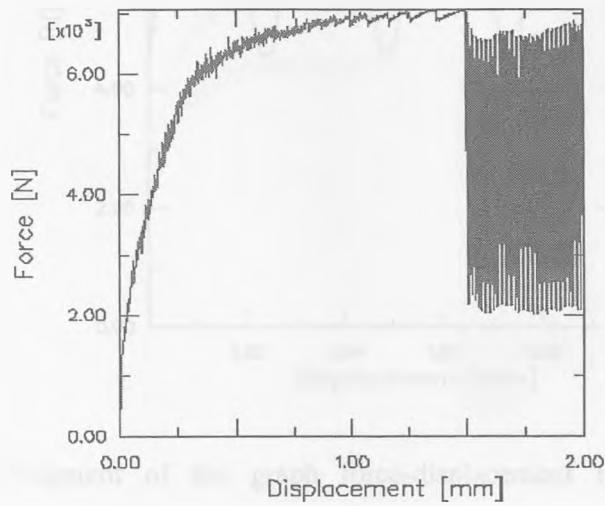
Fig.7.3.2-3 Force versus anvil displacement for back extrusion Aluminium (anvil velocity 200mm/s, amplitude 0.0085mm).
