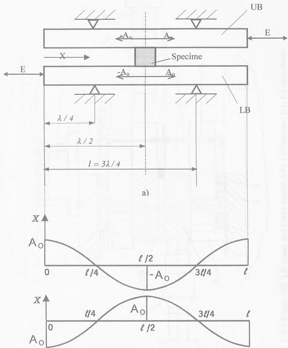
Fig.4.4.1-1 Concept of WT/P tool (a), amplitude of vibration along the length of the beams; UB-upper beam, LB – lower beam, E-excitation, A_0 -amplitude, l -beam length, X - direction.
