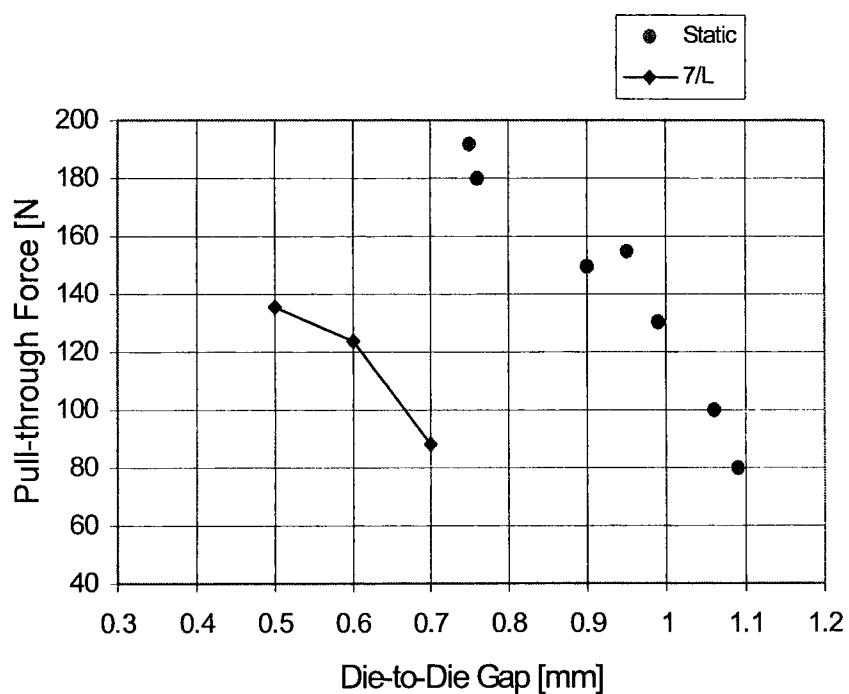
Fig.7.2.4-2 Pull-through force versus die-to-die gap for AL-G21 wire, \Phi = 1.2\text{mm} . L – under lubricated condition, amplitude of vibration – 0.007mm.
