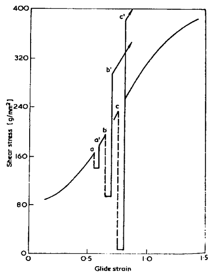
Fig.2-2 Acoustic softening by low power ultrasonic vibrations and acoustic hardening by high power ultrasonic vibrations in zinc crystal during tensile deformation. [1]
