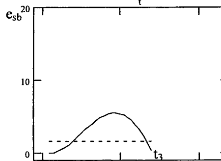
Fig.8.2.2-5 Changes in the elastic deflection of the work-material with time during unloading and reloading.
