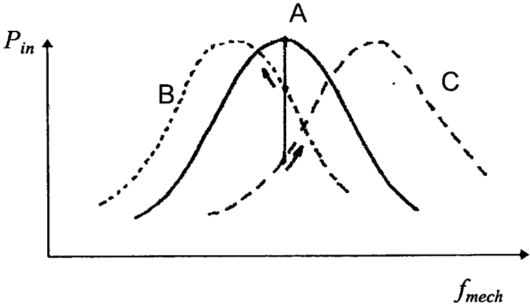
Fig.4.1.2-4 Generator output power versus frequency.
