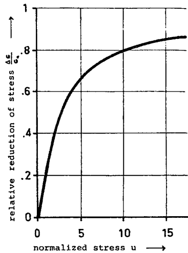
Fig.2.1.1-2 Relative reduction in static stress \Delta\sigma/\sigma_A ; \Delta\sigma - stress reduction, \sigma_A - amplitude of vibrational stress, normalised stress u = C \sigma_A . [32]
