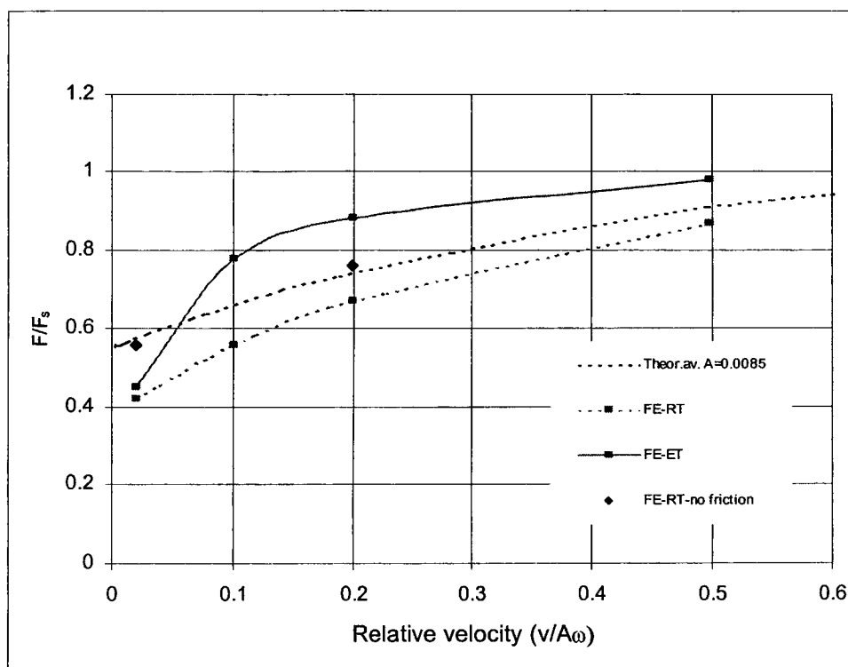
Fig.8.2.2-11 Comparison of the results obtained in EF simulations to the theoretical curves from Fig.8.2.2-9.
