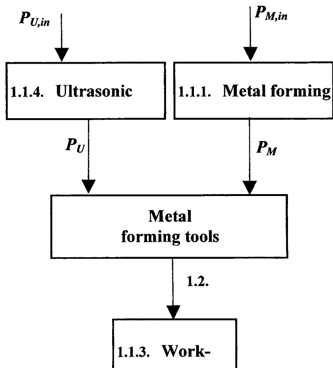
Fig.8.2.3-7 The flow of power in the UMFORM (power losses not shown). Subscripts refer to input powers.
