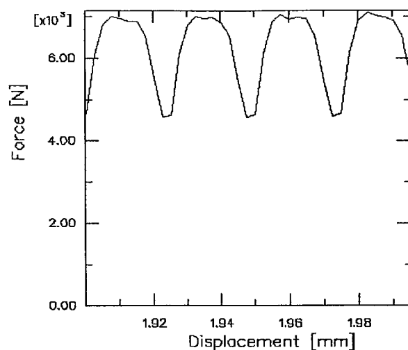
Fig.7.3.2-5 Fragment of the graph force-displacement for back extrusion of Aluminium for an anvil velocity of 500mm/s and amplitude of 0.0085mm.
