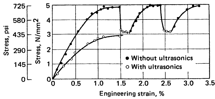
Fig.2-1 Effect of superimposed 800kHz ultrasound on the tensile deformation of zinc crystal. Specimen coupled to ultrasonic generator by immersion in insolated liquid bath. [5]
