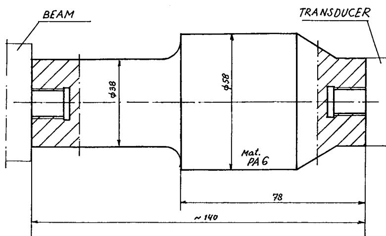
Fig.4.3-6 Booster (material PA6).
