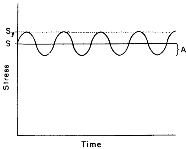
Fig.2.1.1-1 Superposition of steady and alternating stress to cause yielding. [6]
