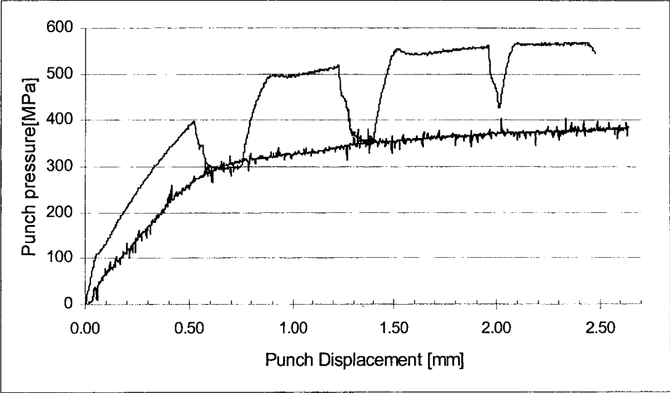
Fig.7.2.3-6 Punch pressure versus punch displacement; (1) vibration applied from the beginning of the process, (2) vibrations imparted to the punch for short time within the process.
