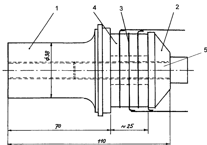
Fig.4.3-4 Transducer – (1) head (material PA6), (2) cap (material 30HgsA), (3) connection tags (material B7), (4) piezoelectric rings (material PZ-28)
