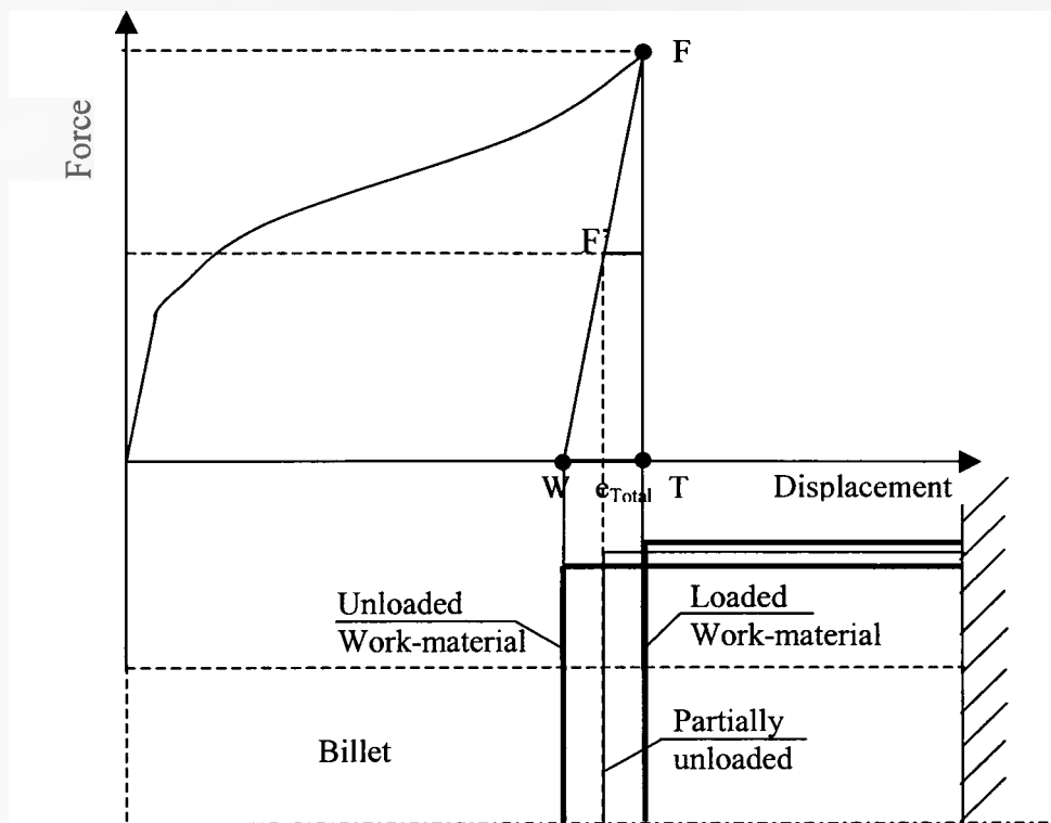
Fig.8.2.2-7 Relationship between load and spring back of the work-material.
