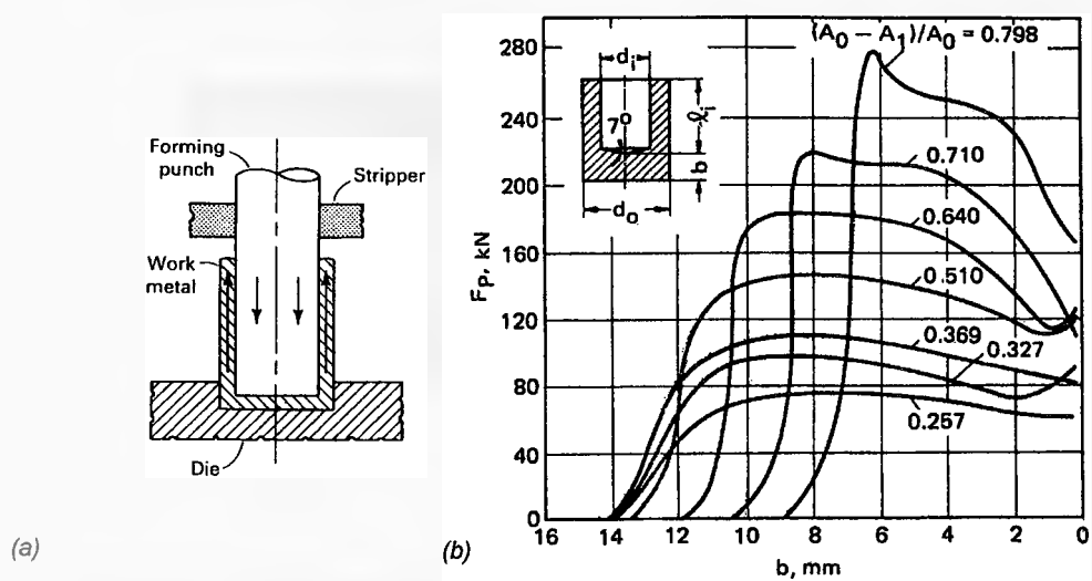
Fig.4.5.1-5 Back extrusion scheme (a), forming force for different reduction versus the bottom thickness. [101]
