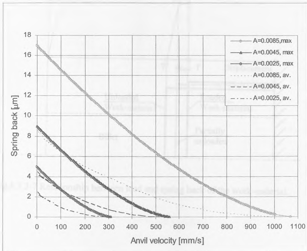
Fig.8.2.2-6 Variation of the maximum and average springback with velocity of the anvil for amplitudes of vibration 0.0085, 0.0045 and 0.0025mm.
