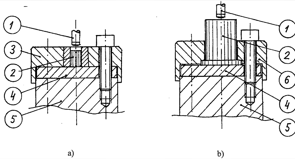
Fig.4.5.2-2 The die assembly used for backward extrusion (a) and indentation (b); 1 -punch WT/I-1.06, 2 - specimen, 3 - die, 4 - hard washer, 5 - anvil, 6 - specimen holder
