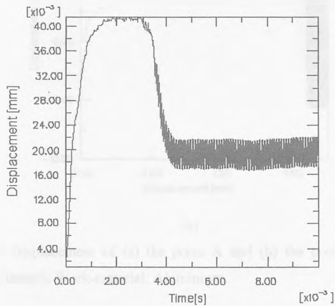
Fig.7.3.2-15 Displacement of the point C with ram displacement at a velocity of 20mm/s. Work-material: Aluminium.
