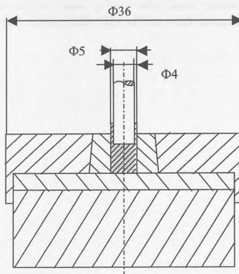
Fig.8.2.2-8 Die for back extrusion.
