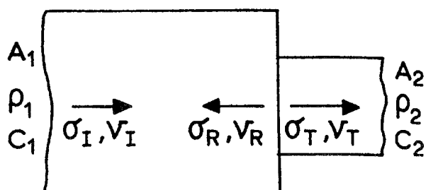
Fig.1-5. A bar with a vary cross-sectional area ( A_1 and A_2 ) and properties ( c_1 , \rho_1 and c_2 , \rho_2 respectively). [4]
