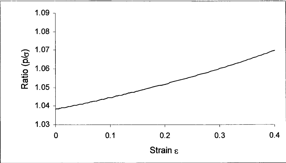
Fig.8.1-1 Variation of ratio of mean pressure to Yield Strength with strain \mu=0.1 .
