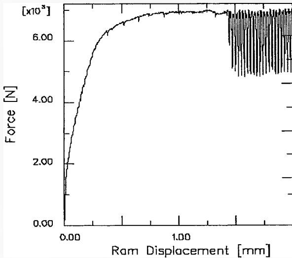
Fig.7.3.2-4 Force versus anvil displacement for back extrusion Aluminium (anvil velocity 500mm/s, amplitude 0.0085mm).
