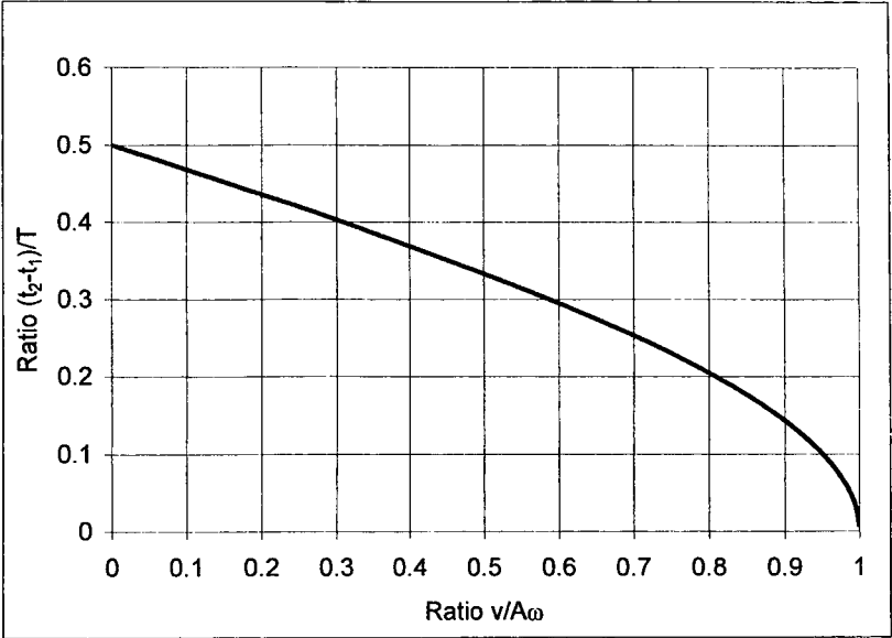
Fig.8.2.2-3 Variation of the ratio of the period (t_2 - t_1)/T , with relative anvil velocity (v/A\omega) .
