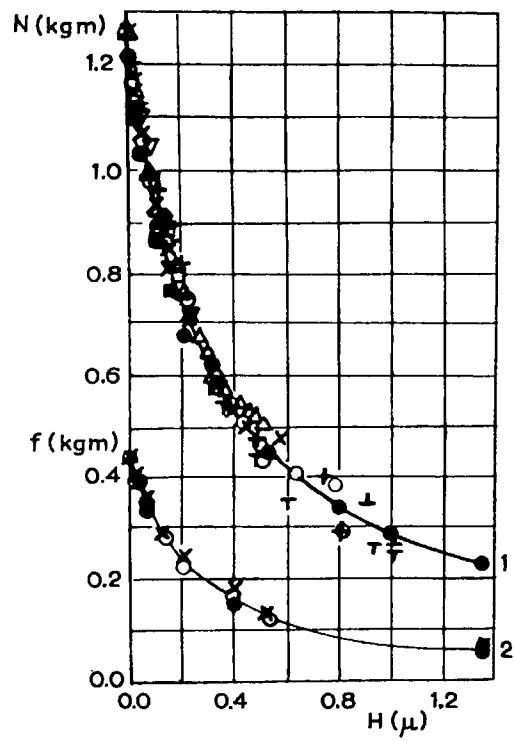
Fig.2.1.2-3 Net normal load ( N , curve 1) and static friction force ( f , curve 2) plotted against the distance between the bodies.[14]
