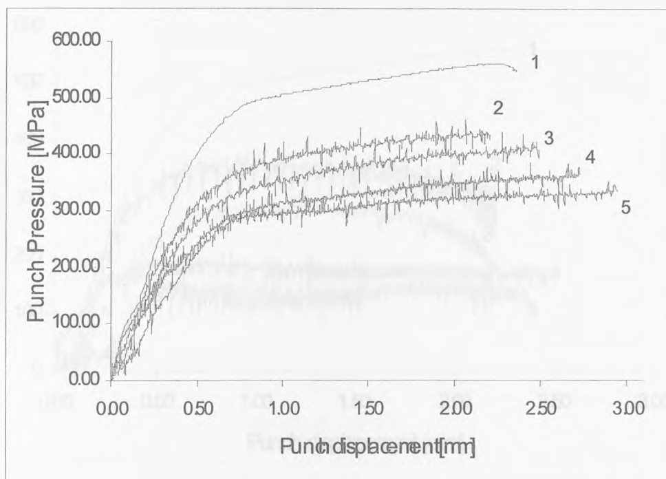
Fig.7.2.3-11 Punch pressure versus punch displacement for the nominal amplitude of vibrations A=4.5\mu\text{m} : (1) without vibration, (2) v=10\text{mm/s} , (3) v=5\text{mm/s} , (4) v=1\text{mm/s} , (5) v=0.5\text{mm/s} .
