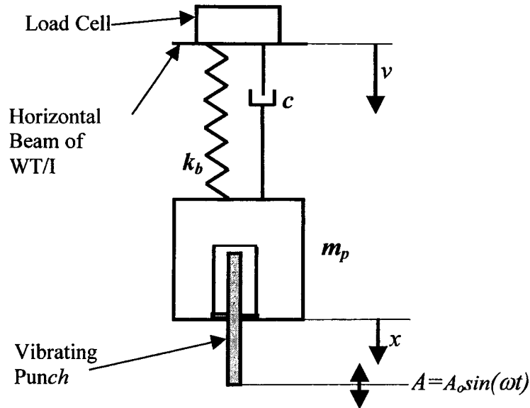
Fig.8.2-1 Scheme for force measurement; k_b – beams stiffness, m_p – mass of the upper plate and beams, c – damping, v – ram velocity, x – displacement of the upper plate, A – punch amplitude.
