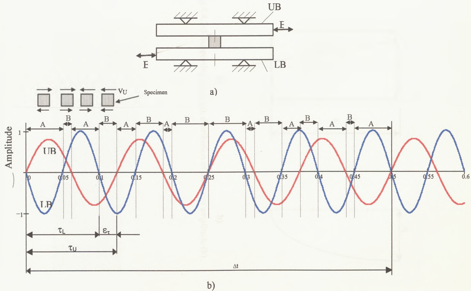
Fig.4.4.3-2 WT/P tool – scheme (a), relationship v_U(t) , v_L(t) and directions of these velocities relative to the specimen (b).
