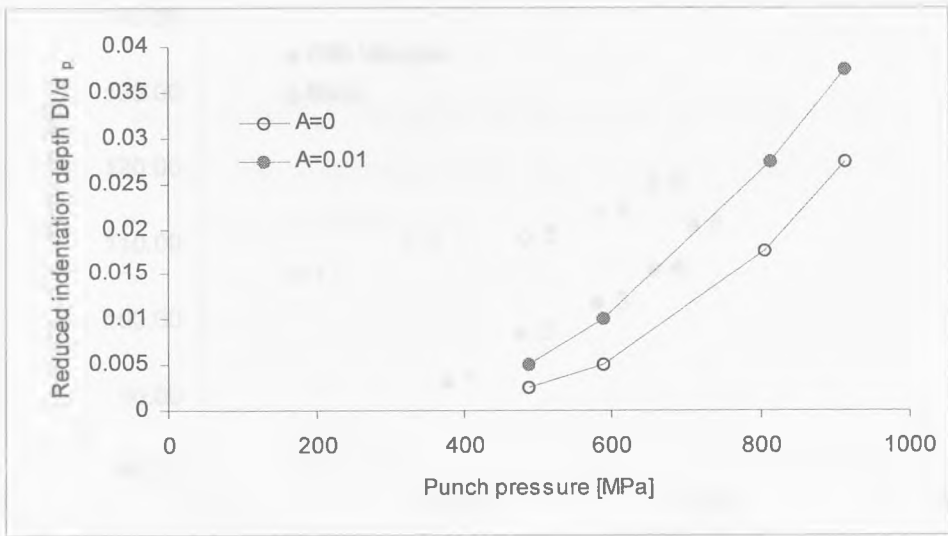
Fig.7.2.1-3 Indentation. Reduced indentation depth ( DI/d_p ) versus punch pressure for steel specimens.
