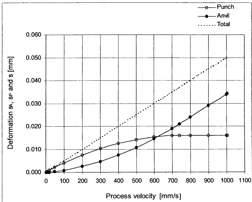
Fig.8.2.2-13 Total deformation ( s ) over one period of vibration and its components attributed to the punch ( s_P ) and anvil ( s_A ) movement. (Amplitude of vibration - 0.008mm.)
