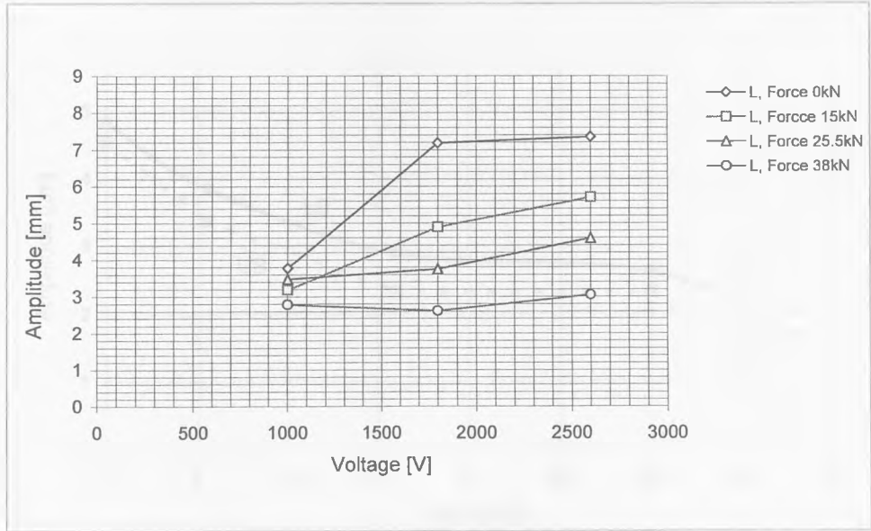
Fig.7.1-4 Amplitudes of vibration of the lower beam versus the excitation voltage for a mechanical load of 0, 15, 25.5 and 38kN.
