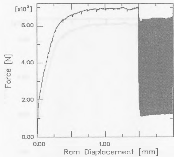
Fig.7.3.2-2 Force versus anvil displacement for back extrusion of Aluminium (anvil velocity 100mm/s, amplitude 0.0085mm).
