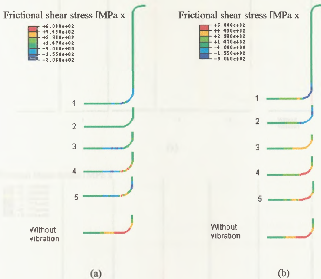
Fig.7.3.2-11 Frictional shear stress on the work-material surface in contact with the punch, with and without vibration imposed on the punch, for anvil velocity (a) 20mm/s and (b) 200mm/s. Profiles 1 to 5 corresponds to the the punch vibrational velocity shown in Fig.7.3.9a and Fig.7.3.10a.
