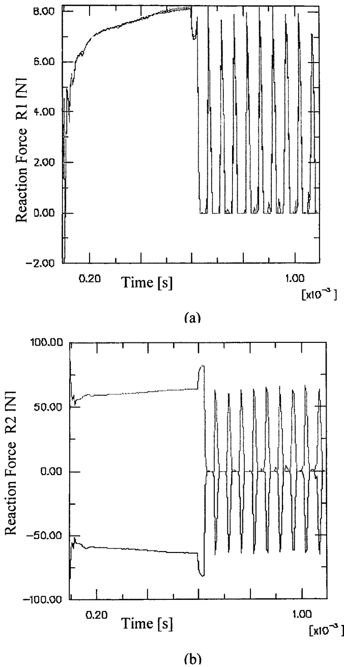
Fig.7.3.1-1 Reaction force on the forming tools (a) R1 in the drawing direction, (b) R2 in the direction perpendicular to drawing. Amplitude 0.01mm, drawing velocity 150mm/s.
