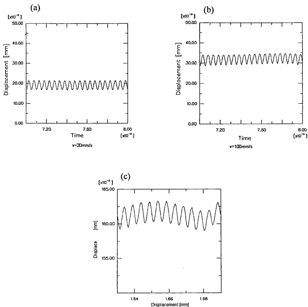
Fig.7.3.2-20 Displacement of the point C (tip of the punch), Aluminium specimens and ram velocity (a) 20mm/s, (b) 100mm/s, steel specimen and the ram velocity 100mm/s (c). Punch holder subjected to sinusoidal pressure of amplitude 10MPa at the surface marked by point A in Fig.7.3.2-14.
