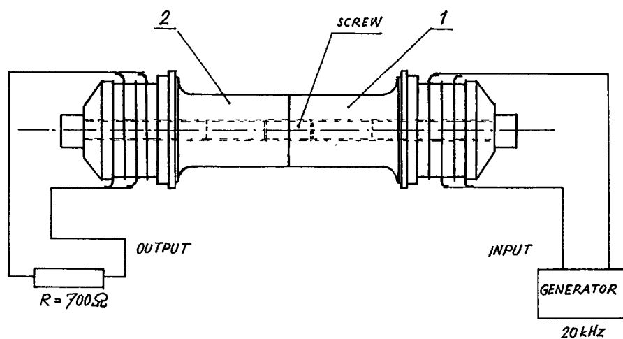
Fig.4.3-5 Scheme for measurement of efficiency of transducer ((1) and (2) transducers).
