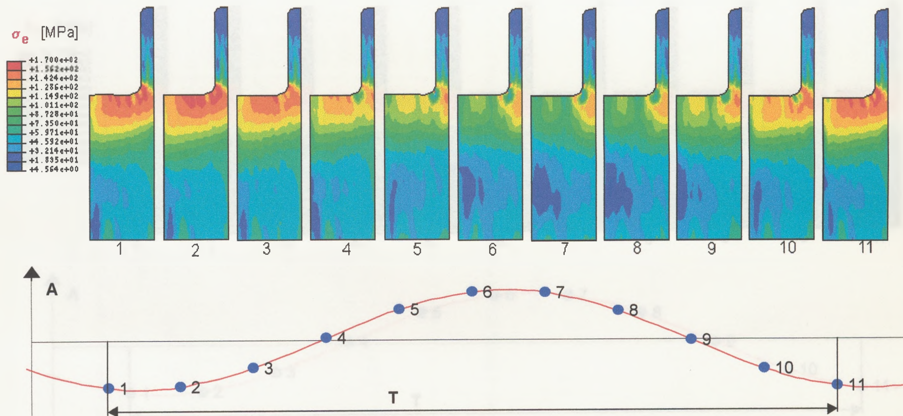
Fig.7.3.2.24 Back extrusion. Variation of the distribution of equivalent stress in the specimen over one cycle of vibration for a process velocity of 20mm/s and amplitude of vibration of 0.0085mm.
