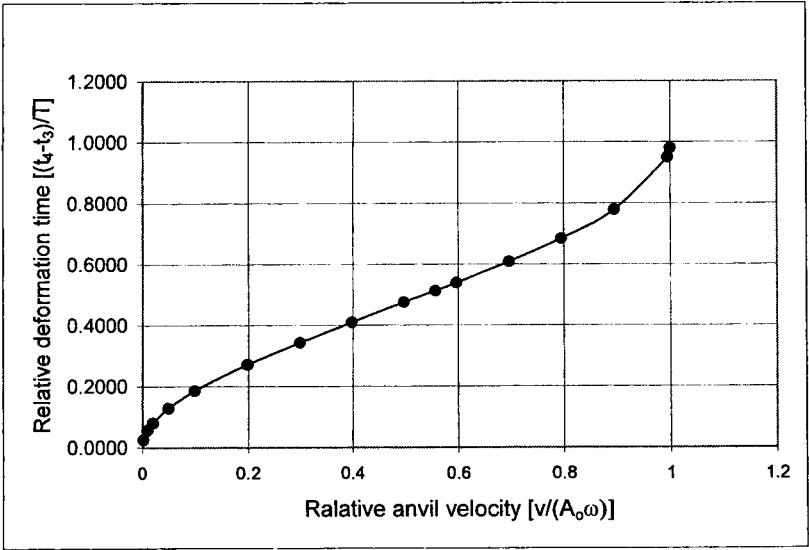
Fig.8.2.2-4 Variation of the relative time of deformation ((t_4 - t_3)/T) with relative anvil velocity (v_A/A\omega) .
