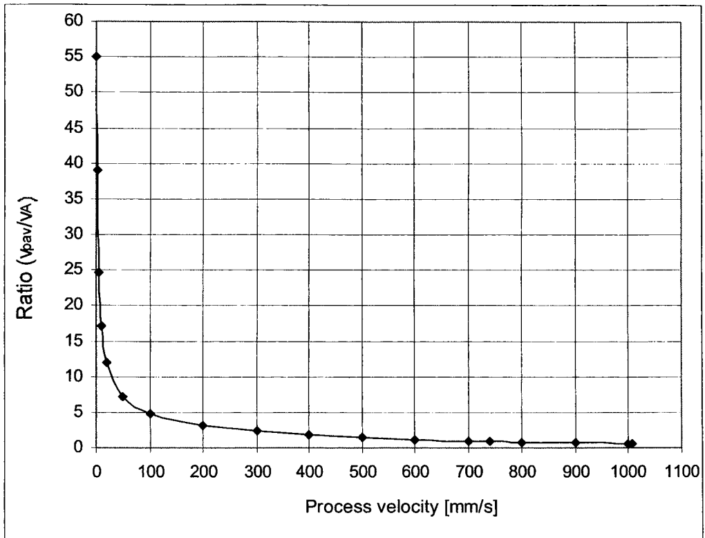
Fig.8.2.2-15 Variation of the ratio ( v_{pav}/v_A ) with the relative anvil velocity. (Amplitude of vibration – 0.008mm.)
