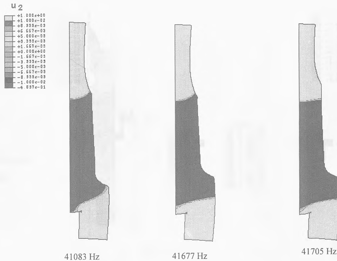
Fig.4.5.3-2 Influence of the shape of the element on the magnitude of the natural frequency and the location of the nodes (border between the ray and black sections).
