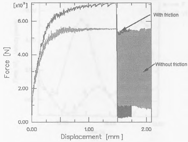
Fig.7.3.2-7 Force versus displacement when friction \mu=0.1 and frictionless conditions (amplitude 0.0085, anvil velocity 20mm/s).
