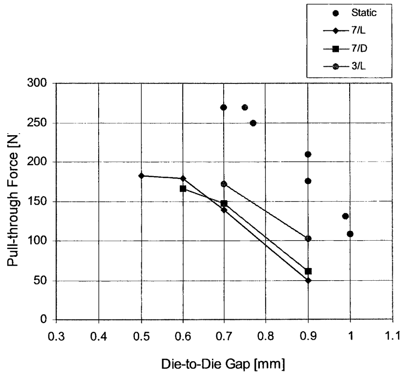
Fig.7.2.4-1 Pull-through force versus die-to-die gap for copper wire, \Phi = 1.2\text{mm} . L – under lubricated condition, D – under dry condition, amplitude of vibration - 3 or 7\mu\text{m} .
