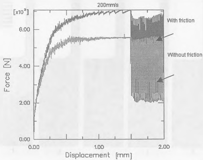
Fig.7.3.2-8 Force versus displacement when friction \mu=0.1 and frictionless conditions (amplitude 0.0085mm, anvil velocity 200mm/s).
