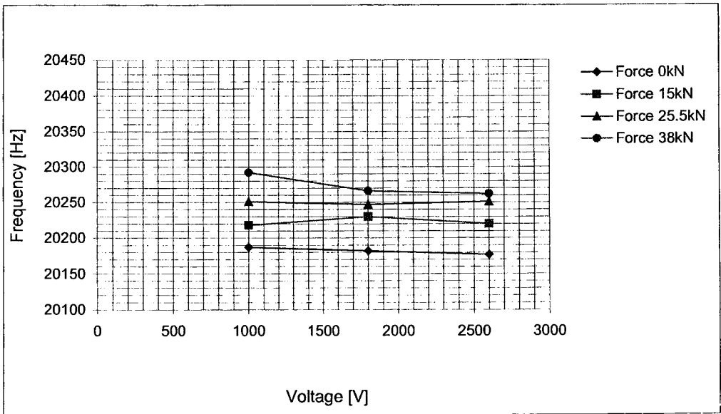
Fig.7.1-2 Frequencies of vibration of the upper beam versus the excitation voltage for a mechanical load of 0, 15, 25.5 and 38kN.
