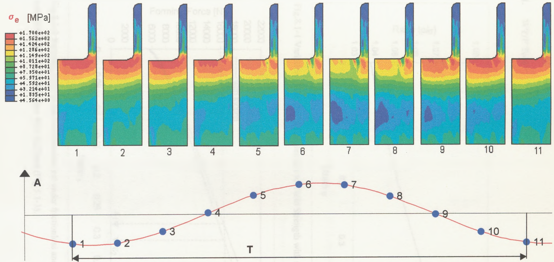
Fig.7.3.2.25 Back extrusion. Variation of the distribution of the equivalent stress in the specimen over one cycle of vibration for a process velocity of 100mm/s and amplitude of vibration of 0.0085mm.
