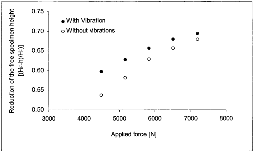
Fig.7.2.2-1 Heading. Variation of the specific head height with the applied force with and without vibration; aluminium specimens.
