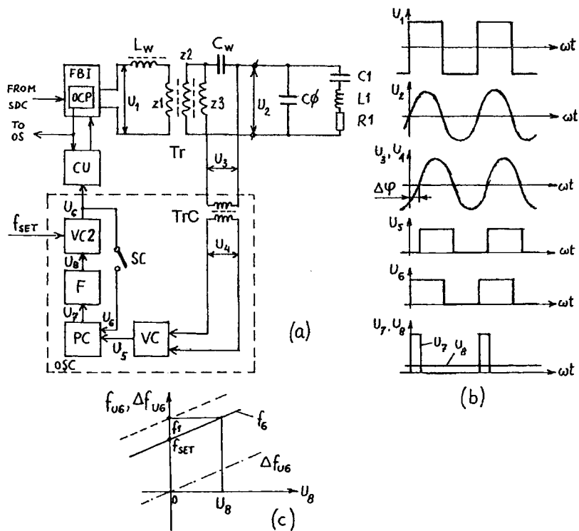
Fig.4.3-3 The feed-back control loop – Version II: a) block diagram, b) waveforms, c) Relationship between f_{U6} , \Delta f_{U6} and U_8 .
