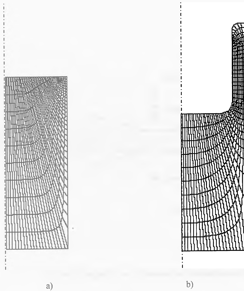
Fig.6-3 Can extrusion, specimen mesh undeformed (a) and deformed (b).
