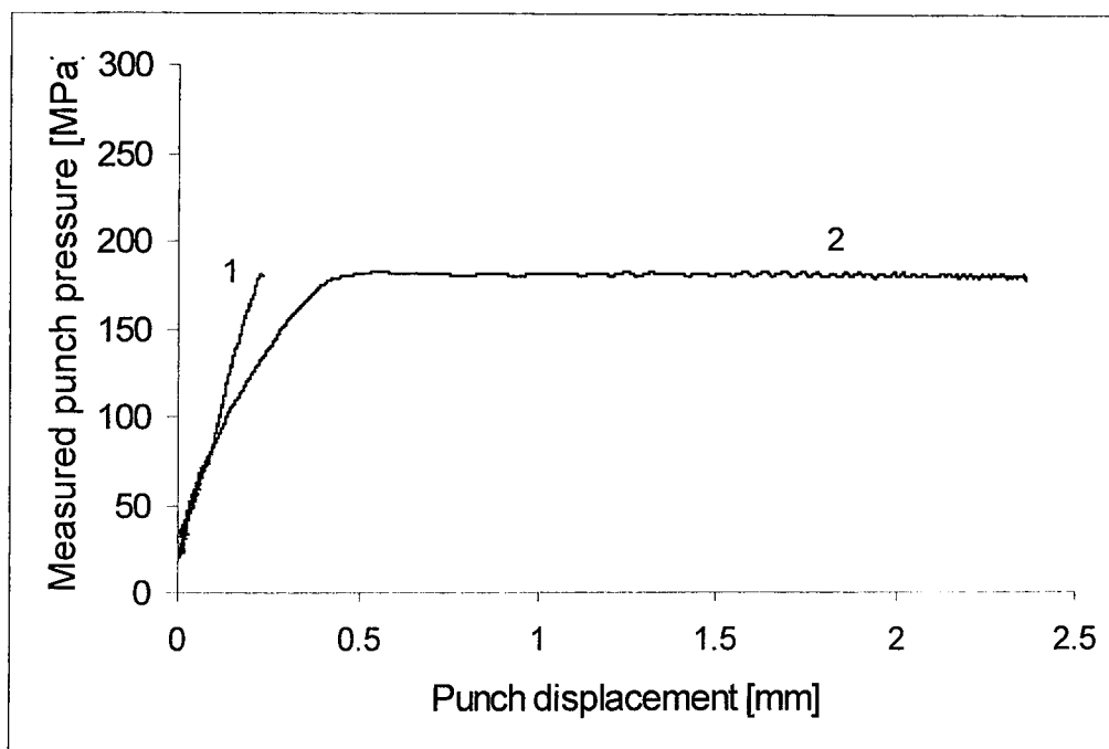
Fig.7.2.3-14 Influence of holding time of the load under superimposed ultrasonic vibrations on the final punch penetration. Punch penetration without vibrations (1) and superimposed vibrations (2), applied pressure – 180MPa, amplitude of vibration – 7,5 \mu\text{m} .
