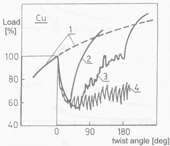
Fig.2.1.1-4 Tensile load versus angle of torsion in the tensile test with simultaneous torsion of cooper specimen: 1 – simple tensile test, 2 – with one direction continuos torsion by an angle of 45°, 3 – with one direction continuos torsion by an angle of 180°, 4 – cyclic twisting with an angle \pm 1^\circ .[35]
