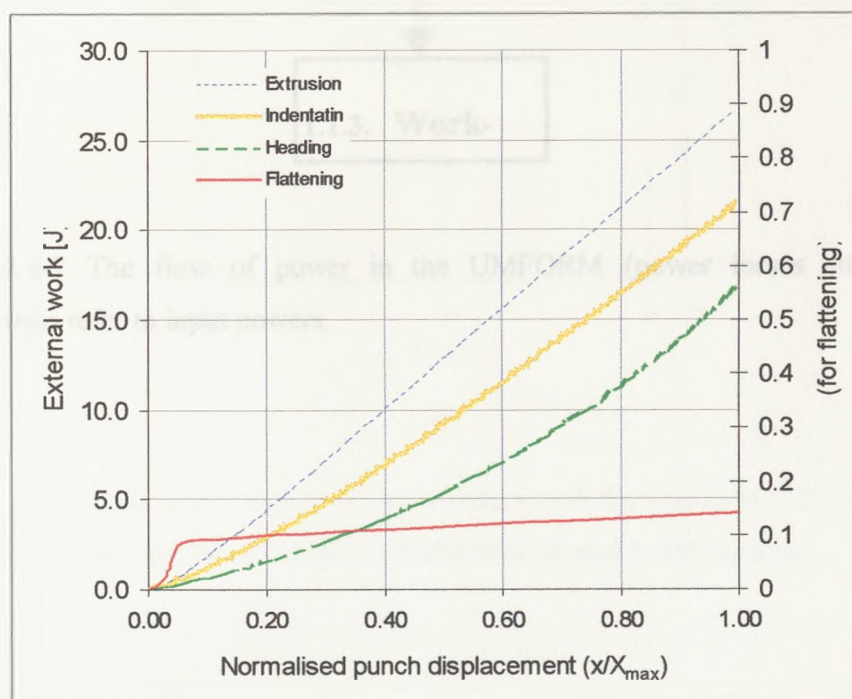
Fig.8.2.3-6 Variation of work done by external forces with normalised punch displacement for indentation, heading, can extrusion and wire flattening operations.
