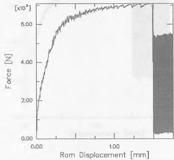
Fig.7.3.2-1 Force versus anvil displacement for back extrusion of Aluminium (anvil velocity 20mm/s, amplitude 0.0085mm).
