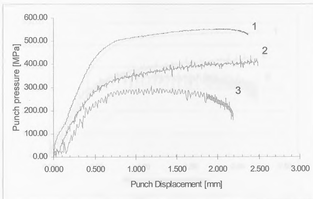
Fig.7.2.3-9 Back extrusion. Punch pressure versus punch displacement, deformation velocity v=5.0\text{mm/s} ; (1) without vibration, (2) amplitude of vibration A=3\mu\text{m} , (3) amplitude of vibration A=8.5\mu\text{m} .
