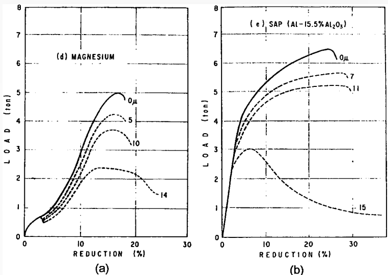
Fig.2.1.1-3 Relationship between compressive load and strain with superimposed ultrasonic vibrations of different amplitudes.[9]
