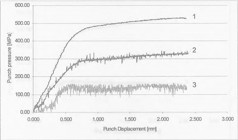
Fig.7.2.3-7 Back extrusion. Punch pressure versus punch displacement, deformation velocity v=0.5\text{mm/s} ; (1) without vibration, (2) amplitude of vibration A=4.5\mu\text{m} , (3) amplitude of vibration A=9.5\mu\text{m} .
