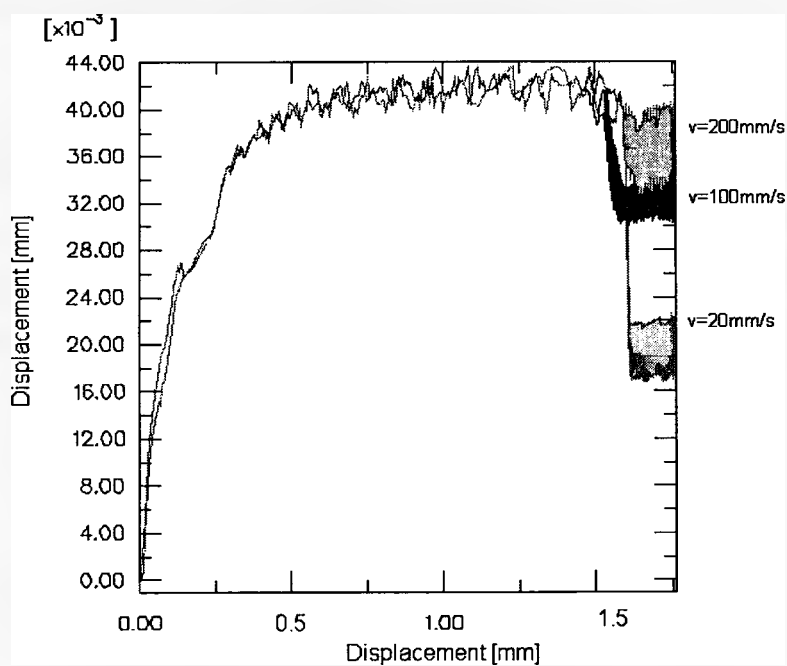
Fig.7.3.2-22 Displacement at the point C for the process velocity 20, 100 and 200mm/s. Amplitude of vibration of 0.0085 mm at the point A.
