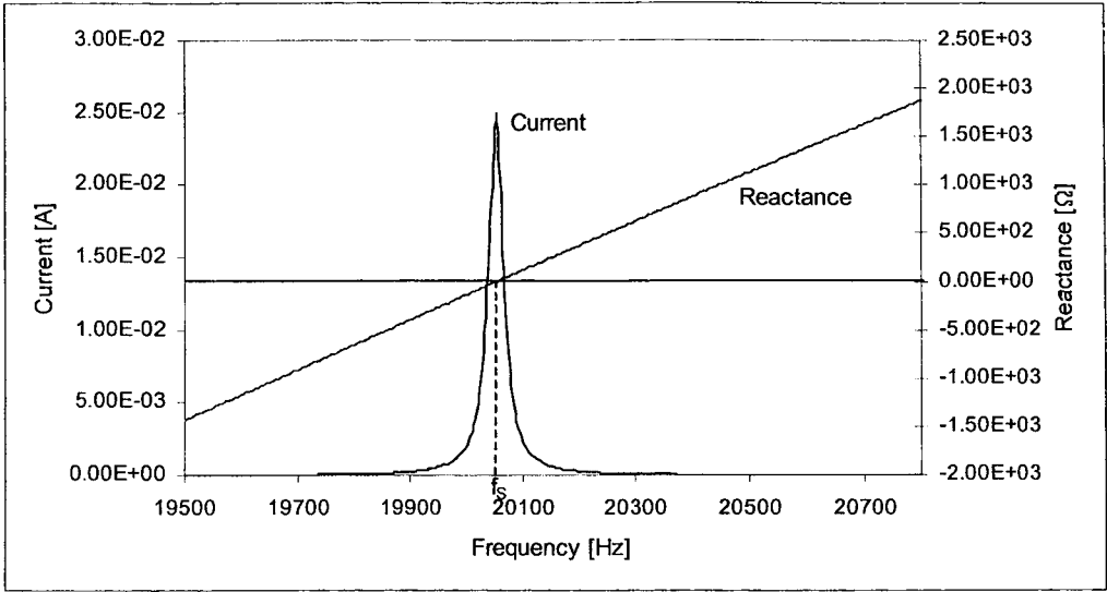
Fig.4.1.2-3 Variation of current and reactance with frequency in the mechanical branch of the equivalent circuit.
