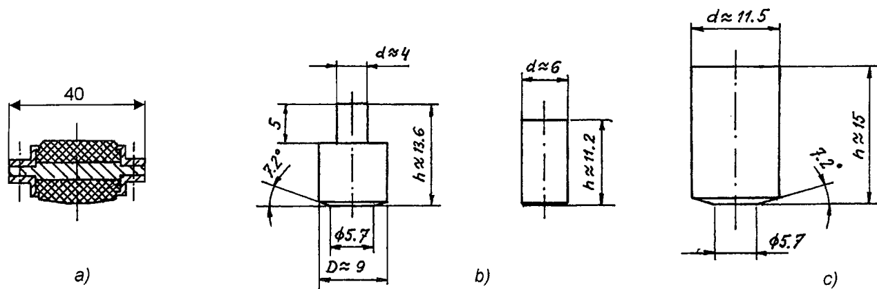
Fig.5.1-1 Specimens used in experiments with the WT/P tool – nylon (a), steel (b), aluminium (c).
