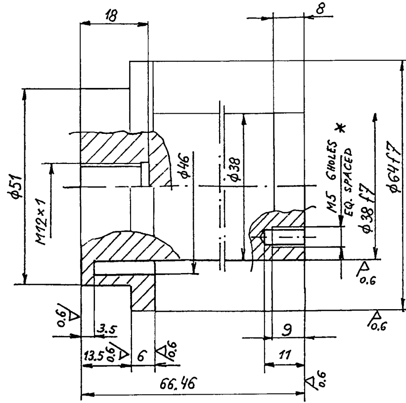
Fig.4.5.4-2 The anvil design
