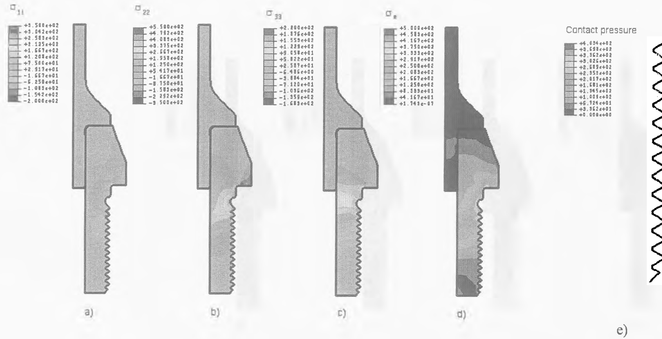
Fig.4.5.5-2 Stress in the induced by the tightening procedure; (a) axial stress, (b) radial stress, (c) circumferncial, (d) equivalent stress, (e) contact pressure in the thread.
