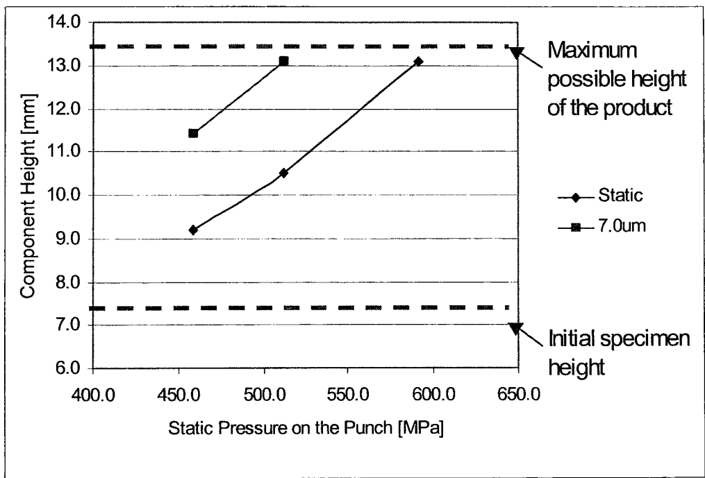
Fig.7.2.3-2 Back extrusion. Variation of the component height with the punch pressure with and without vibration. Punch diameter 4mm. Amplitude of vibration 7 \mu\text{m} . Specimen material: Al-2.
