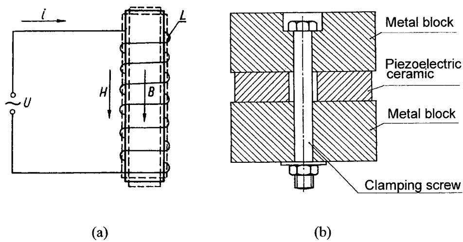
Fig.1-2 Transducers: (a) magnetostrictive, (b) piezoelectric.
