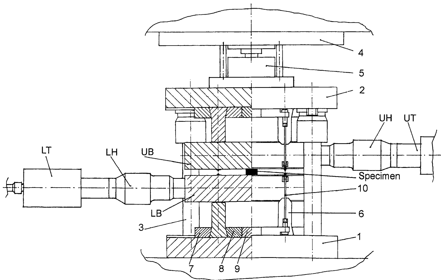
Fig.4.4.2-1 WT/P tool; UB, LB-upper and lower beams, UH, LH-booster, UT, LT-transducer.
