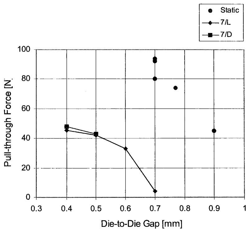
Fig.7.2.4-3 Pull-through force versus die-to-die gap for pure aluminium wire, \Phi=1\text{mm} . L – under lubricated condition, D – under dry condition, amplitude of vibration 0.007mm.
