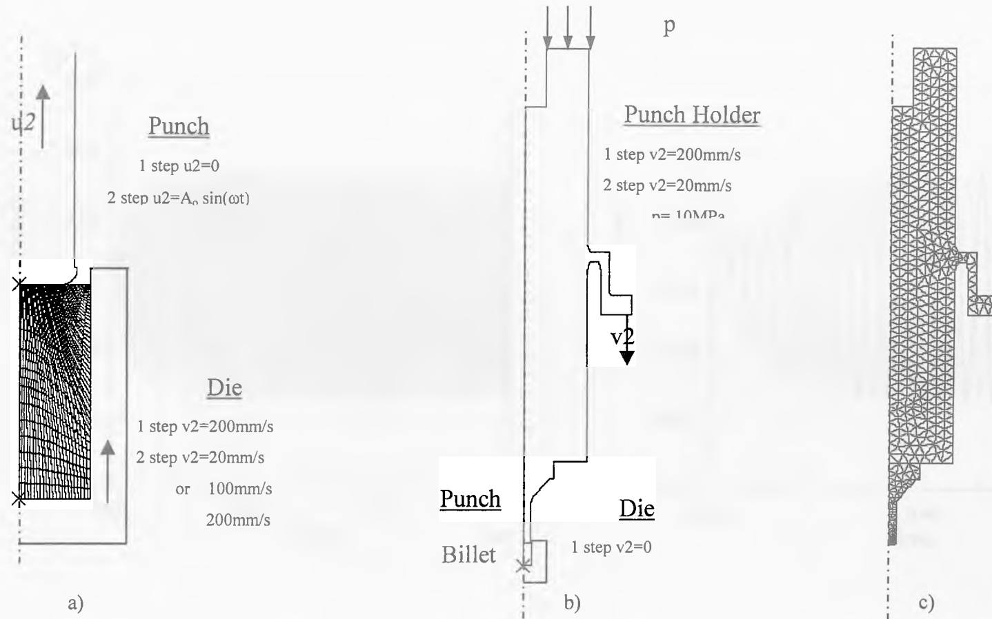
Fig.6-5 FE model for back extrusion with superimposed vibration, (a) with both tools rigid, (b) with the rigid die and deformable punch, (c) mesh of the punch holder and punch.
