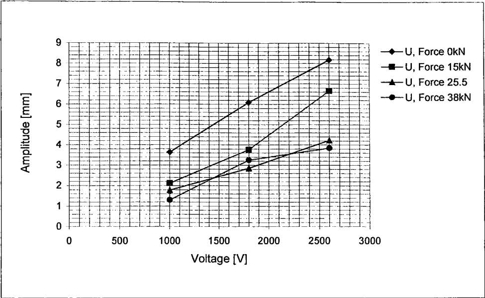
Fig.7.1-5 Amplitudes of vibration of the upper beam versus the excitation voltage for a mechanical load of 0, 15, 25.5 and 38kN.
