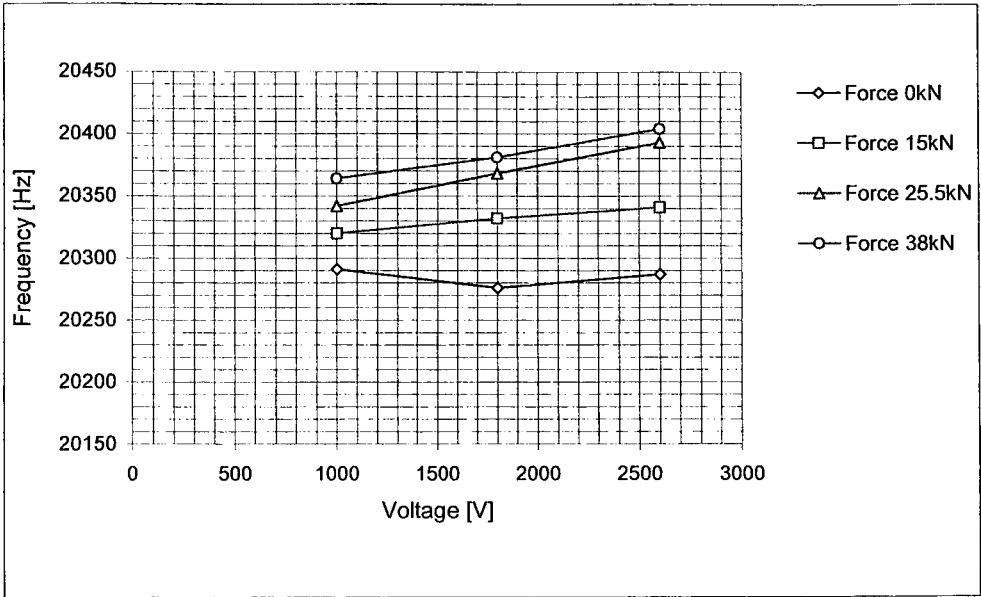
Fig.7.1-1 Frequencies of vibration of the lower beam versus the excitation voltage for a mechanical load of 0, 15, 25.5 and 38kN.
