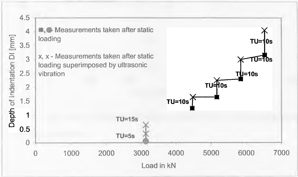
Fig.7.2.1-1 Indentation. Variation of the indentation depth with the applied force with and without vibrations. Amplitude of vibration 5 \mu m. Specimens – Aluminium, TU – time of applying vibration.
