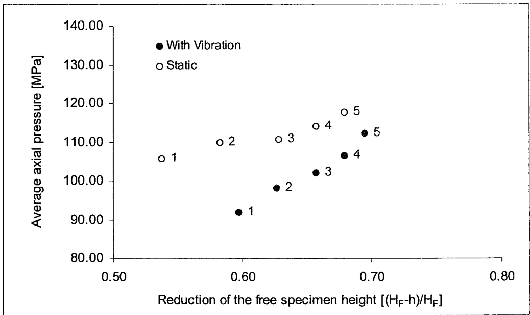
Fig.7.2.2-2 Heading. Average punch pressure versus reduction of the free specimen height.
