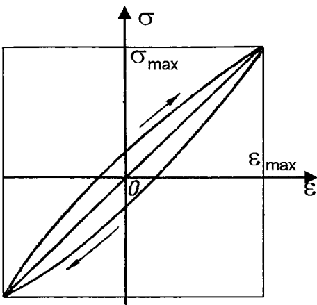
Fig.4.2-1 Mechanical hysteresis loop. The area of the loop represents the energy per a unit volume dissipated as heat.
