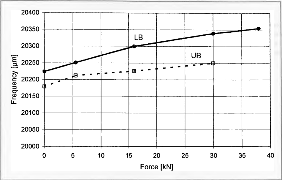
Fig.7.1- 3 Variation of the frequency of the beams with load for the excitation voltage 1800V. (LB – lower beam, UB – upper beam)
