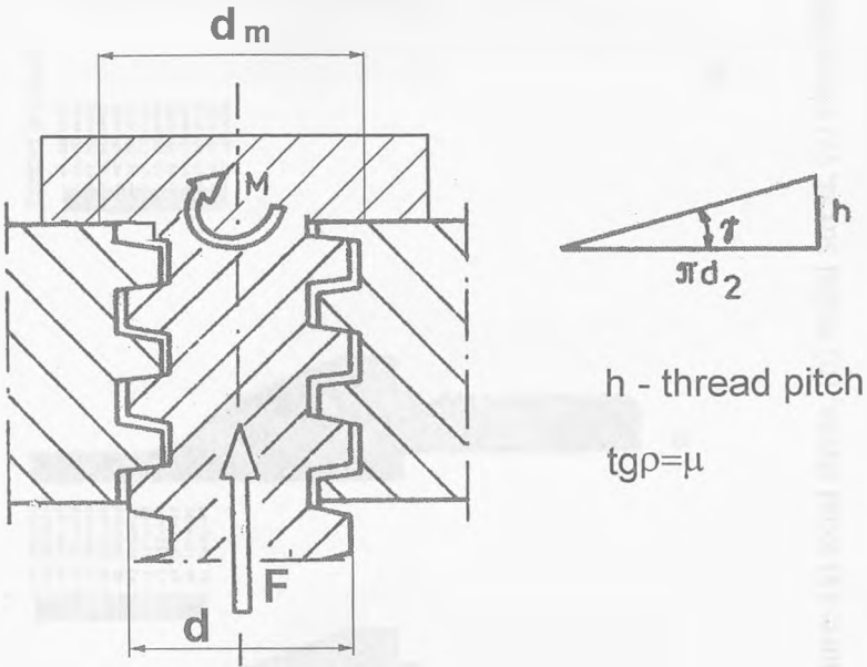
Fig.4.5.5-1 A screw.
