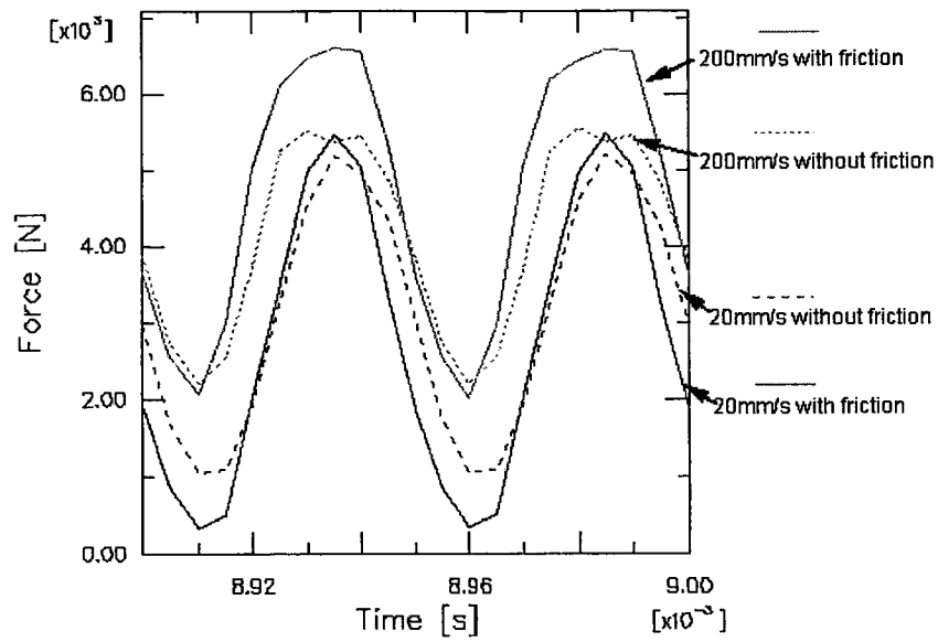
Fig.7.3.2-13 Variation of the force with time over two cycles of vibration for anvil velocities of 20 and 200mm/s when friction ( \mu=0.1 ) and frictionless conditions.
