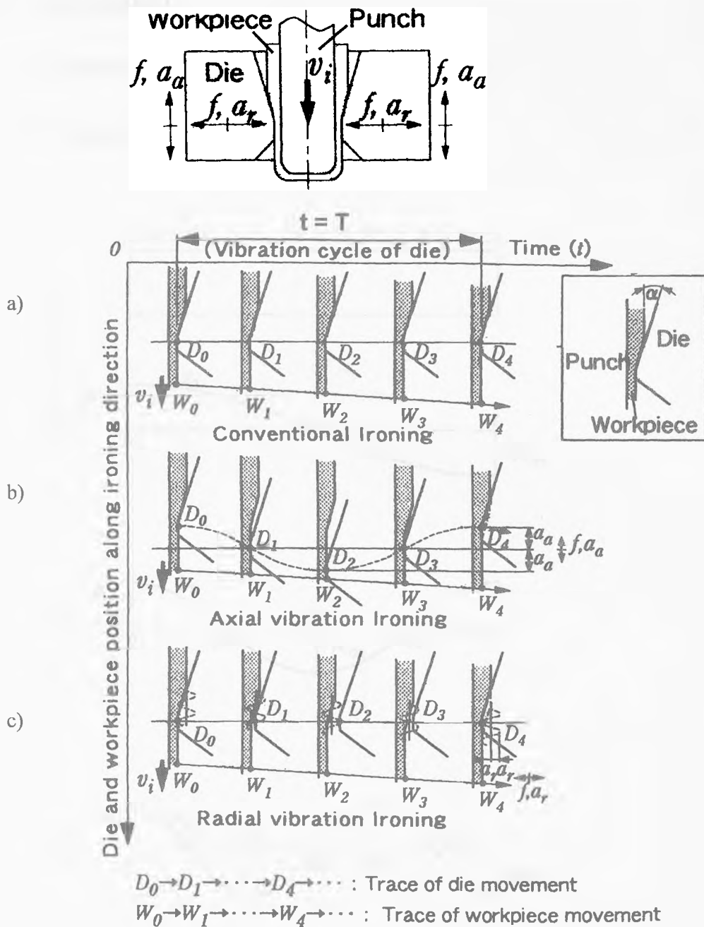
Fig.2.2.1-2 Ironing process using (a) conventional method, (b) die vibrating longitudinally and (c) die vibrating radially. Symbols; f , a_a and a_r denote frequency, amplitude of longitudinal vibration, amplitude of radial vibration respectively. [18]
