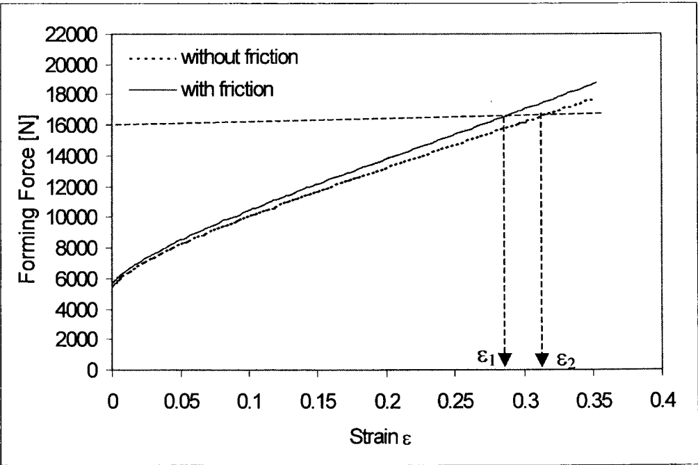
Fig.8.1-2 Forming force in the compression test under frictionless and friction conditions \mu=0.1 (Aluminium \Phi 11.5 \times 15 \text{ mm} (Fig.5.1-3)).
