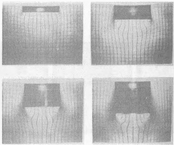
Fig.4.5.1-4 Material flow in indentation for different reduced indentation depth ( h/d_p )=0.2, 0.4, 0.6 and 0.8 (work-material H10). [101]
