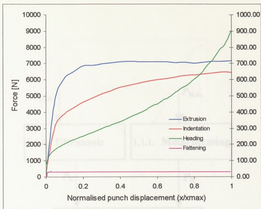
Fig.8.2.3-5 Forming force for indentation, heading, can extrusion and wire flattening (right scale refers to wire flattening).
