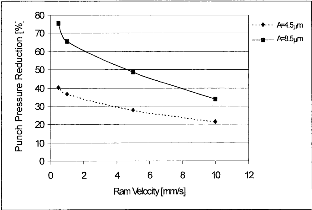
Fig.7.2.3-13 Reduction in punch pressure with ram velocity for amplitude of vibration 4.5 and 8.5μm.
