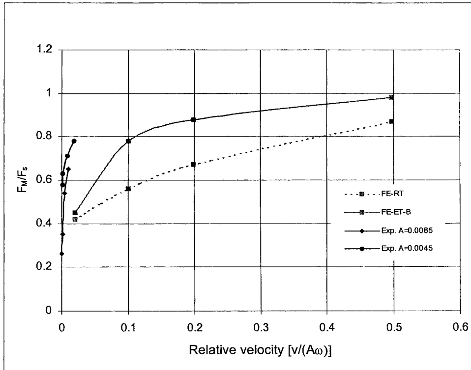
Fig.7.3.2-23 Ratio of the average forming force F_M to the forming force F_S under static conditions versus relative velocity. Finite element results FE-RT (model with rigid tools), FE-ET (model with elastic tool), and experimental results Exp.A=0.0085 and Exp.A=0.0045.
