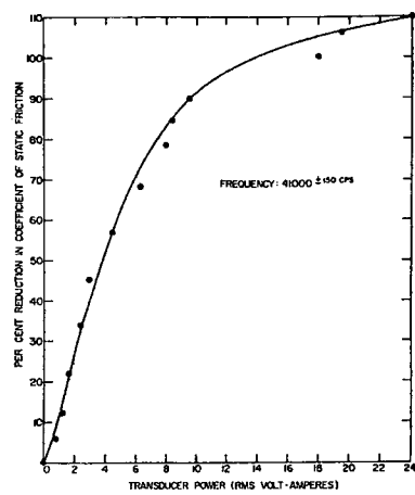
Fig.2.1.2-1 Coefficient of static friction versus transducer power for highly polished steel surface. [12]
