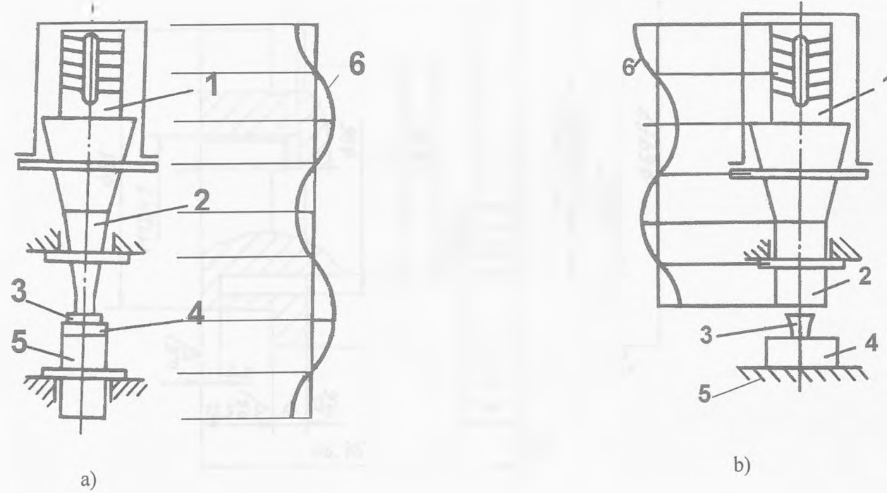
Fig.4.5.4-1 Closed (a) and open vibrating system. 1 – transducer, 2- booster-tool, 3 –workpiece, 4- die, 5 – anvil, 6 – amplitude distribution along the system
