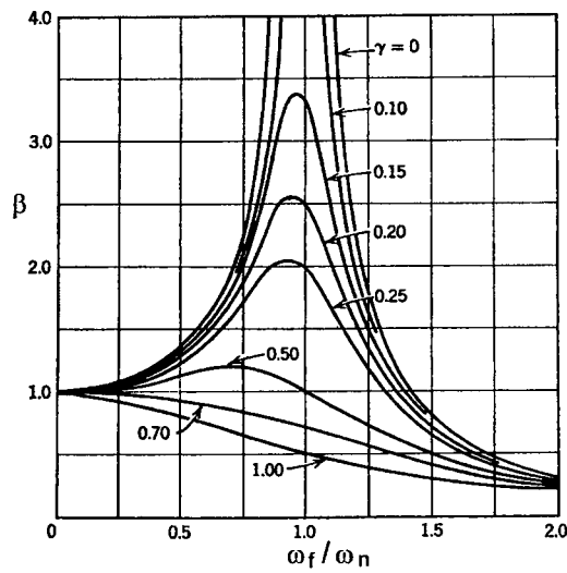
Fig.8.2.2-2 Variation of the amplitude of forced vibrations with the ratio \omega_f/\omega_n for different damping coefficient [2].
