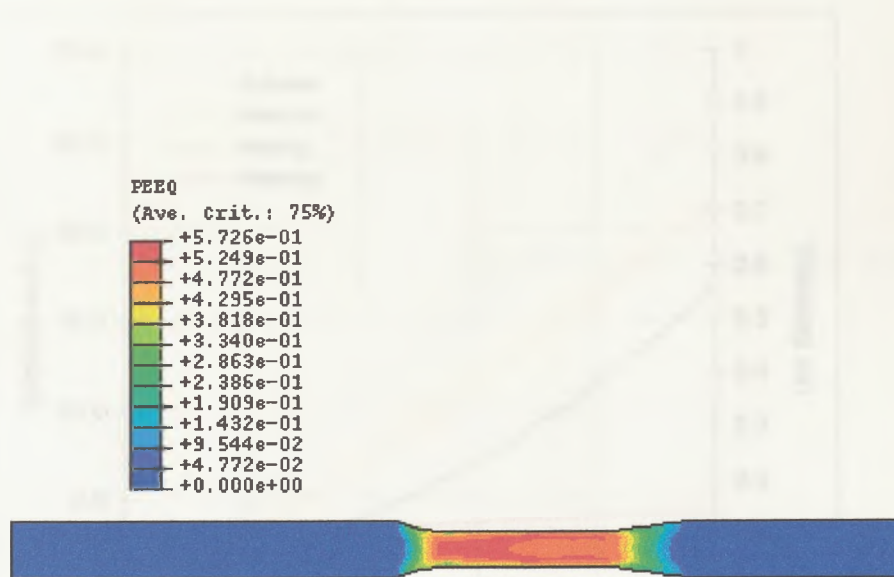
Fig.8.2.3-3 Can extrusion – equivalent strain distribution.
