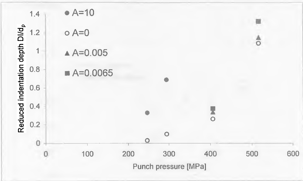
Fig.7.2.1-2 Indentation. Reduced indentation depth ( DI/d_p ) versus punch pressure for aluminium specimens.
