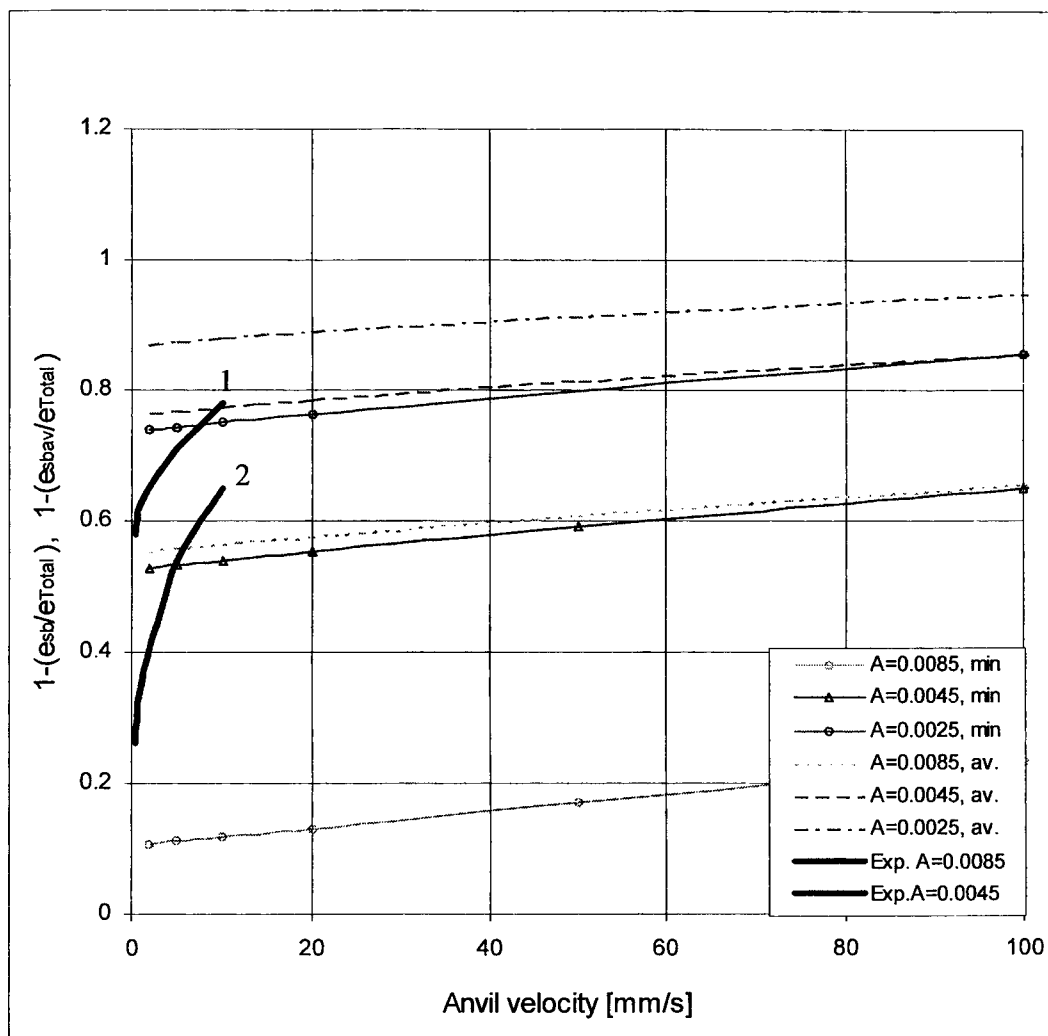
Fig.8.2.2-10 Variation of the ratio of the forces measured in processes with and without vibration for amplitudes of vibration 0.0045 mm (curve 1) and 0.0085mm (curve 2) and the punch velocity ranging from 0.5mm/s to 10mm/s. Plotted against theoretical curves from Fig.8.2.3-9.
