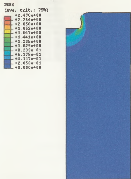
Fig.8.2.3-1 Indentation – equivalent strain distribution.
